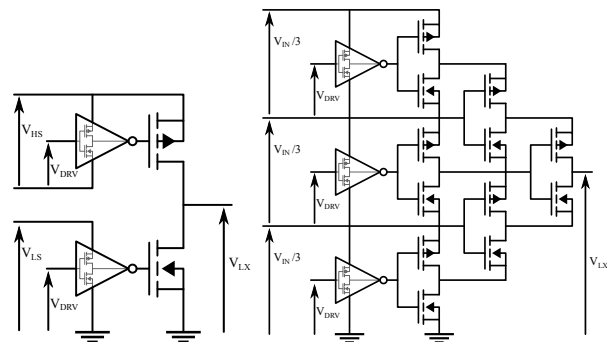
Fig. 16 Standard (left) and cascode (right) power stage.
