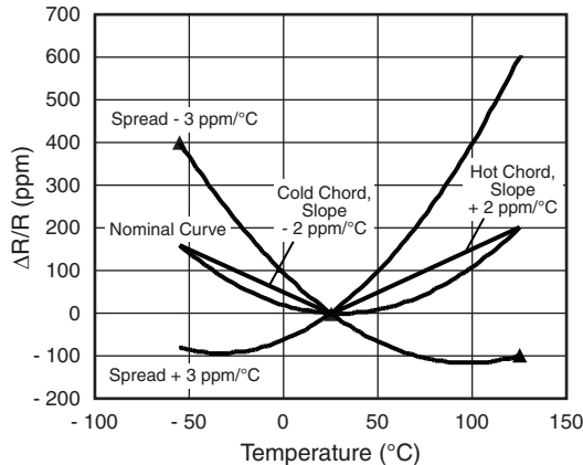
Fig. 1 - ( \Delta R/R = f(T) ) Chart of Resistors of \pm 5 ppm/ ^{\circ}\text{C} TCR
