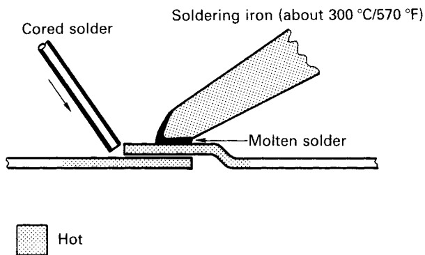
Figure 3.1 The principle of handsoldering
