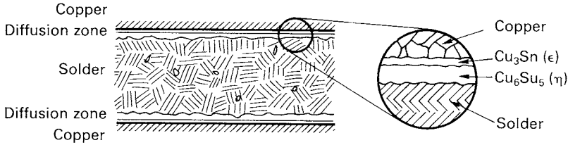
Figure 3.7 Cross-section through a soldered joint, made with eutectic solder
