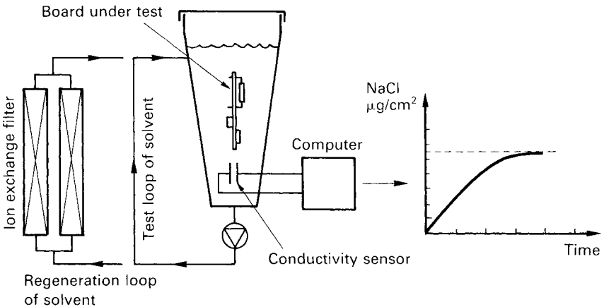
Figure 8.19 Working principle of a MIL contamination meter
