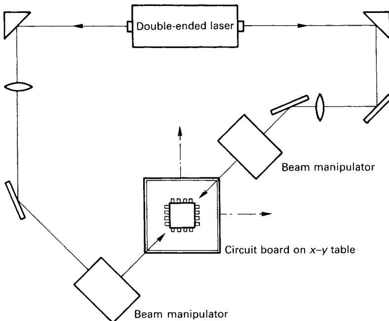
Figure 5.25 A twin-beam Nd: YAG lasersoldering machine (Baasel, Germany)
