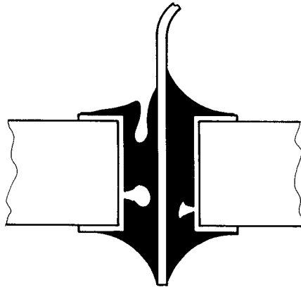
Figure 9.6 Blowholes in a throughplated wavesoldered joint
