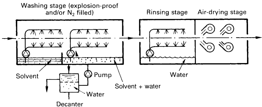
Figure 8.16 In-line semi-aqueous cleaning (water-immiscible solvent)
