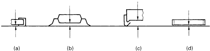
Figure 8.5 Stand-off heights of various SMDs. (a) Chip resistors and ceramic condensers 25\ \mu\text{m}/1\ \text{mil} ; TA condensers 100\ \mu\text{m}/4\ \text{mil} ; (b) SOTs 125\ \mu\text{m}/5\ \text{mil} ; SOICs, QFPs < 250\ \mu\text{m}/10\ \text{mil} ; (c) PLCCs 250\ \mu\text{m}/10\ \text{mil} ; (d) LCCCs and BGAs < 25\ \mu\text{m}/1\ \text{mil}
