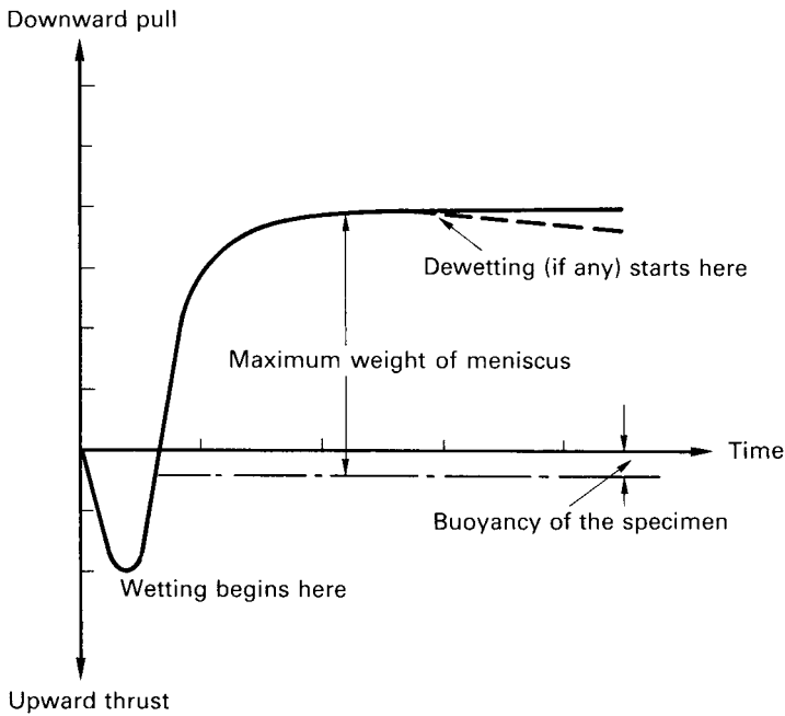
Figure 3.24 The wetting curve
