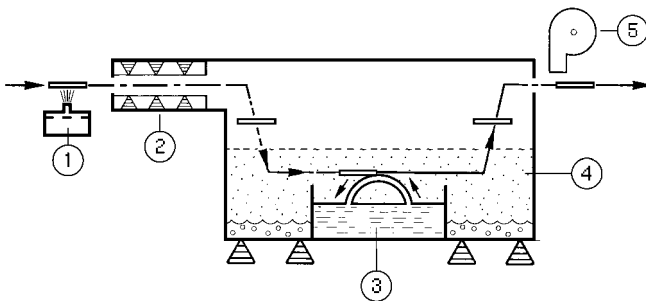
Figure 4.26 Wave soldering in a vapourphase atmosphere: 1, spray fluxer; 2, preheating; 3, solder wave; 4, working vapour; 5, cooling stage
