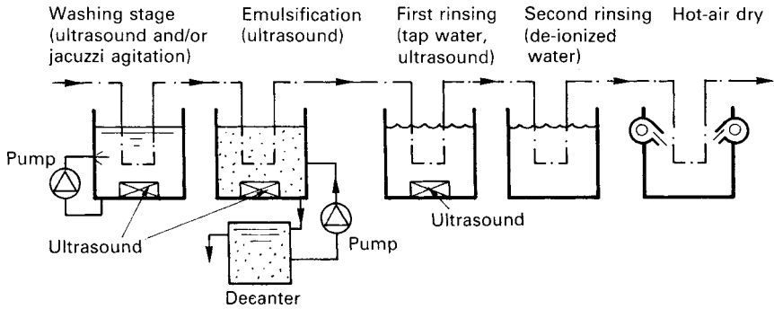
Figure 8.17 Batch-type semi-aqueous cleaning (water-immiscible solvent)
