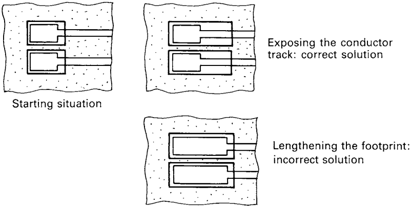
Figure 6.7 Letting the conductor track lead the solder to the joint
