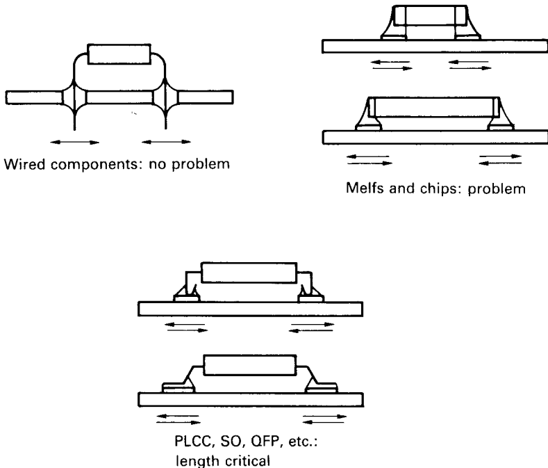
Figure 6.1 Thermal expansion: the behaviour of SMDs and wired components
