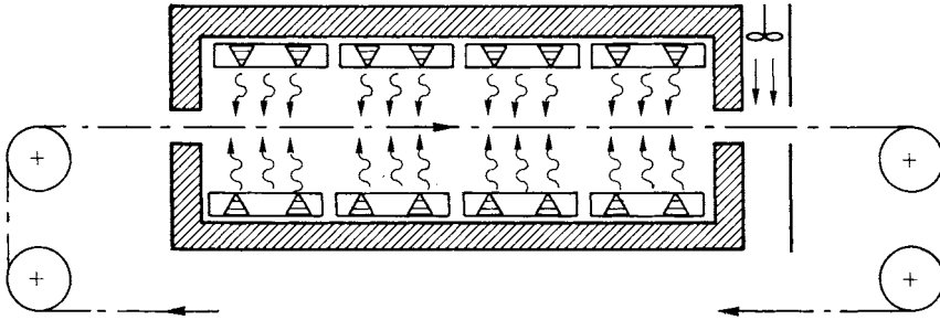
Figure 5.13 Working principle of an infrared soldering oven. \triangle Heaters
