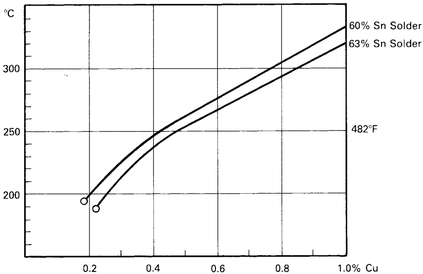
Figure 3.6 Solubility of copper in non-antimonial solder (author's measurements)
