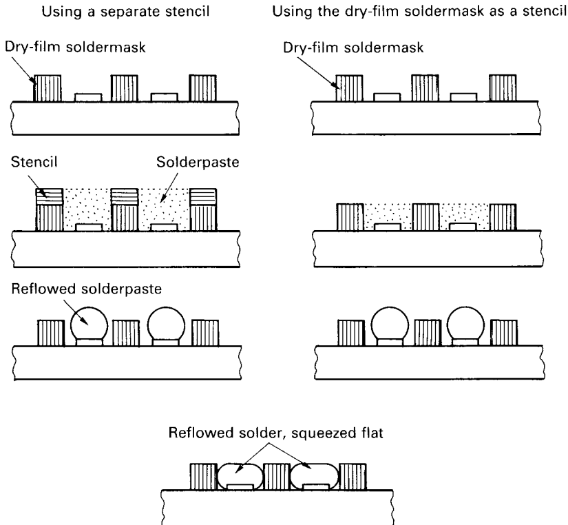
Figure 6.6 Two options for creating flat solder depots (the Sipad ® process)
