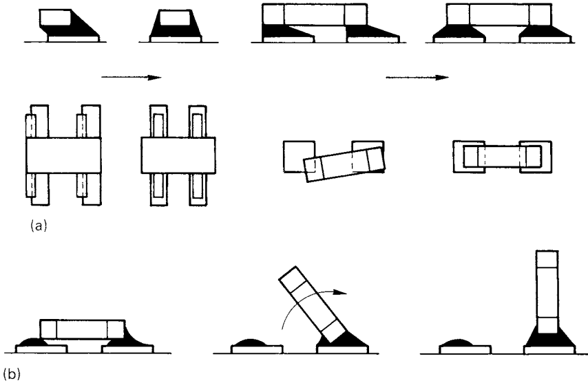
Figure 3.18 The effects of capillarity in reflowsoldering. (a) Self-alignment of components; (b) tombstoning
