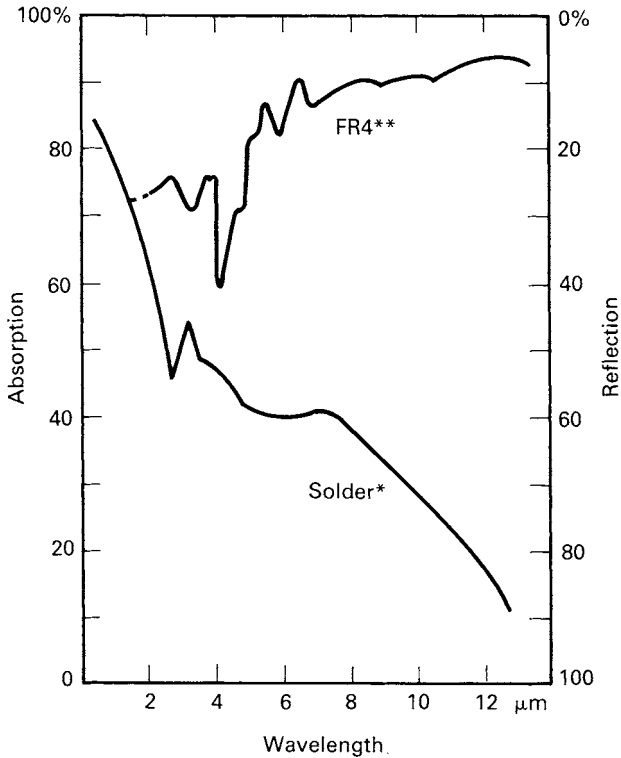
Figure 5.15 Reflection and absorption behaviour of solder and FR4 in the IR range. * After Lusk, E. F. (1984) Electronic Packaging Prod. , 24 , 3, pp. 98–104. ** After Dow, S. J. (1985) Brazing and Soldering , No. 8, pp. 16–19
