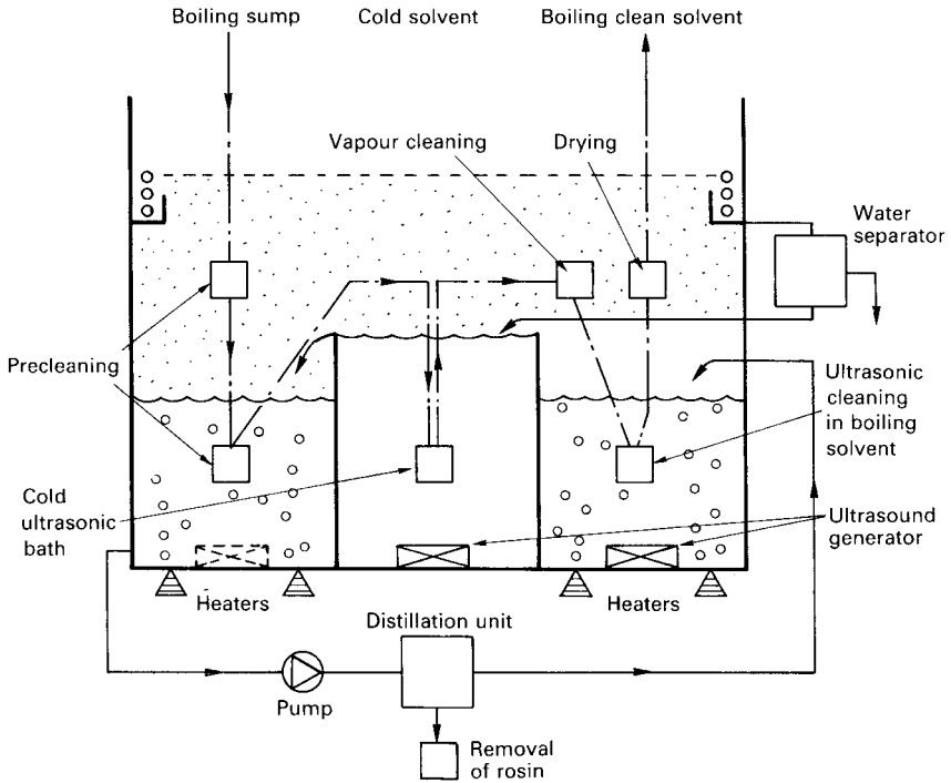
Figure 8.11 Three-tank solvent cleaning unit
