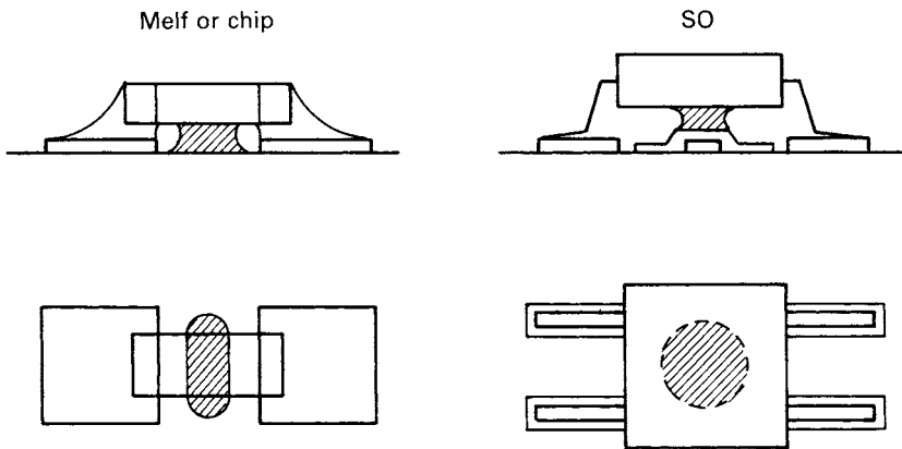
Figure 8.4 Effect of the adhesive joint on the accessibility of the flux residue
