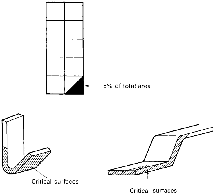
Figure 3.27 Judging a dipping test result
