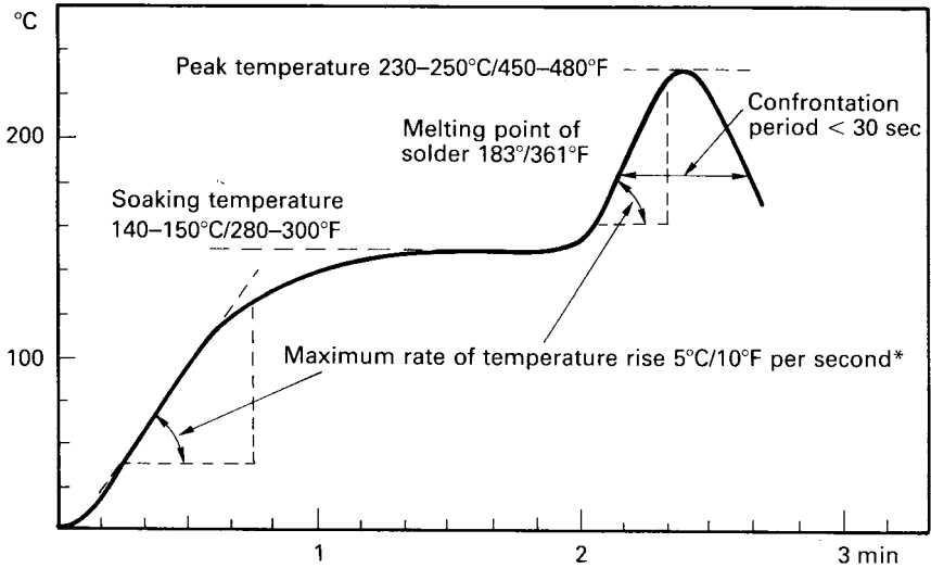
Figure 5.19 Realistic temperature profile of an infrared reflowsoldering operation. *After Reithinger, M. (1991) Reflow Soldering Technology for Surface Mount Assembly, Electr. Productn. , March 1991, pp. 27–37
