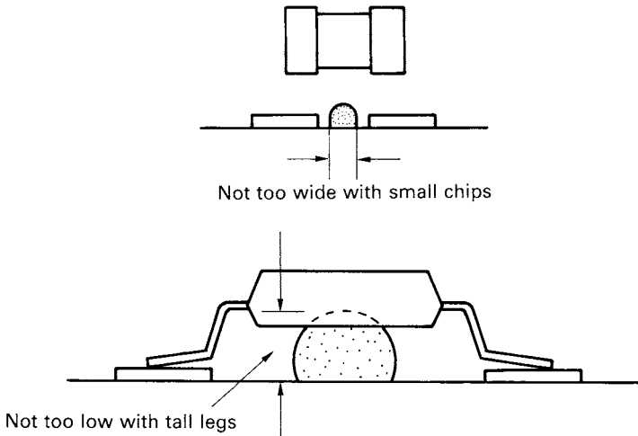
Figure 4.33 Demands on the adhesive spot
