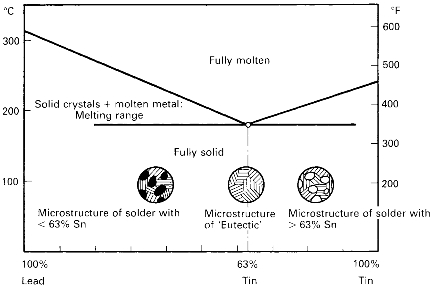
Figure 3.4 Melting-point diagram and microstructure of the tin–lead alloys
