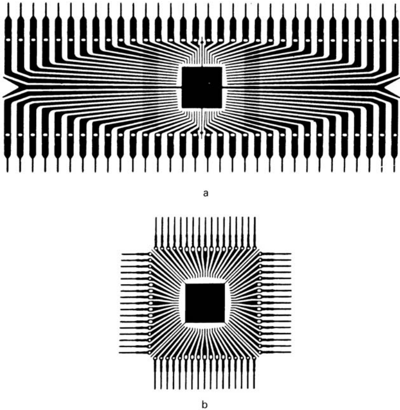
Figure 1.2 DIL and PLCC. (a) 64-lead DIL, 2.54 mm/100 mil pitch; (b) 68-lead PLCC, 1.27 mm/50 mil pitch (Philips)
