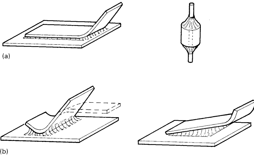
Figure 3.19 (a) Capillary joints and (b) open joints
