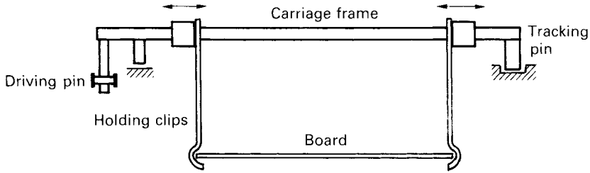
Figure 4.27 Board carriage
