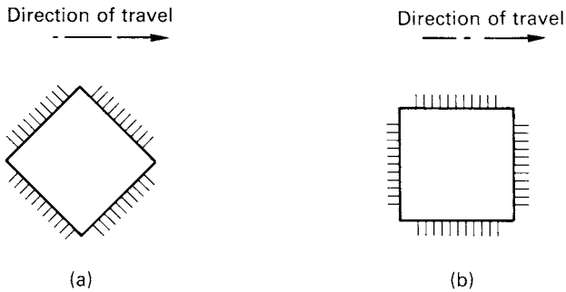
Figure 6.8 Mitigating the shadow effect. (a) Favourable alignment; (b) unfavourable alignment
