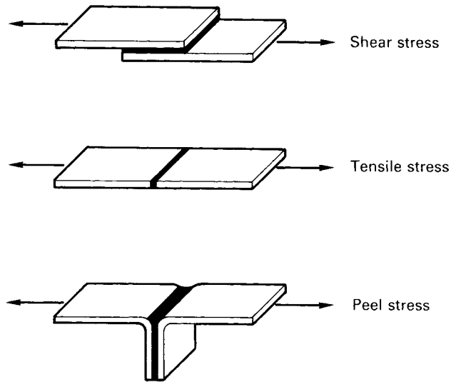
Figure 3.8 The mechanical behaviour of soldered joints under stress
