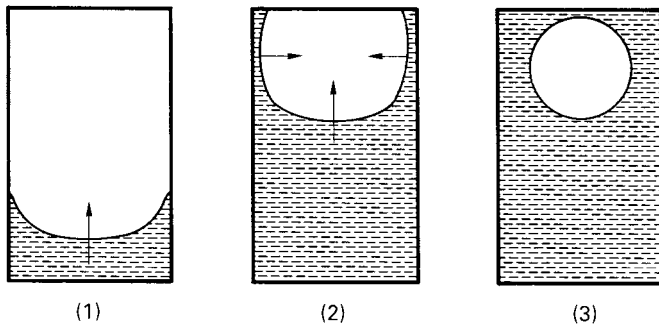
Figure 3.20 How molten solder fills a capillary joint
