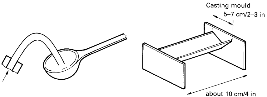
Figure 4.32 Taking a solder sample
