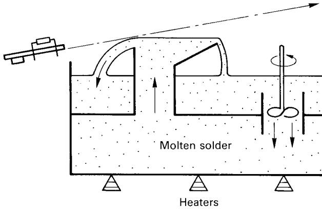
Figure 4.10 Working principle of a wavesoldering machine
