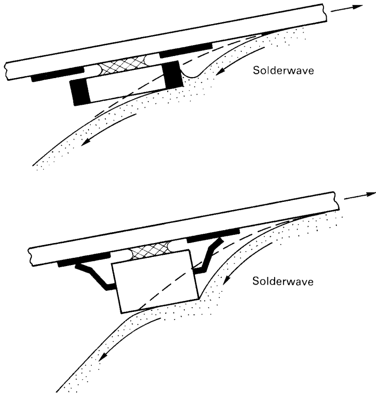
Figure 4.11 The shadow effect
