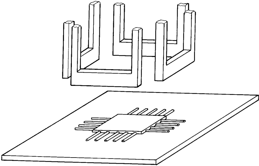
Figure 5.31 Four-bar thermode
