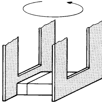
Figure 10.3 Desoldering with heated tweezers
