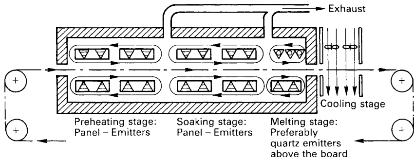
Figure 5.20 Principal features of an IR reflowsoldering oven
