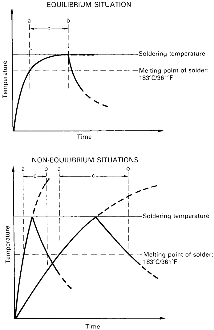
Figure 3.14 Equilibrium and non-equilibrium heating situations
