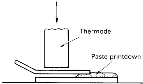
Figure 5.27 Paste printdown for thermode soldering
