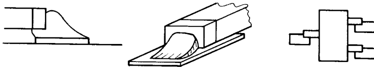
Figure 9.4 Some soldering imperfections
