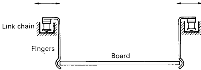
Figure 4.28 Finger conveyor
