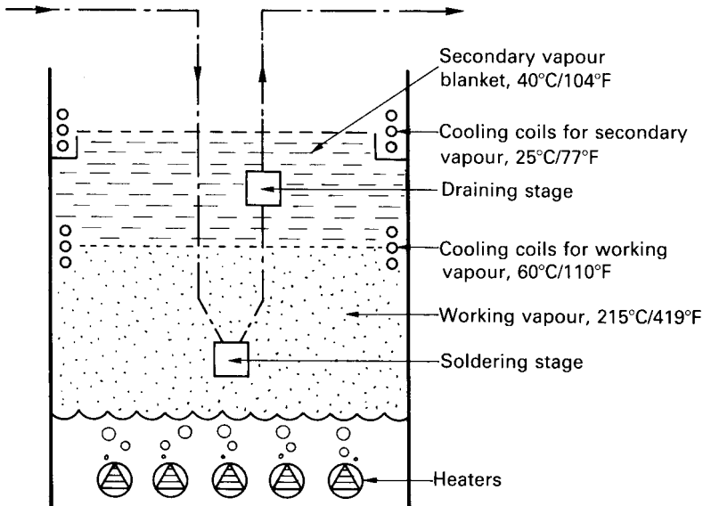
Figure 5.9 Vapour phase batch soldering principle
