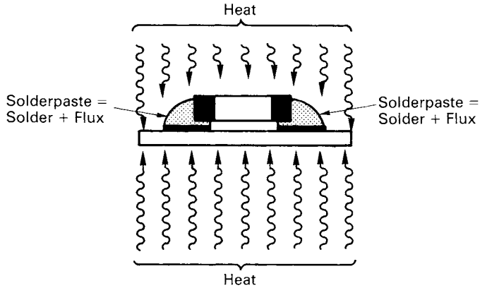
Figure 3.3 The reflowsoldering principle
