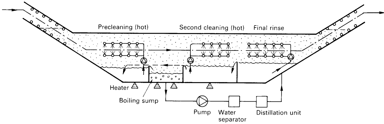
Figure 8.13 An in-line pure jet cleaning plant (OSL)
