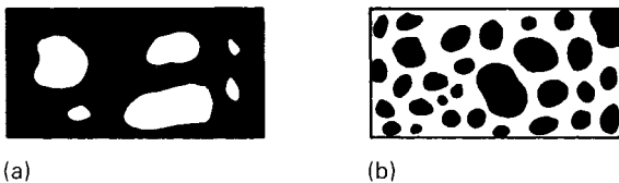
Figure 9.8 X-ray images of capillary joints. (a) Innocuous cavities caused by trapped air or vapour; (b) pattern of unsoundness indicating a wetting or solderability problem. ■ Solder, □ void
