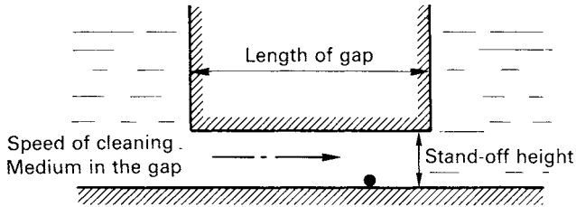
Figure 8.8 The hydrodynamics of cleaning
