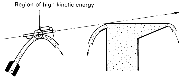
Figure 4.19 Unidirectional jetwave as primary wave
