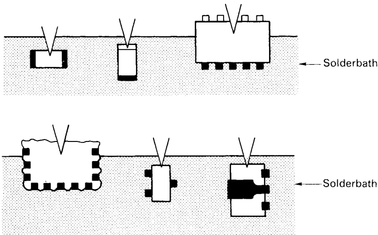
Figure 3.26 The dipping test for SMDs
