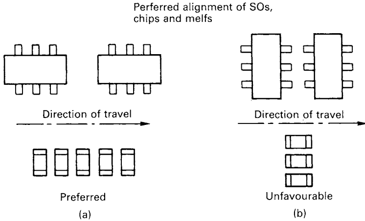
Figure 6.9 Preferred alignment relative to direction of travel. (a) Favourable alignment; (b) alignment resulting in the formation of bridges
