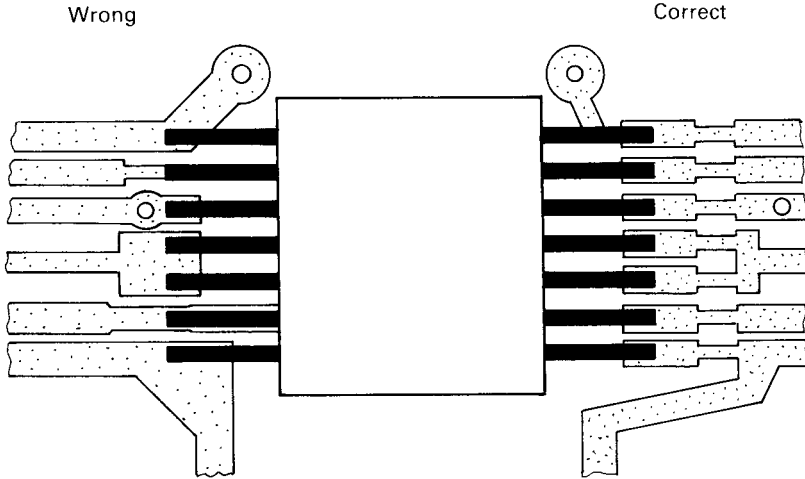
Figure 5.30 Footprint layout for impulse soldering. After Soldering in SMD Technology, Siemens, Munich, Germany
