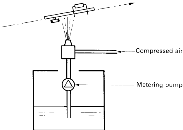
Figure 4.4 Working principle of a compressed-air sprayfluxer
