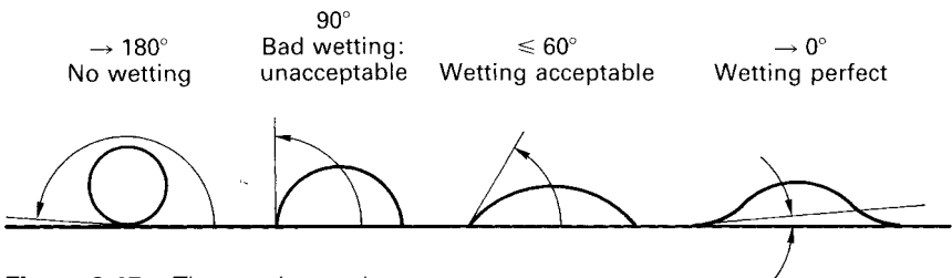
Figure 3.15 The wetting angle
