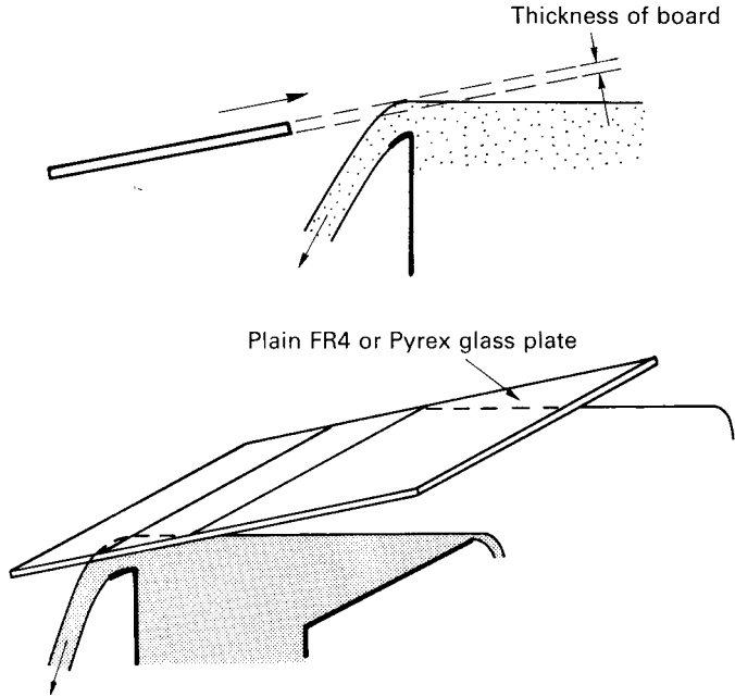
Figure 4.31 Checking depth of immersion and horizontal alignment between wavecrest and board
