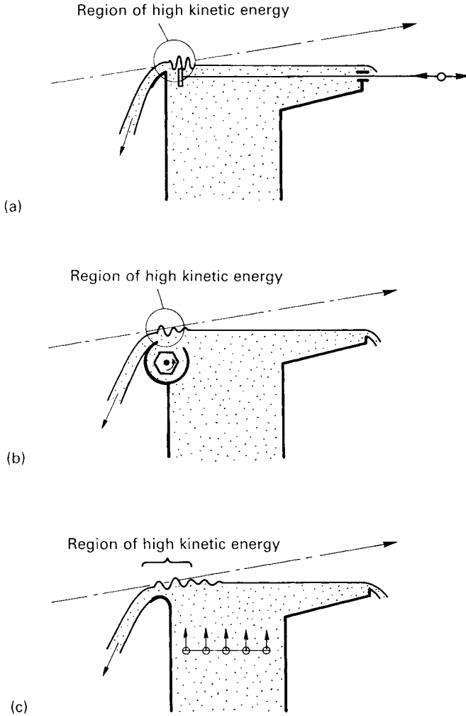
Figure 4.22 Three examples of combination waves. (a) Omega Wave ®; (b) Smart Wave ®; (c) CMS Wave ®
