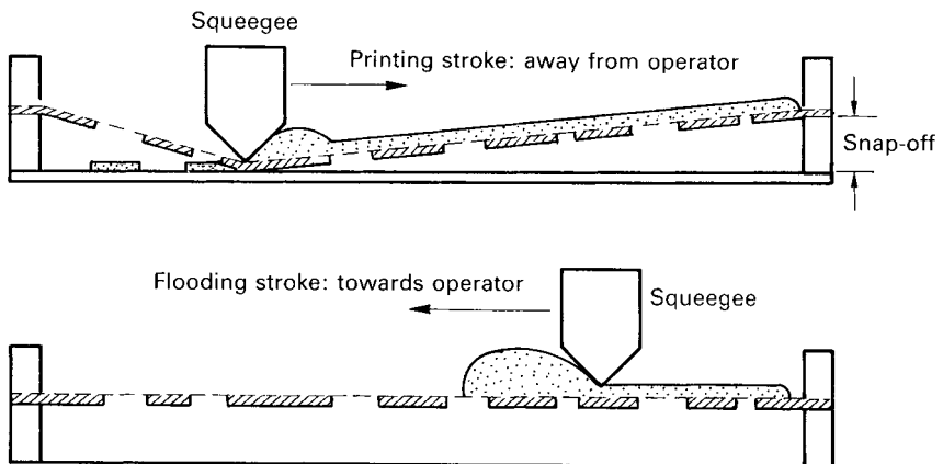
Figure 5.5 Screen printing by hand
