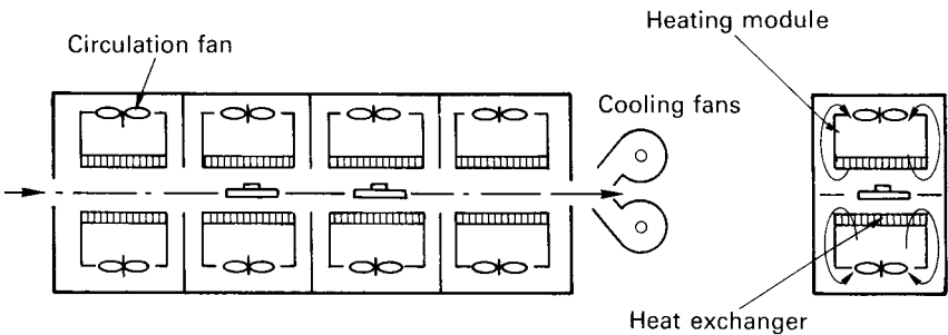
Figure 5.21 Working scheme of a convection soldering oven
