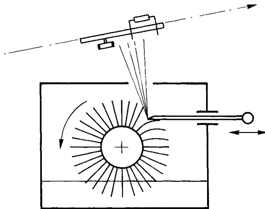
Figure 4.6 Working principle of a sprinkling fluxer
