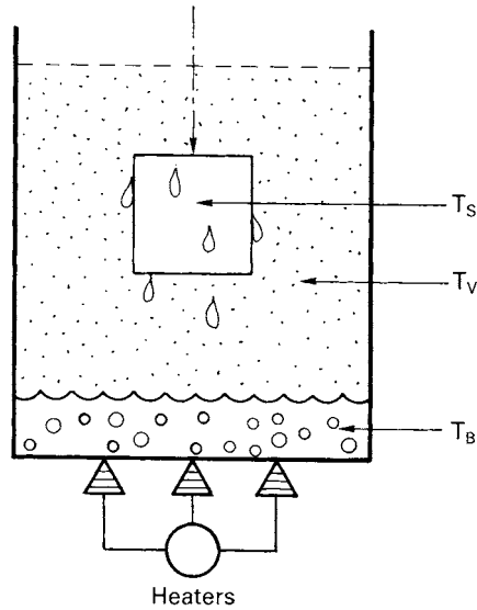
Figure 5.7 The working principle of vapourphase soldering. T_B = T_V = Boiling temperature of the working fluid; T_S = Temperature of the item to be soldered \leq T_V
