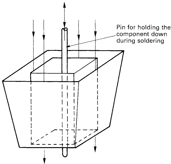
Figure 5.23 Hot-air nozzle for soldering a multilead component
