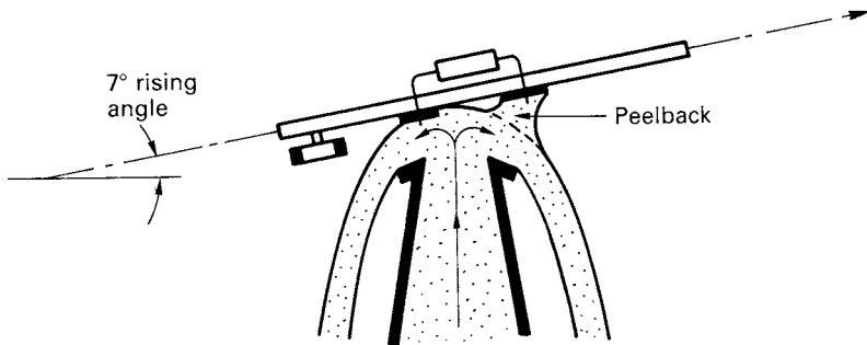
Figure 4.13 Peelback
