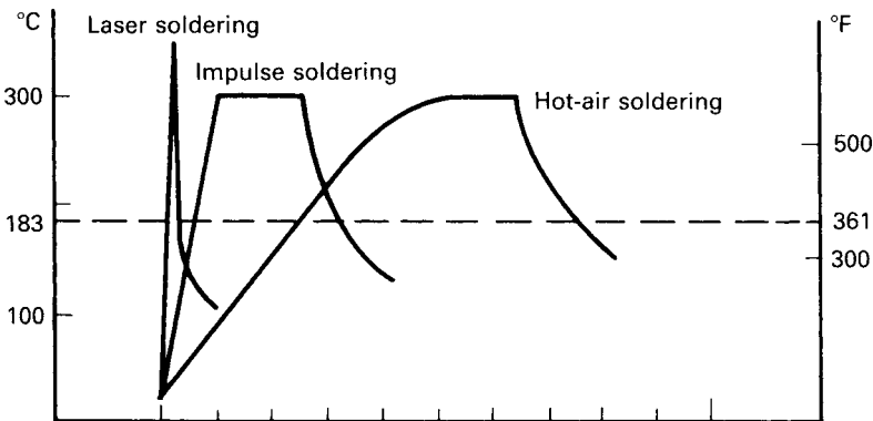
Figure 5.32 Temperature profiles of the different soldering methods
