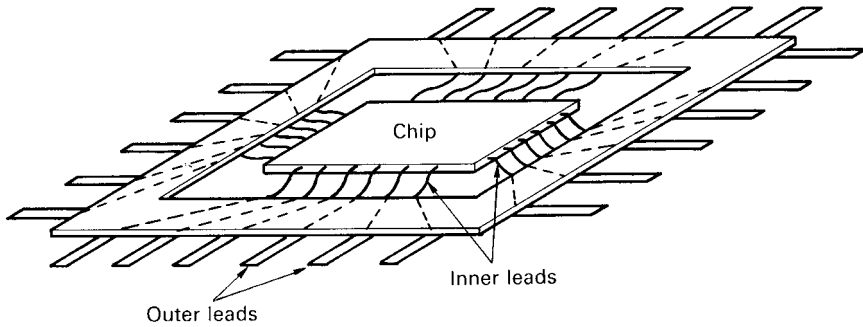
Figure 2.2 The TAB
