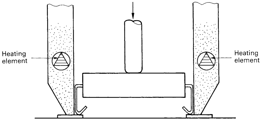
Figure 5.29 Thermode for PLCCs
