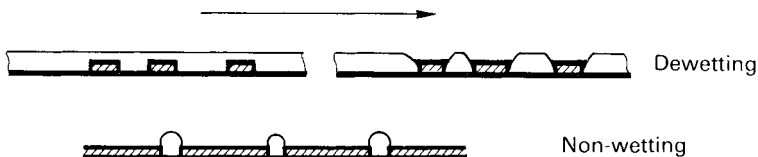
Figure 3.16 Dewetting and non-wetting
