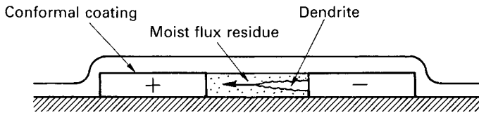
Figure 8.3 Formation of dendrites
