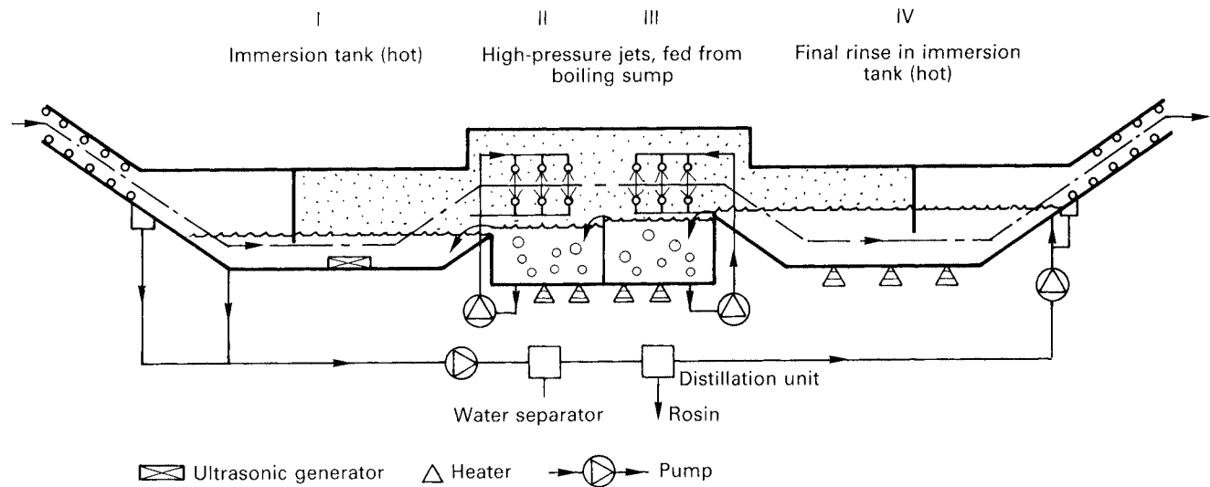
Figure 8.14 Combined jet and immersion cleaning machine (Electrovert)
