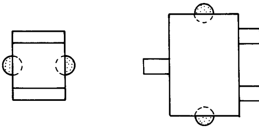
Figure 4.36 Location of adhesive spots for ultraviolet hardening
