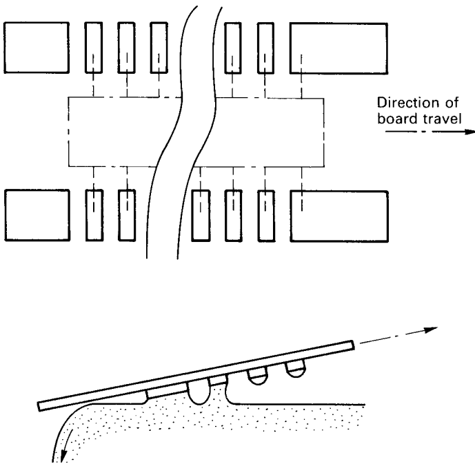
Figure 4.15 Peelback and solder thieves
