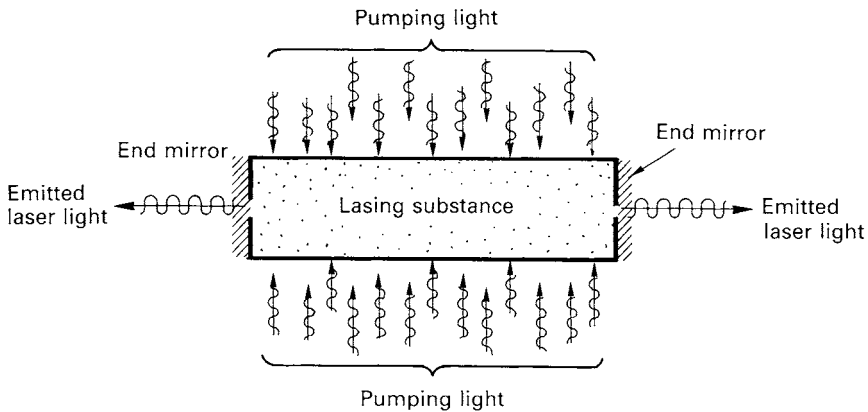
Figure 5.24 Working principle of a laser with emission at both ends
