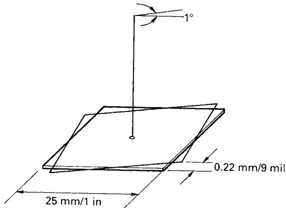
Figure 7.1 Angular accuracy of placement
