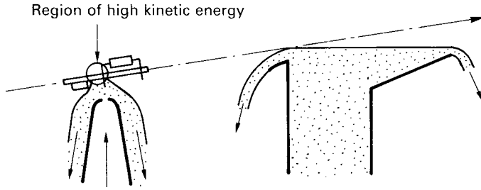
Figure 4.18 Turbulent primary wave
