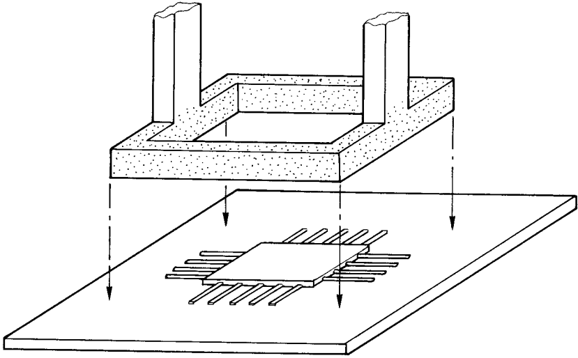
Figure 5.28 Thermode for ICs with flat leads
