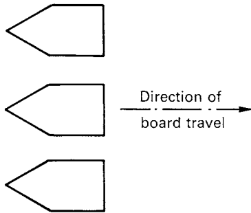
Figure 4.25 Shape of solderpads to minimize solderballing
