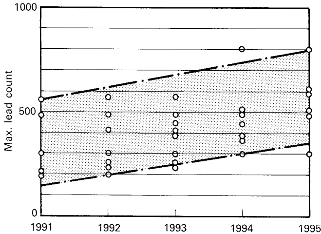
Figure 2.1 Maximum lead count trends (after E. J. Vardaman 4 ). General trend: +60 leads/year (courtesy Techsearch International Inc., Austin, Texas, USA)
