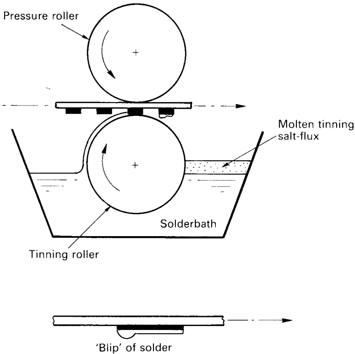
Figure 6.4 Rollertinning
