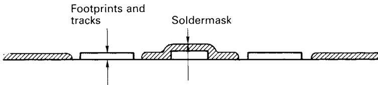
Figure 8.6 Height of various surface features on a circuit board. Footprints and tracks 35–135 \mu\text{m} /1.5–5.5 mil; soldermask lacquer 10–20 \mu\text{m} /0.4–0.8 mil; soldermask dry-film 50–100 \mu\text{m} /2–4 mil
