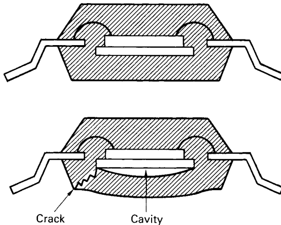
Figure 2.5 The popcorn effect
