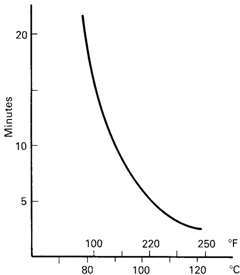
Figure 4.35 Hardening curve of an epoxy adhesive
