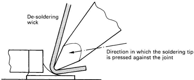
Figure 10.1 Desoldering a melf or chip with a solder-wick
