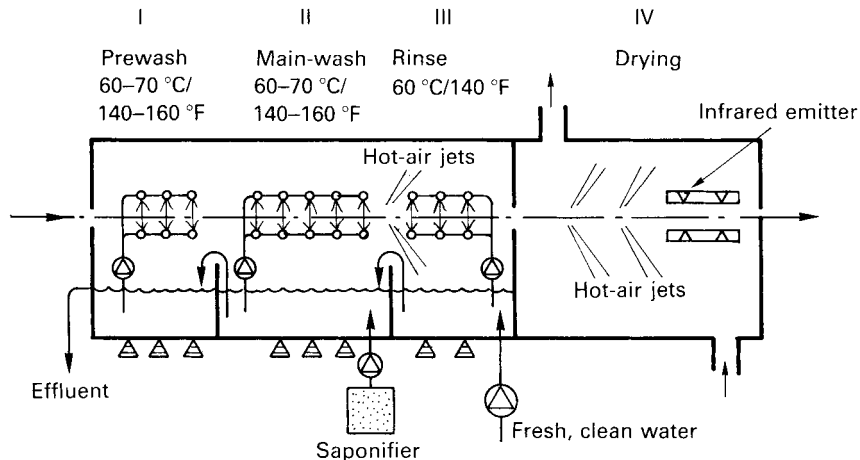
Figure 8.15 In-line water washing machine
