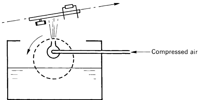
Figure 4.5 Working principle of a rotating-drum sprayfluxer
