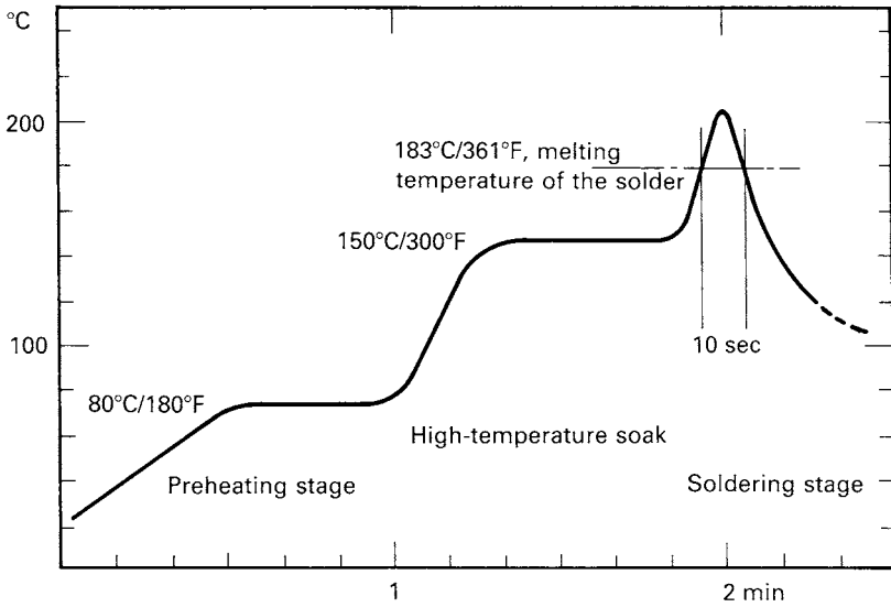
Figure 5.18 Idealized temperature profile of an infrared reflowsoldering operation
