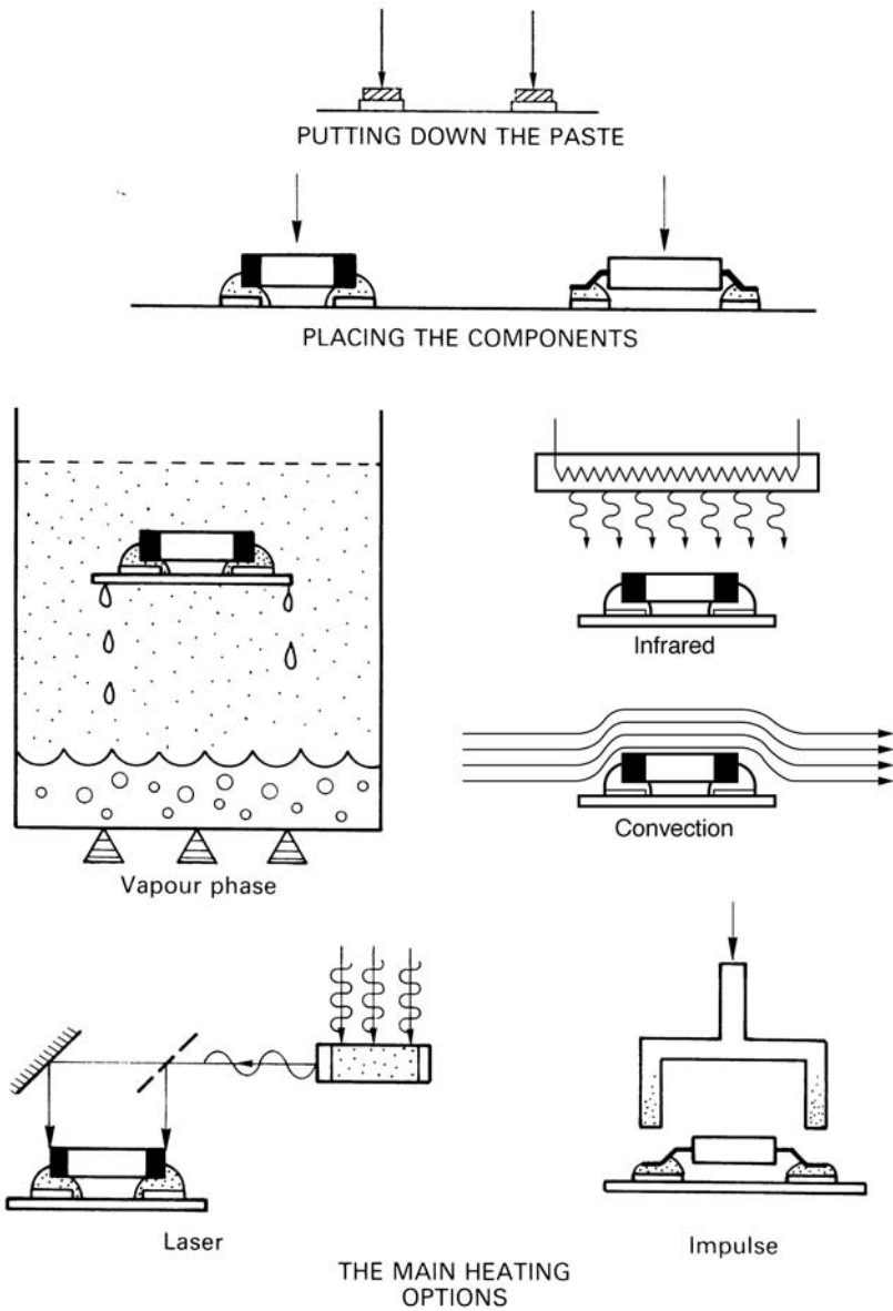
Figure 5.1 The reflow soldering options
