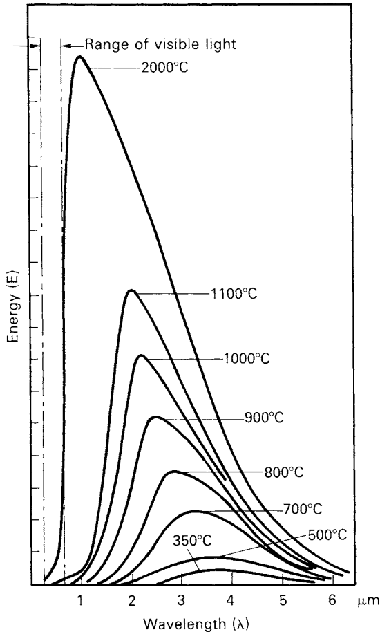
Figure 5.14 Distribution of emitted energy over the wavelength spectrum for different emitter temperatures
