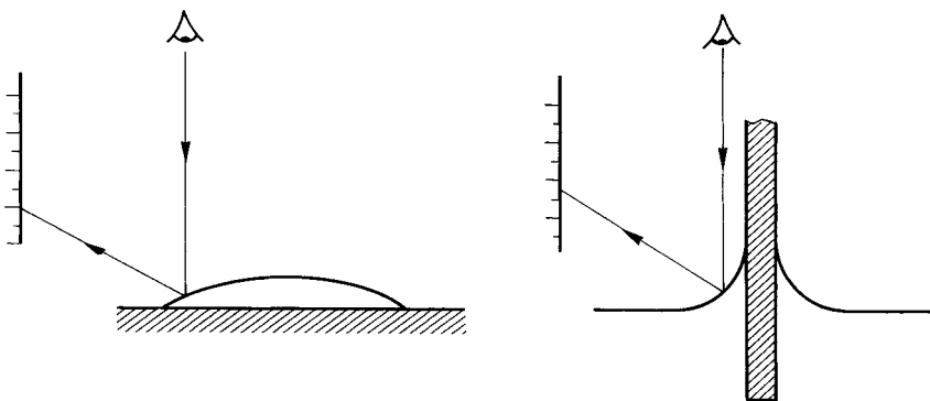
Figure 3.22 The solder meniscus and its assessment
