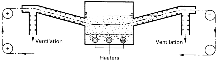
Figure 5.10 In-line vapourphase soldering system
