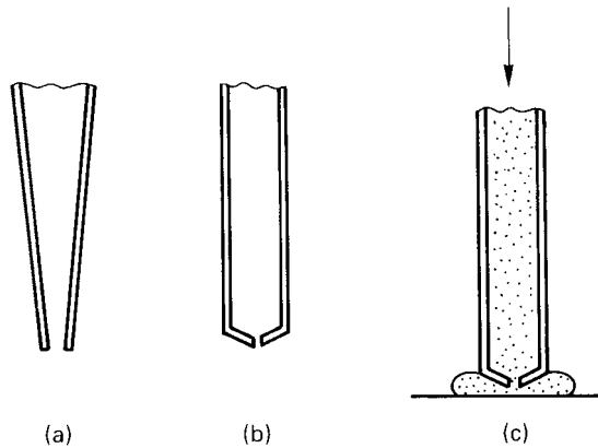
Figure 5.4 Placement of solder paste by dispensing. (a) Unsuitable nozzle shape; tends to block; (b) recommended nozzle shape; (c) nozzle too close to footprint; squashing of paste deposit
