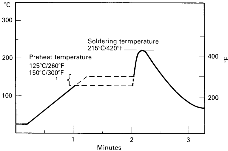
Figure 5.11 Temperature profile of vapourphase soldering with preheat
