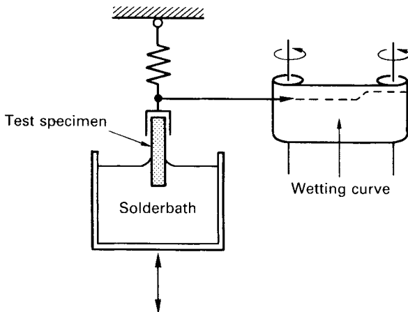
Figure 3.23 The wetting balance
