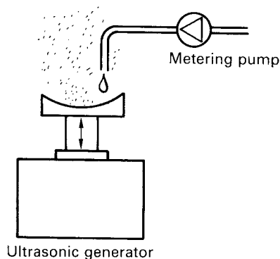
Figure 4.7 Working principle of ultrasonic atomization
