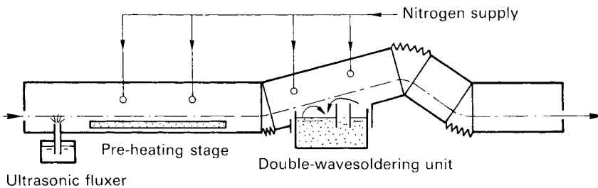
Figure 4.23 Wavesoldering under nitrogen (SEHO, Germany)
