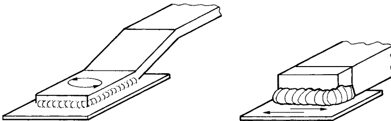
Figure 5.26 Oscillating laser spot
