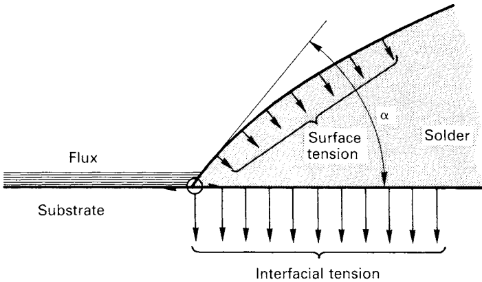
Figure 3.13 The wetting process as a balance between surface tension and interfacial tension. \alpha : Wetting angle
