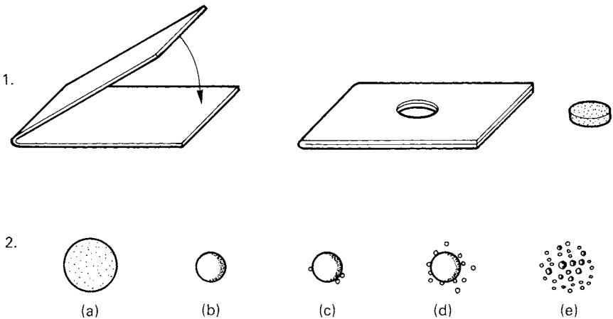
Figure 5.3 The solderballing test. 1. Making the stencil from a self-adhesive label; the paste printdown made with it; 2. Results: (a) paste printdown; (b), (c) acceptable results; (d), (e) unacceptable results
