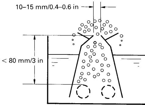
Figure 4.3 Critical design features of a foamfluxer
