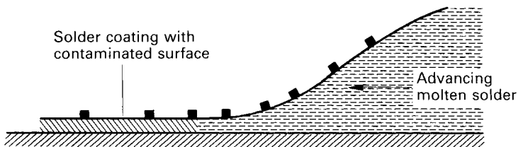
Figure 3.21 The lift-off effect
