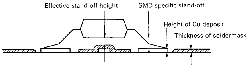
Figure 8.7 \text{Effective stand-off height} = \text{SMD-specific stand-off} - \text{thickness of soldermask}
