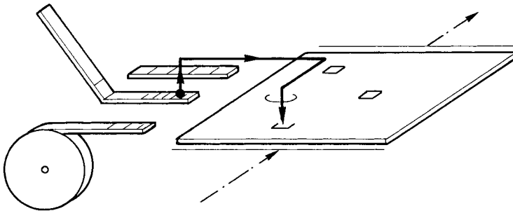
Figure 7.3 Sequential placement
