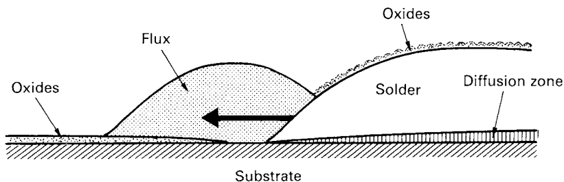
Figure 3.9 The function of the flux in soldering
