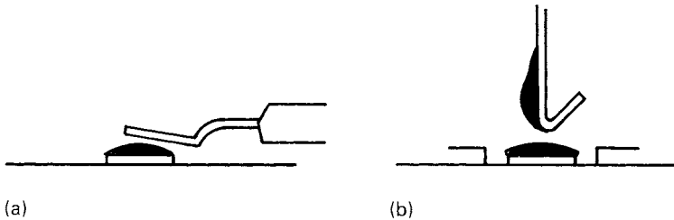
Figure 9.1 Open joints caused by: (a) lack of coplanarity; (b) wicking
