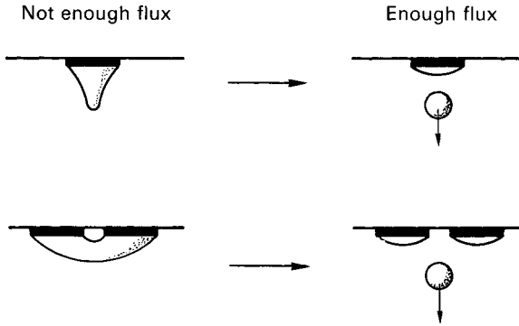
Figure 3.12 Icicles, bridges, and surface tension
