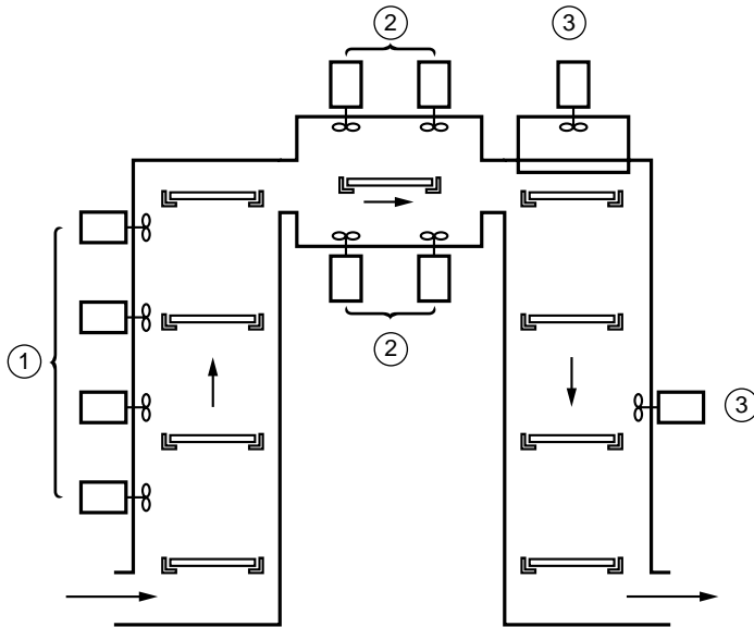
Figure 5.22 Vertical tower oven (SMT, Germany): 1, pre-heating section; 2, melting section; 3, cooling section
