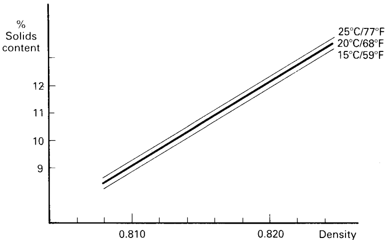
Figure 4.8 Flux-density/Solids-content curve
