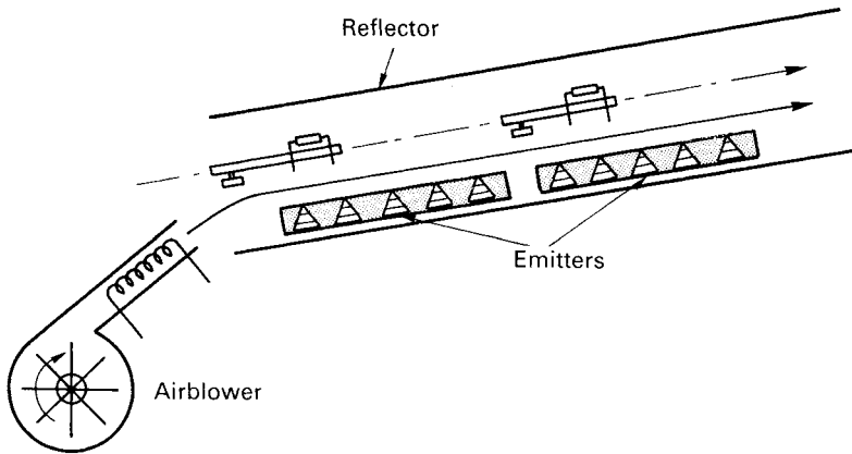
Figure 4.9 The preheating section
