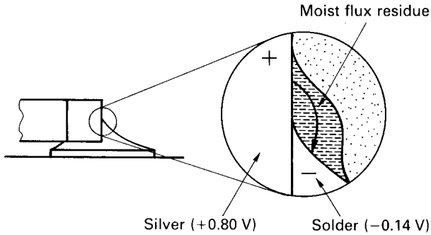
Figure 8.2 Electrolytic corrosion
