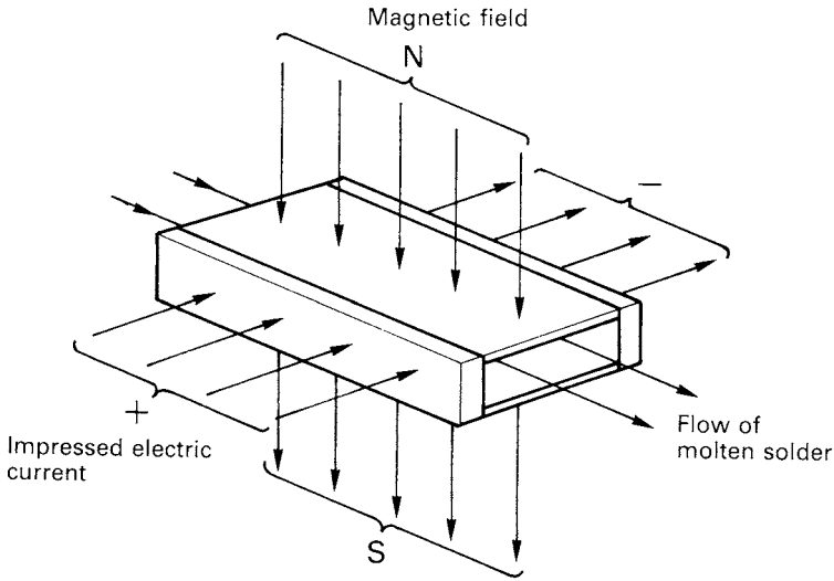
Figure 4.21 Electrodynamic solder pump (Kirsten)
