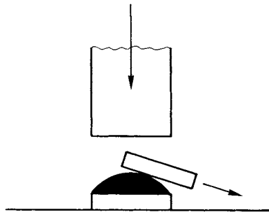
Figure 5.6 Danger of domed solder depot
