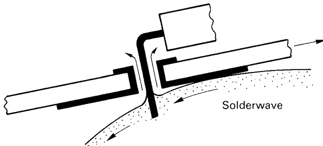
Figure 4.12 Wired joint entering the solderwave
