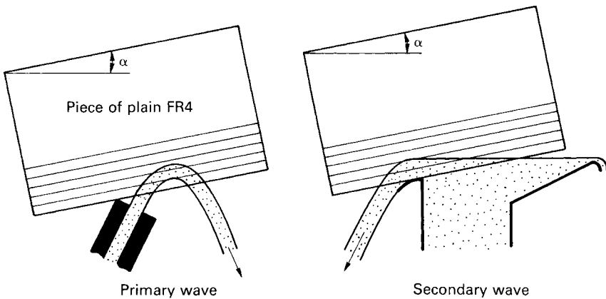
Figure 4.30 Checking the wave height. \alpha : Conveyor angle
