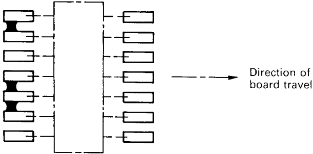
Figure 4.16 Bridging in a row of footprints aligned at right angles to the direction of travel
