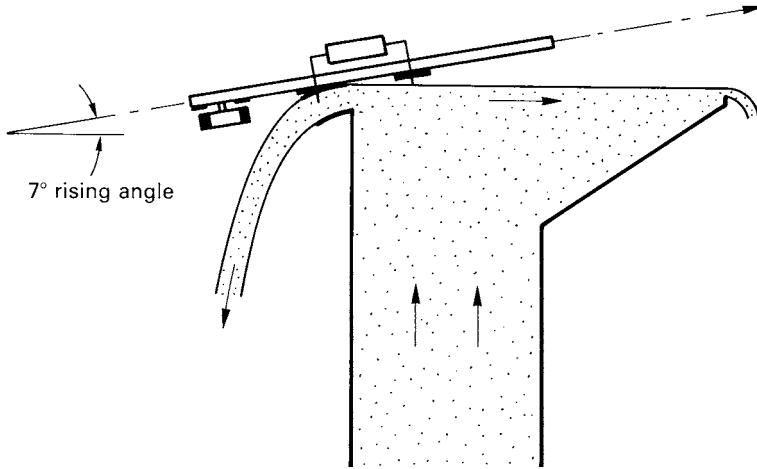
Figure 4.14 The movements of board and solder in an asymmetrical solder-wave
