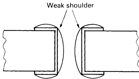
Figure 6.2 ‘Weak shoulder’ of HAL-tinned through-hole
