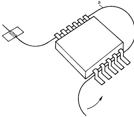
Figure 10.4 Desoldering a SOIC leg by leg (courtesy Edsyn Corp.)
