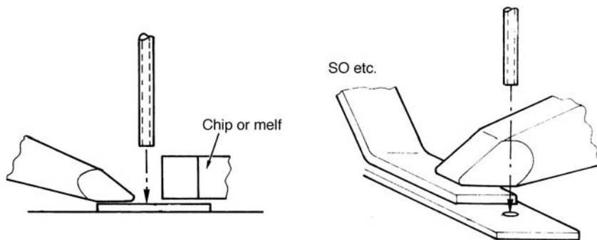
Figure 10.5 Filling an open joint with a soldering iron. Place the end of the solderwire on the footprint in spot (1). Then place the flat side of the soldering iron against the footprint or component leg as shown
