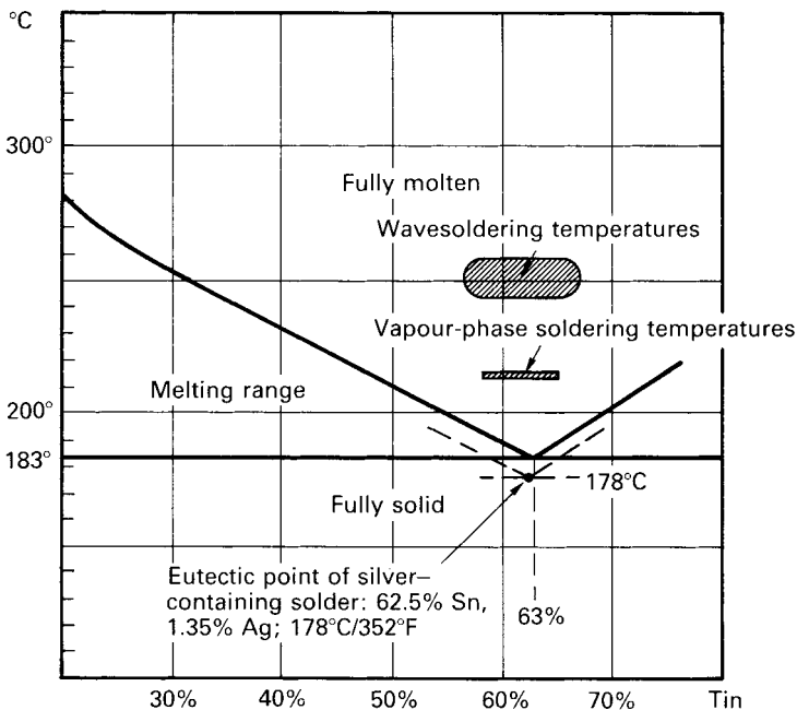
Figure 3.5 Electronic solders and their melting behaviour
