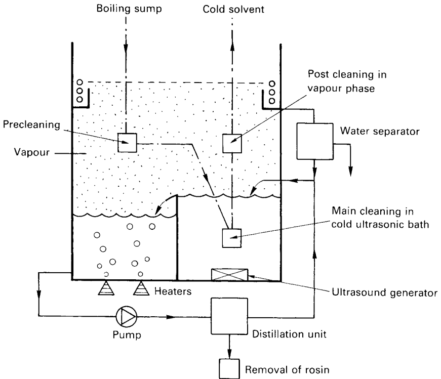
Figure 8.10 Twin-tank solvent cleaning unit
