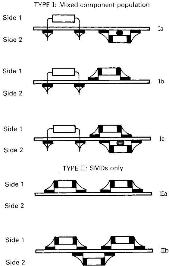
Figure 5.2 Options of board construction
