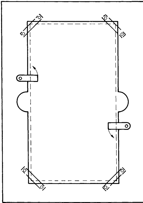
Figure 4.29 Soldering template
