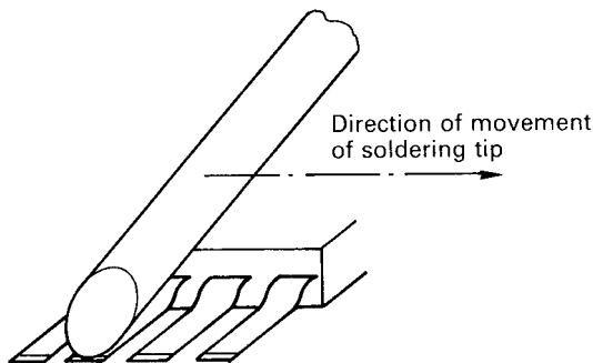
Figure 10.6 Soldering bit with an oblique endface (courtesy Pace Inc.)
