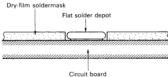
Figure 6.5 Flat solder depot
