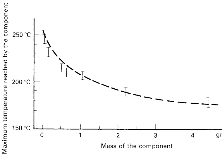
Figure 5.16 Component peak temperature versus mass during IR soldering [24]
