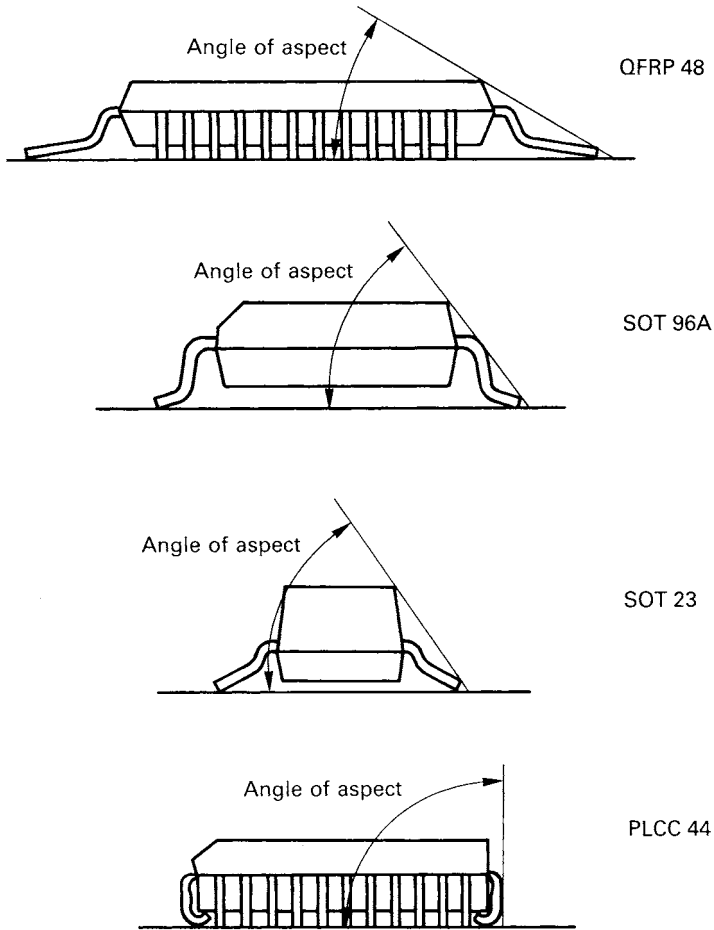
Figure 2.4 The contours of SOs, PLCCs and QFPs.
