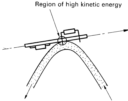
Figure 4.20 Single-wave soldering with a counterflow jetwave
