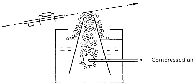
Figure 4.2 Working principle of a foamfluxer
