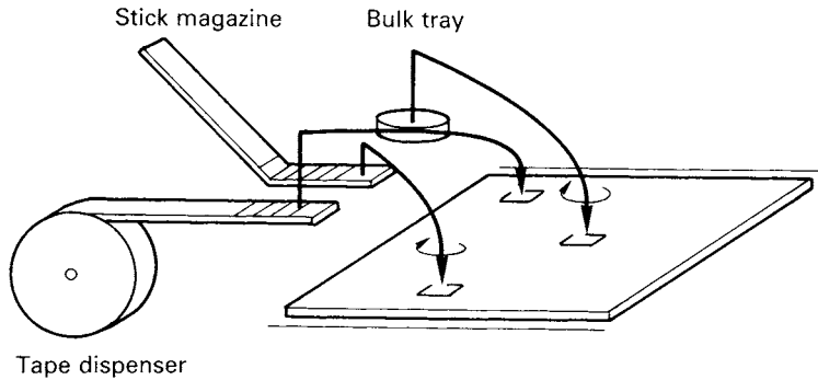
Figure 7.2 The basic tasks of manual placement
