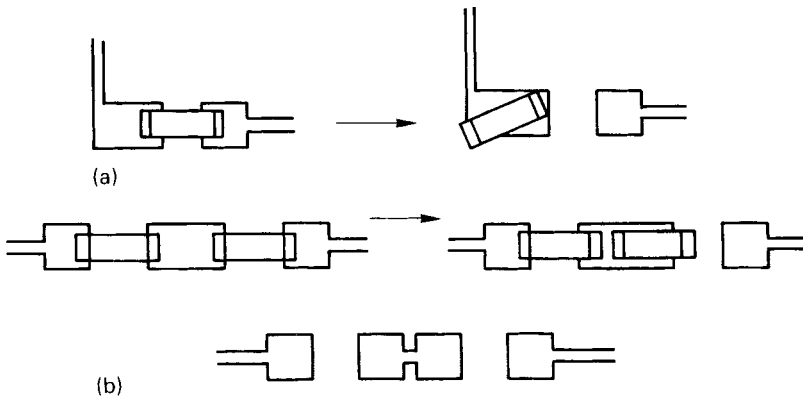
Figure 6.10 The dangers of asymmetry. (a) Floating caused by lack of symmetry between left and right footprint areas; (b) remedy
