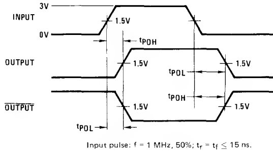
FIGURE 1. Propagation Delays
