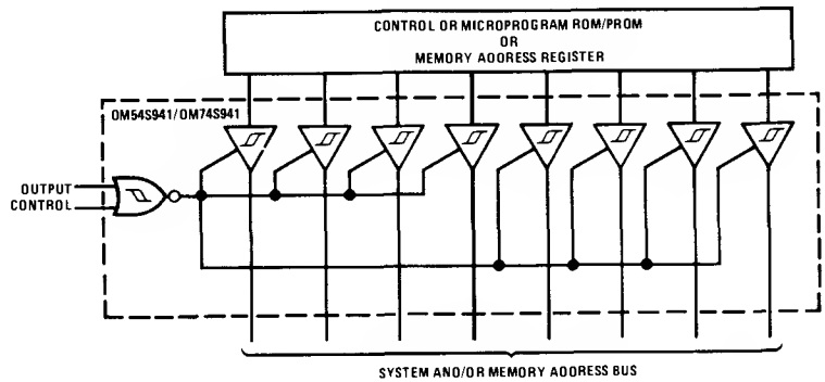
DM54S941/DM74S941
