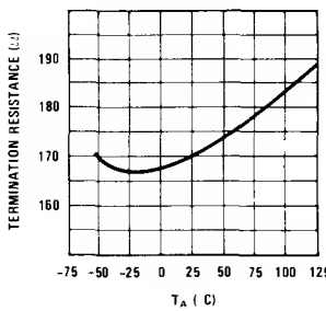
Termination Resistance
