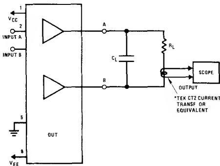
FIGURE 4. TRI-STATE® Delays for DS1692/DS3692
