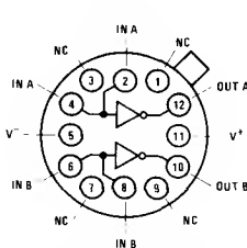
TO-8 Package
