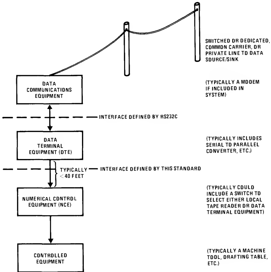
FIGURE 13. EIA RS488 Interface Applications
