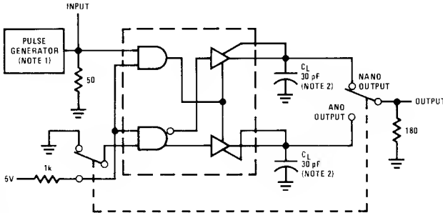
FIGURE 2. t_{pZH} and t_{pHZ}
