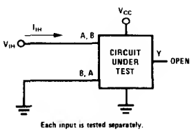
FIGURE 2. I IH
