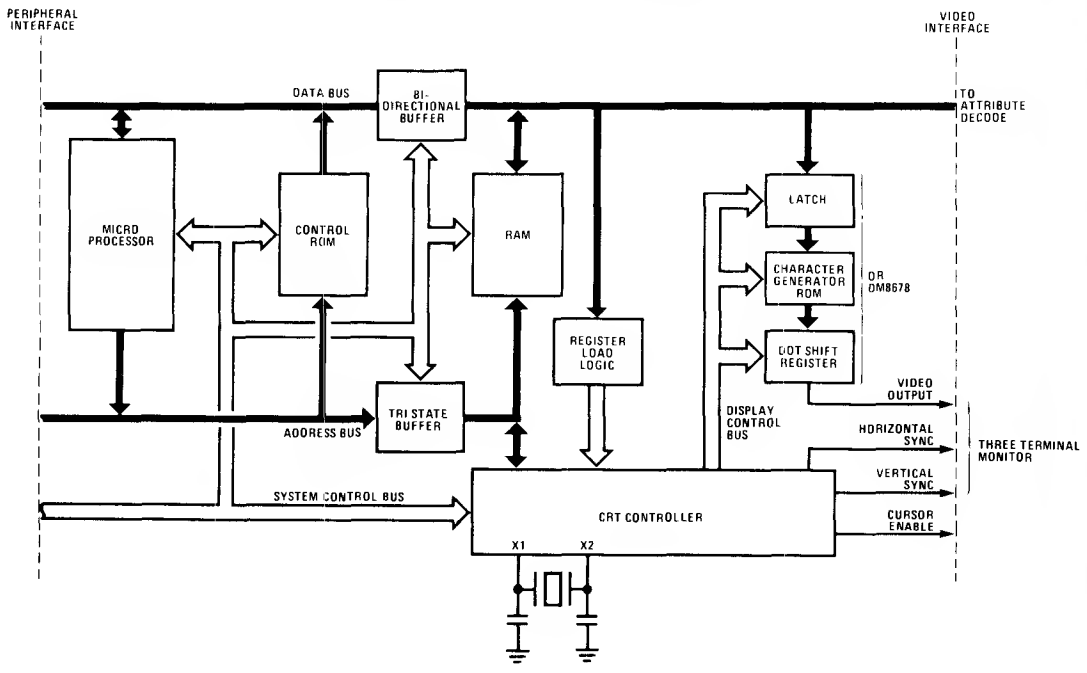
Figure 7. System Diagram with no Line Buffer
