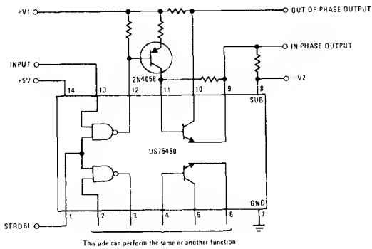
FIGURE 22. Floating Switch
