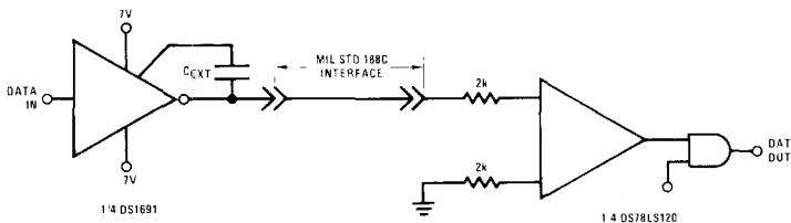
FIGURE 4. MIL-STD-188C Application
