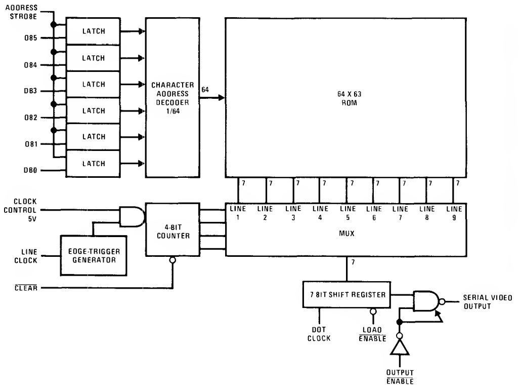
FIGURE 3. DM8678 Character Generator Block Diagram
