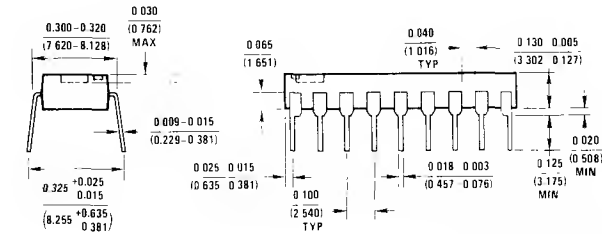
NS Package N18A 18-Lead Molded DIP (N)
