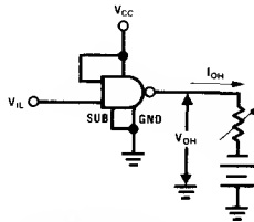
FIGURE 2. V_{IL} , V_{OH}
