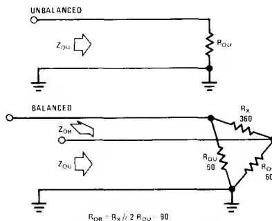
FIGURE 16. Impedance Measurement
