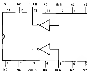
Flat Package
