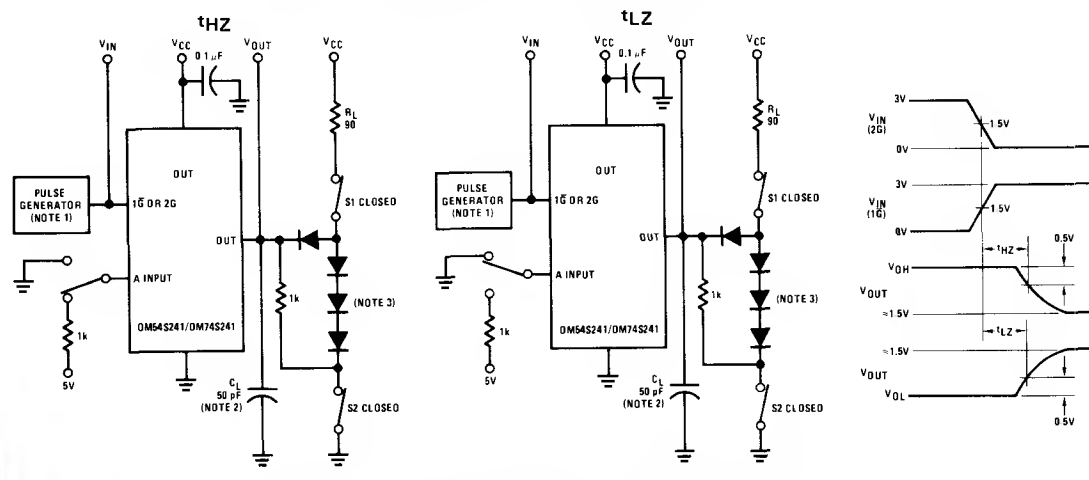
FIGURE 6. Propagation Delay to TRI-STATE from High or Low Level
