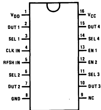
TDP VIEW
