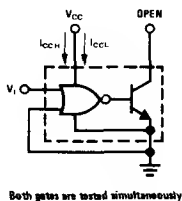
FIGURE 5. I_{CCH} , I_{CCL} for OR, NOR Circuits
