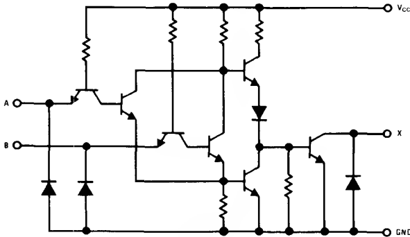
DS3613 Dual OR Peripheral Driver
