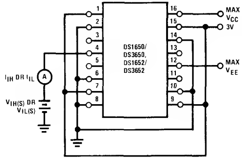
FIGURE 3. I_{1H(S)} and I_{1L(S)}
