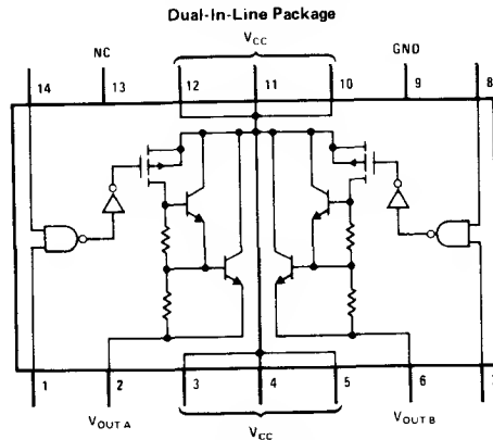
Order Number MM74C918N See NS Package N14A
