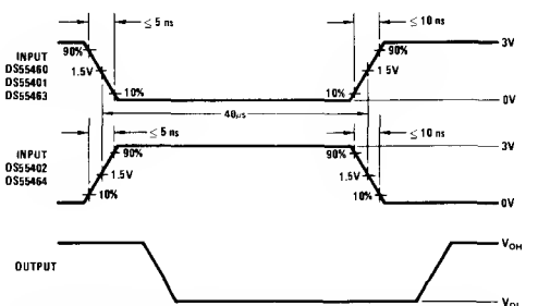
FIGURE 14. Switching Times of Complete Drivers
