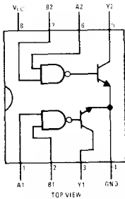
Order Number DS55461J-8, DS75461J-8 or DS75461N-8
