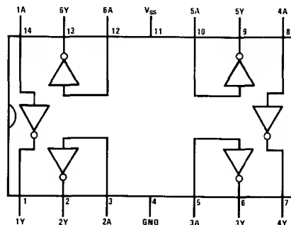
Dual-In-Line Package
