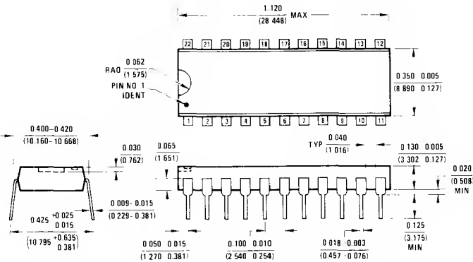
NS Package N22A 22-Lead Molded DIP (N)
