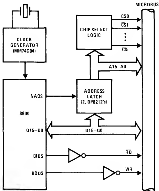
FIGURE 11. 8900 System Model
