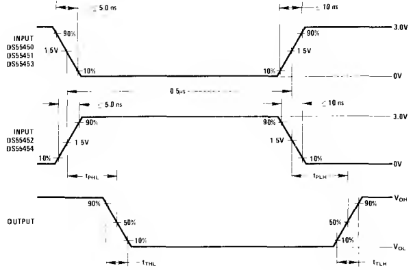
FIGURE 14. Switching Times of Complete Drivers
