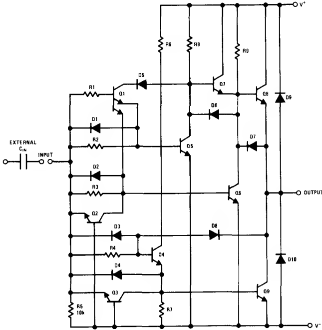
1/2 DS0026
