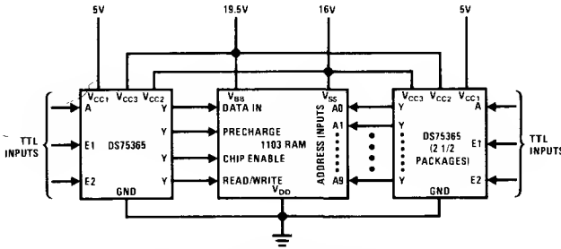
FIGURE 2. Interconnection of DS75365 Drivers With 1103-Type Silicon-Gate MOS RAM
