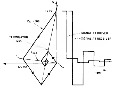
FIGURE 12. Line Reflection Diagram of Fall Time
