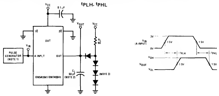
FIGURE 7. Propagation Delay from A Input to Y Output
