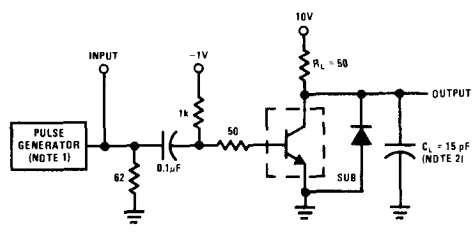
FIGURE 13. Switching Times, Each Transistor (DS55450/DS75450 Only)
