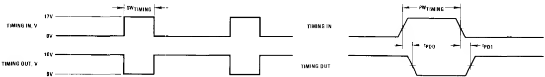
FIGURE 5. DS8694 Timing Signal Buffer
