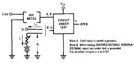
FIGURE 8. V_I , I_{IL}
