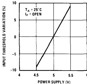
Input Threshold vs Power Supply Variation
