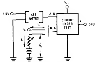
FIGURE 8. V_I , I_{IL}
