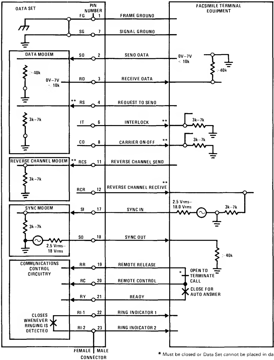
FIGURE 12. Functional and Electrical Characteristics of RS357
