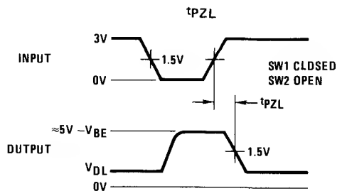
FIGURE 2. Propagation Delay TRI-STATE Control Input to Output
