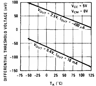
Temperature Sensitivity
