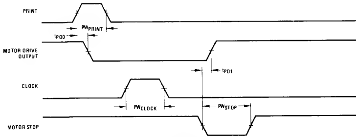
FIGURE 6. DS8693 Motor Drive Latch
