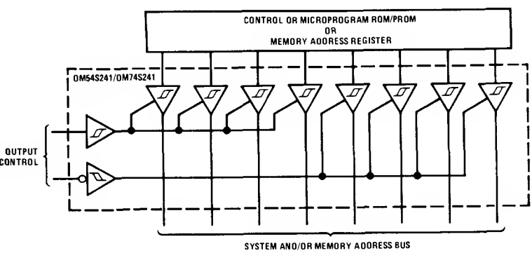
DM54S241/DM74S241
