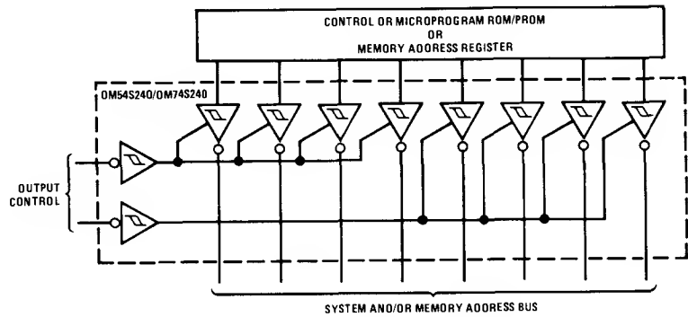
DM54S240/DM74S240, DM54S940/DM74S940
