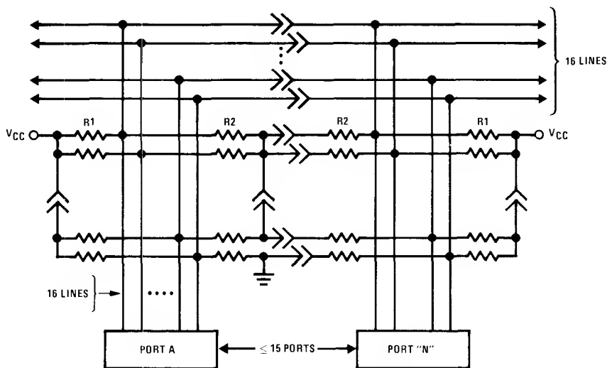
FIGURE 8. IEEE 488 Application
