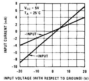
Input Characteristics
