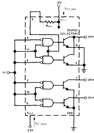
FIGURE 6. I_{CC1}(\text{OFF}) and I_{CC2}(\text{OFF})
