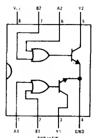
Order Number DS55454J-8, DS75454J-8 or DS75454N-8
