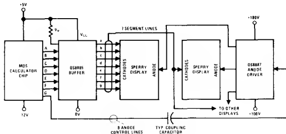
FIGURE 6. Fully Decoded MOS Cathode Outputs
