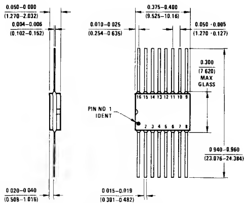
NS Package W16A 16-Lead Flat Package (W)
