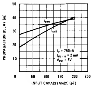
Typical Propagation Delay vs Input Capacitance DS3606
