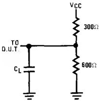
Test Load
