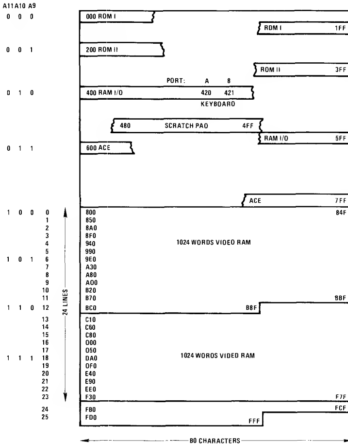
FIGURE 3. Memory Map
