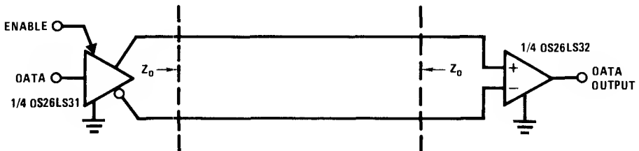
Two-Wire Balanced System, RS-422
