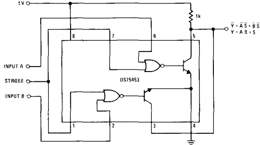
FIGURE 32. Logic Signal Comparator
