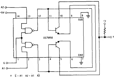
FIGURE 20. Gated Comparator
