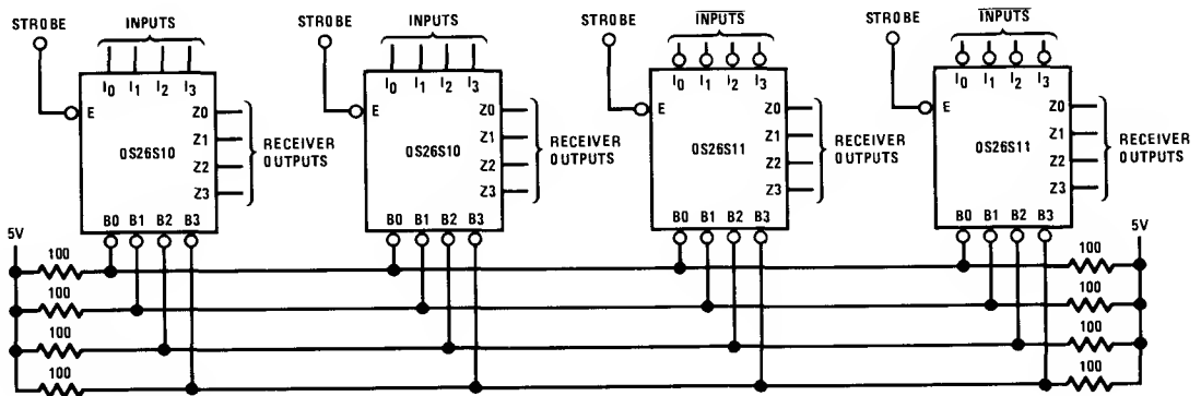
100 PARTY-LINE OPERATION
