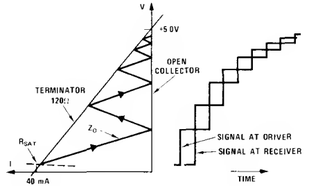
FIGURE 11. Line Reflection Diagram of Rise Time
