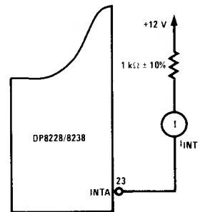
FIGURE 3. INTA Test Circuit (For RST 7)
