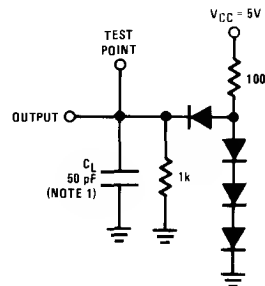
FIGURE 2. B Port Load, DS3647, OS3677
