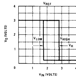
Transfer Characteristics and Equations for Level Detector with Hysteresis
