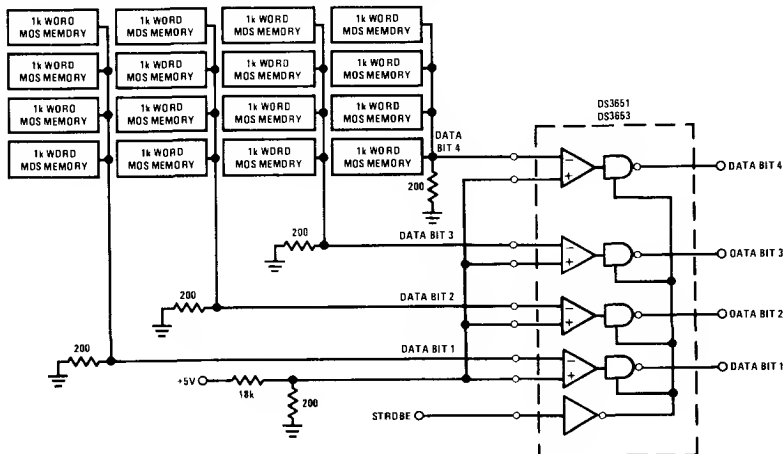
A Typical MOS Memory Sensing Application for a 4k word by 4-bit memory arrangement employing 1103 type memory devices
