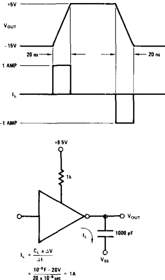
FIGURE 8. Clock Waveforms (Voltage and Current)
