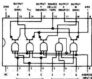
Dual-In-Line Package
