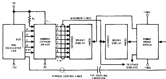
FIGURE 4. BCD Data Interfacing Directly With MOS Output
