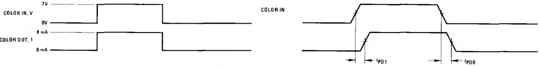
FIGURE 4. DS8693 Color Driver
