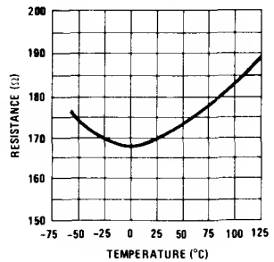
Termination Resistance
