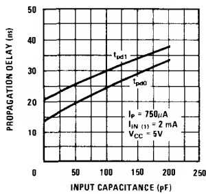
Typical Propagation Delay vs Input Capacitance DS3608
