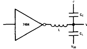
FIGURE 9. Clock Coupling
