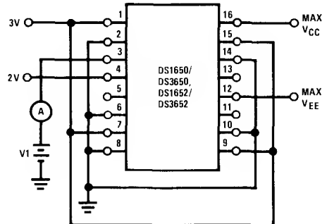
FIGURE 7. I_{OFF}
