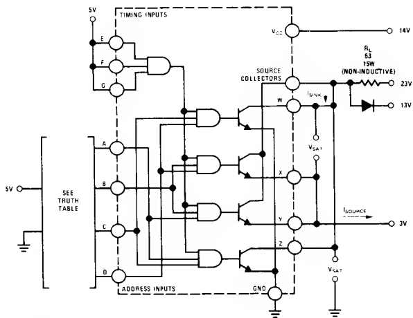
FIGURE 2. V_{SAT}
