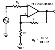
Level Detector with Hysteresis
