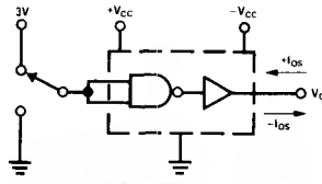
FIGURE 4. I OS
