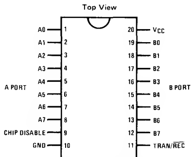
Dual-In-Line Package Order Numbers: DP8304BN, DP8304BJ, DP7304BJ See NS Package J20A or N20A
