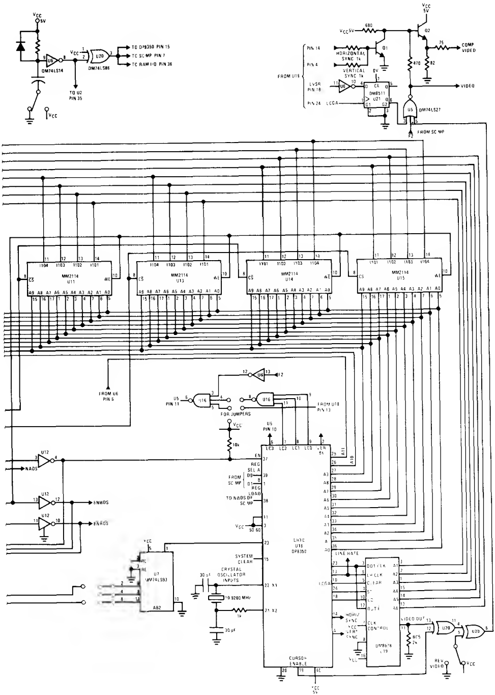
FIGURE 6. Low Cost CRT Terminal (Continued)
