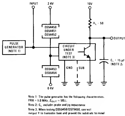
FIGURE 14. Switching Times of Complete Drivers
