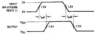
FIGURE 4. MBI/O Bus
