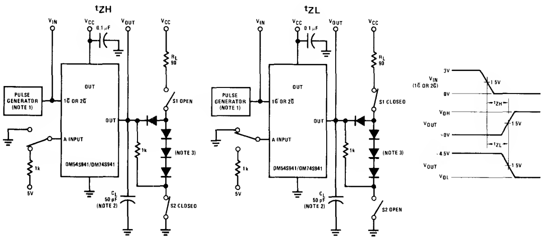
FIGURE 8. Propagation Delay from TRI-STATE to High or Low Level
