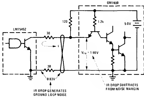
FIGURE 9. Unbalanced Method
