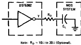
FIGURE 2. Use of Damping Resistor to Reduce or Eliminate Output Transient Overshoot In Certain DS75362 Applications.
