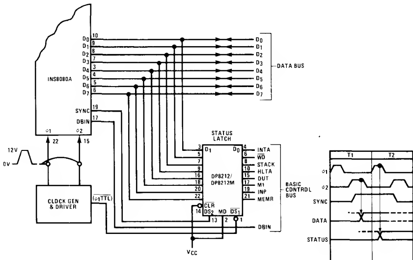
INS8080A Status Latch
