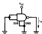
FIGURE 5. I_{Os}
