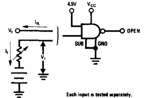
FIGURE 3. V_I , I_{IL}
