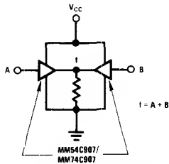
Wire OR Gate
