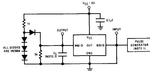
FIGURE 6. BOI/O to MBI/O ac Loads
