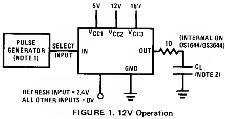
FIGURE 1. 12V Operation
