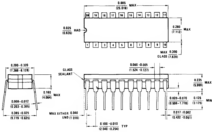
NS Package J20B 20-Lead Cavity DIP (J)
