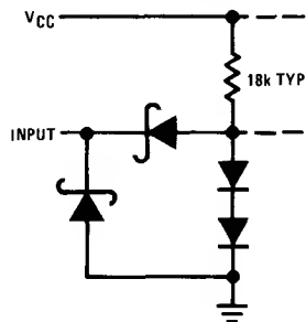
Equivalent of Output Control Clock Inputs
