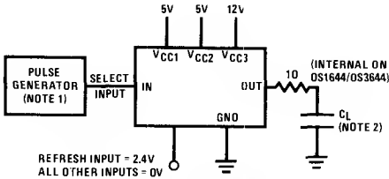
FIGURE 3. 5V Operation
