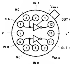
TO-8 Package
