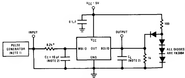
*This input network simulates the actual drive characteristic of the PACE outputs FIGURE 5. MBI/O to BOI/O ac Loads
