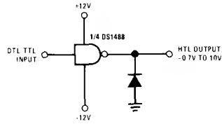
DTL/TTL-to-HTL Translator
