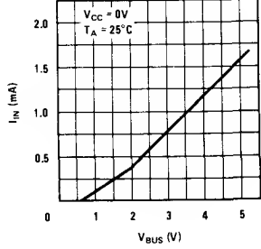
Receiver OFF Impedance
