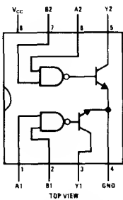
Order Number DS1611J-8, DS3611J-8 or DS3611N-8
