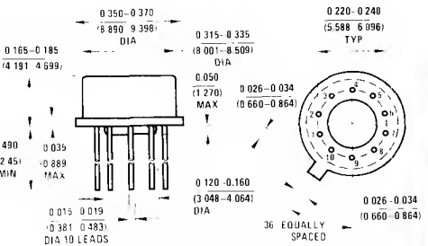
NS Package H10C 10-Lead TO-5 Metal Can Package (H) (Low Profile)
