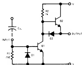
FIGURE 1. DS0025 Schematic (One-Half Circuit)
