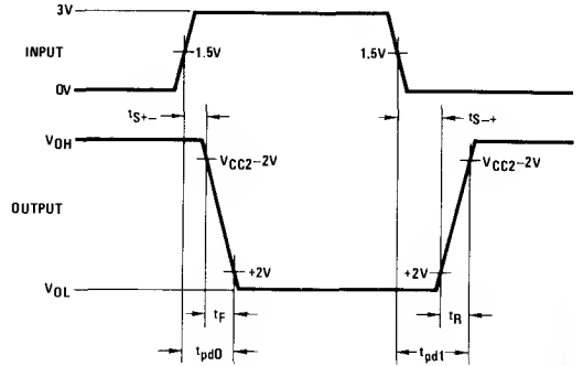
FIGURE 2. 12V Operation
