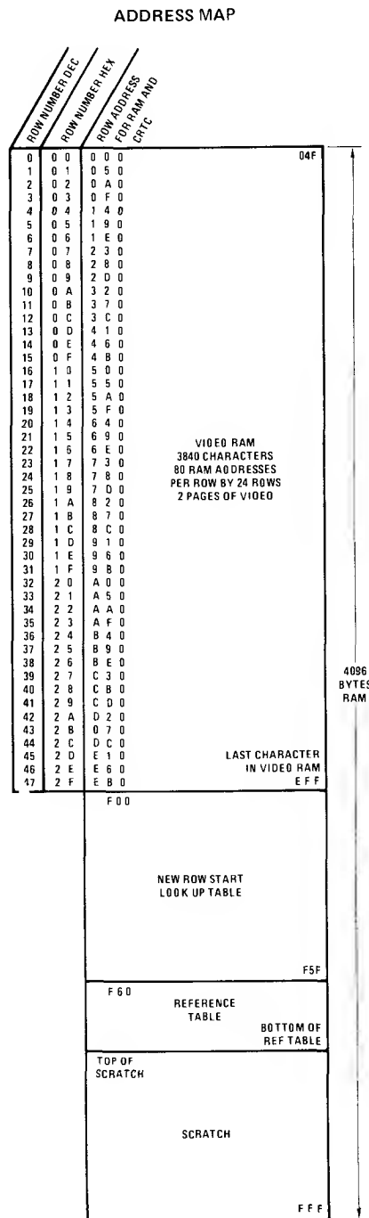
FIGURE 4. RAM Organization
