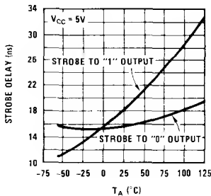
Strobe Delays
