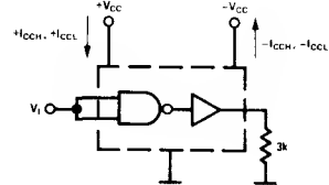
FIGURE 5. I CCH+ , I CCH- , I CCL+ , I CCL-
