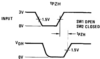
FIGURE 2. Propagation Delay TRI-STATE Control Input to Output
