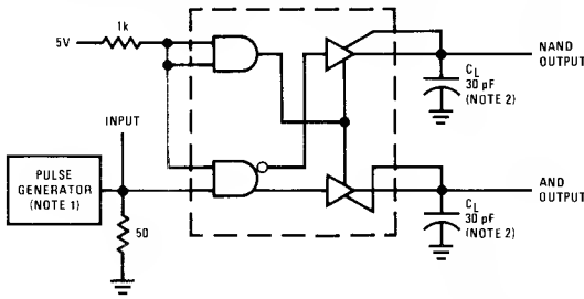
FIGURE 1. t_{pLH} and t_{pHL}
