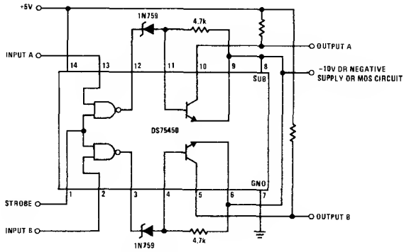
FIGURE 25. Dual TTL-to-MOS Driver
