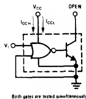
FIGURE 11. I_{OCH} , I_{OCL} for OR, NOR Circuits
