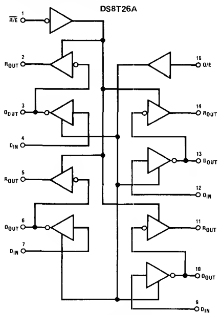
Dual-In-Line Package
