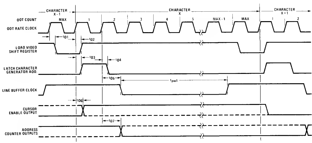
Figure 1. Dot/Character Rate Timing
