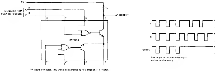
FIGURE 33. In-Phase Detector
