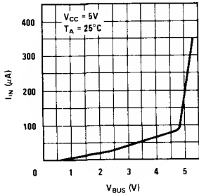
Receiver ON Impedance
