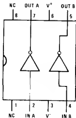
Quad-In-Line Package
