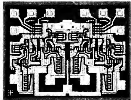
FIGURE 8. Photomicrograph of the DS7830 Dual Line Driver
