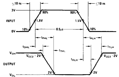
FIGURE 1. Switching Times, Each Driver
