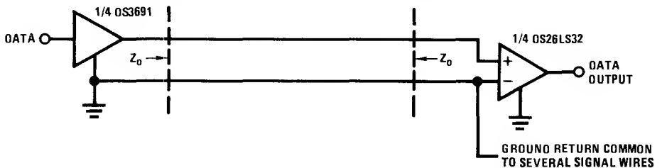
Single Wire with Common Ground Unbalanced System, RS-423
