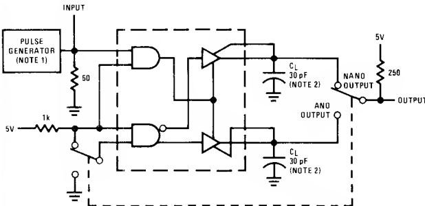
FIGURE 3. t_{pZL} and t_{pLZ}
