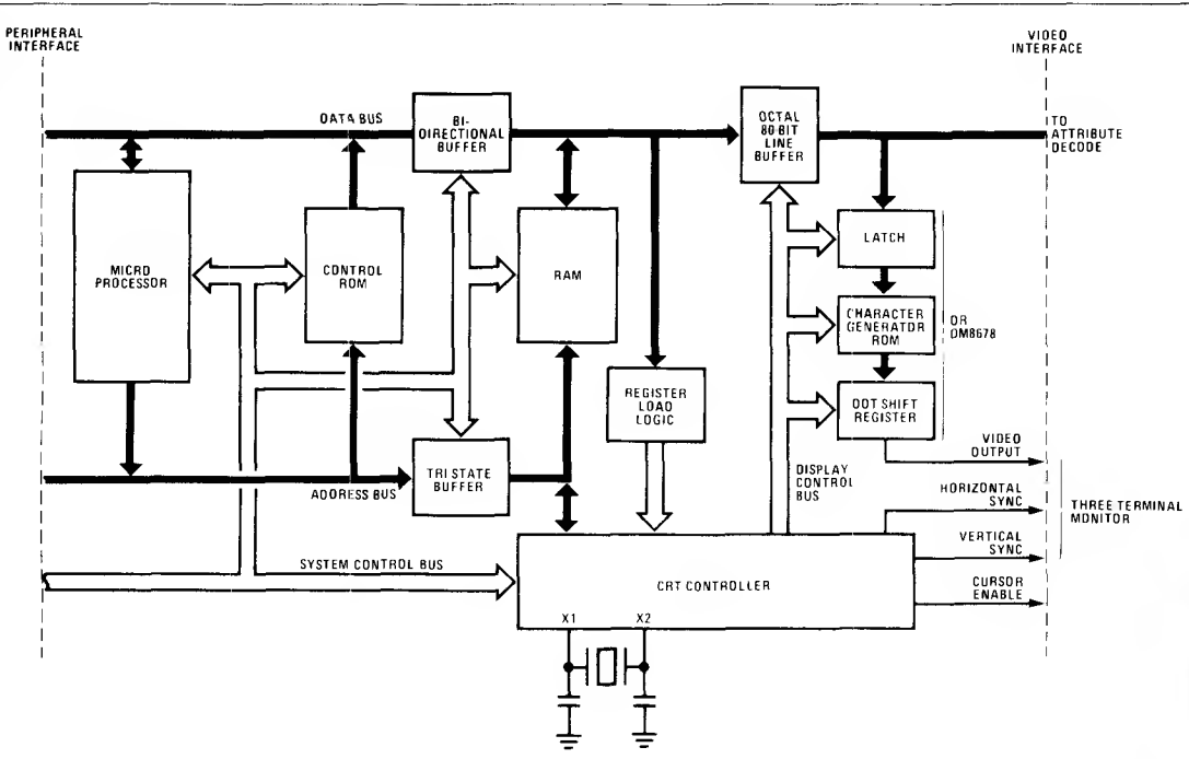
Figure 6. System Diagram Using a Line Buffer
