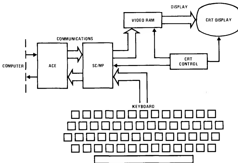
FIGURE 4. Block Diagram of an Interactive Terminal
