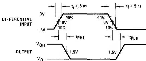
FIGURE 1. Propagation Delay Times
