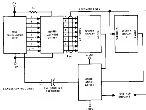
FIGURE 9. Decoded Cathode Data Direct Coupled From MOS Output
