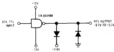
DTL/TTL-to-RTL Translator
