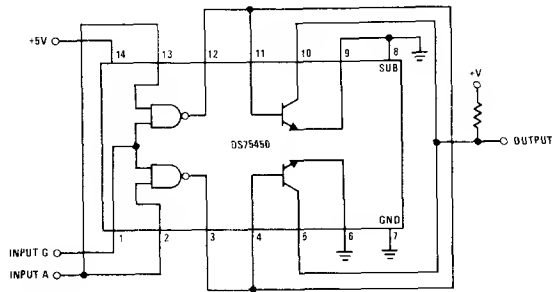
FIGURE 21. 500 mA Sink
