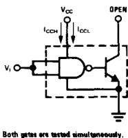
FIGURE 4. I_{CCH} , I_{CCL} for AND, NAND Circuits
