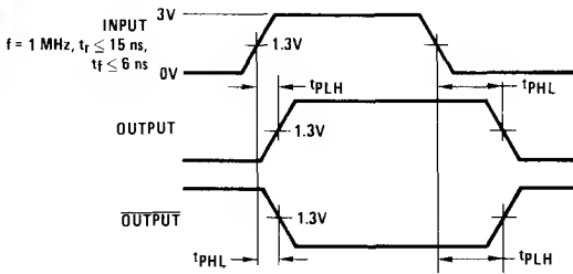
FIGURE 2. Propagation Delays
