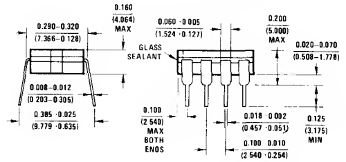
NS Package J08A 8-Lead Cavity DIP (J)
