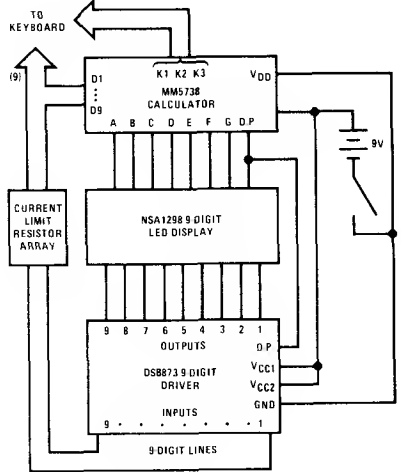
FIGURE 2. 9V System
