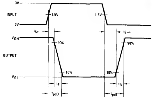
FIGURE 4. 5V Operation
