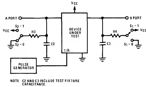
FIGURE B. Propagation Delay from \bar{T}/\bar{R} to A Port or B Port
