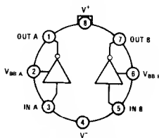
TO-5 Package
