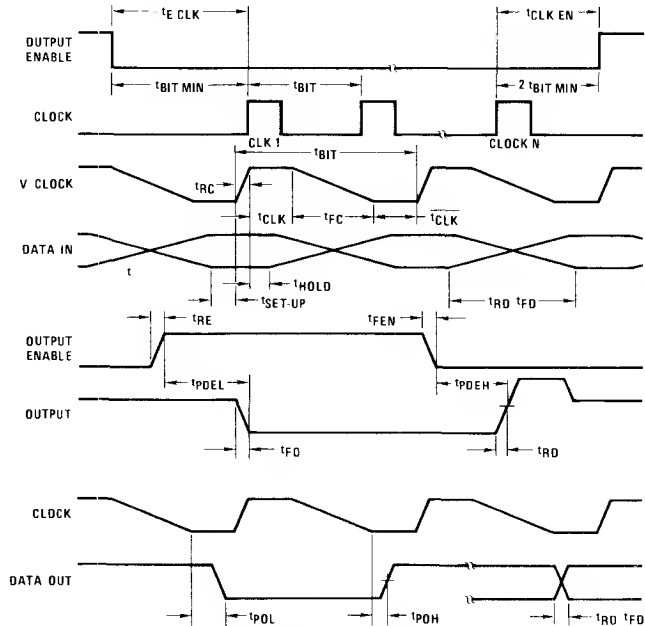
FIGURE 1. Shift Timing
