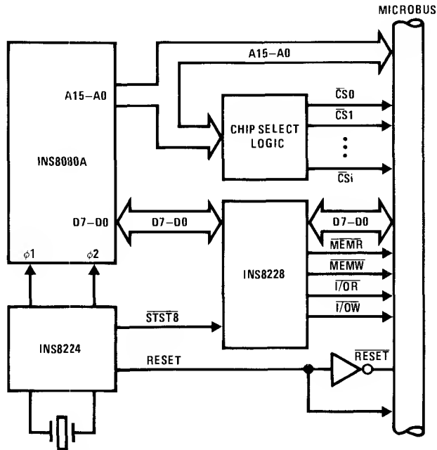
FIGURE 10. 8080 System Model for the Basic Microbus Interface
