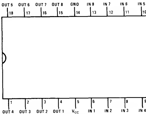
Order Number DS8654N See NS Package N18A
