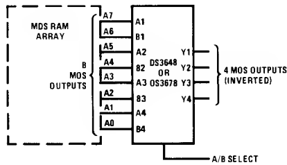
2:1 Multiplexing of RAM Outputs
