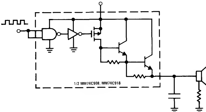
FIGURE 12c. Speaker Driver
