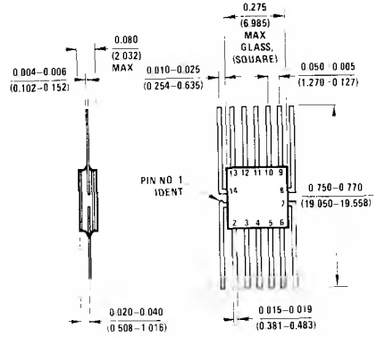
NS Package F14A 14-Lead Flat Package (F)
