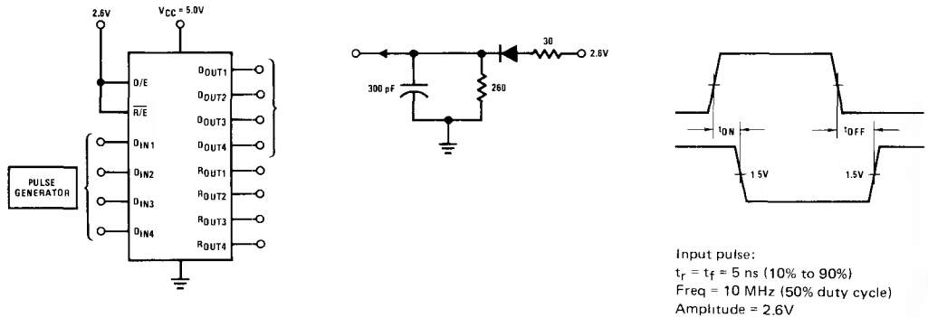
FIGURE 2. Propagation Delay ( D_{IN} to D_{OUT} )
