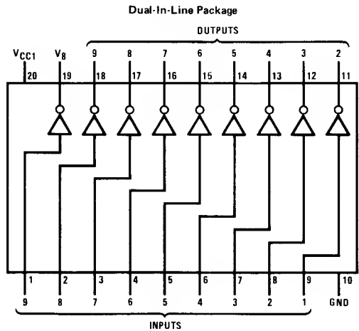
TOP VIEW Order Number DS8978N See NS Package N20A
