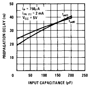
Typical Propagation Delay vs Input Capacitance DS3607
