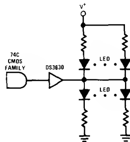
LED Driver
