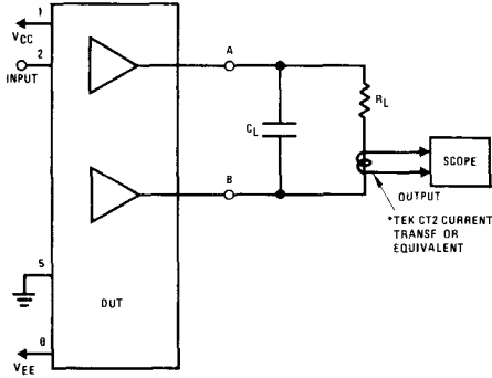
FIGURE 1. Differential Connection
