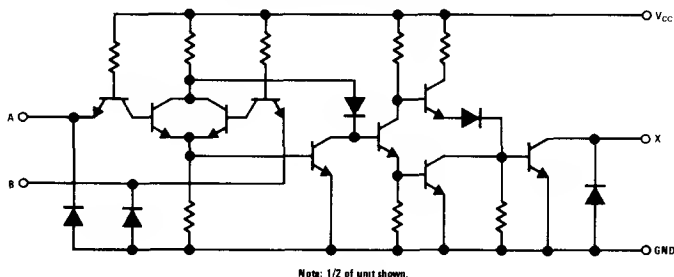
DS3614 Dual NOR Peripheral Driver
