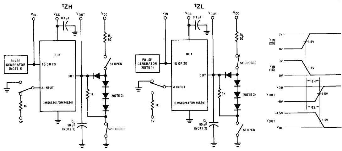
FIGURE 5. Propagation Delay from TRI-STATE to High or Low Level
