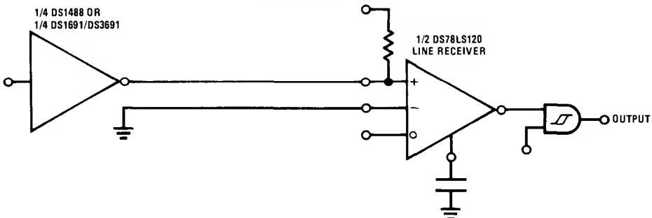
Unbalanced Data Transmission
