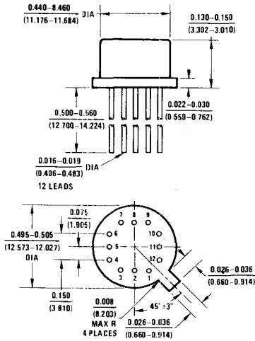
NS Package H12C 12-Lead TO-8 Metal Can Package (G)
