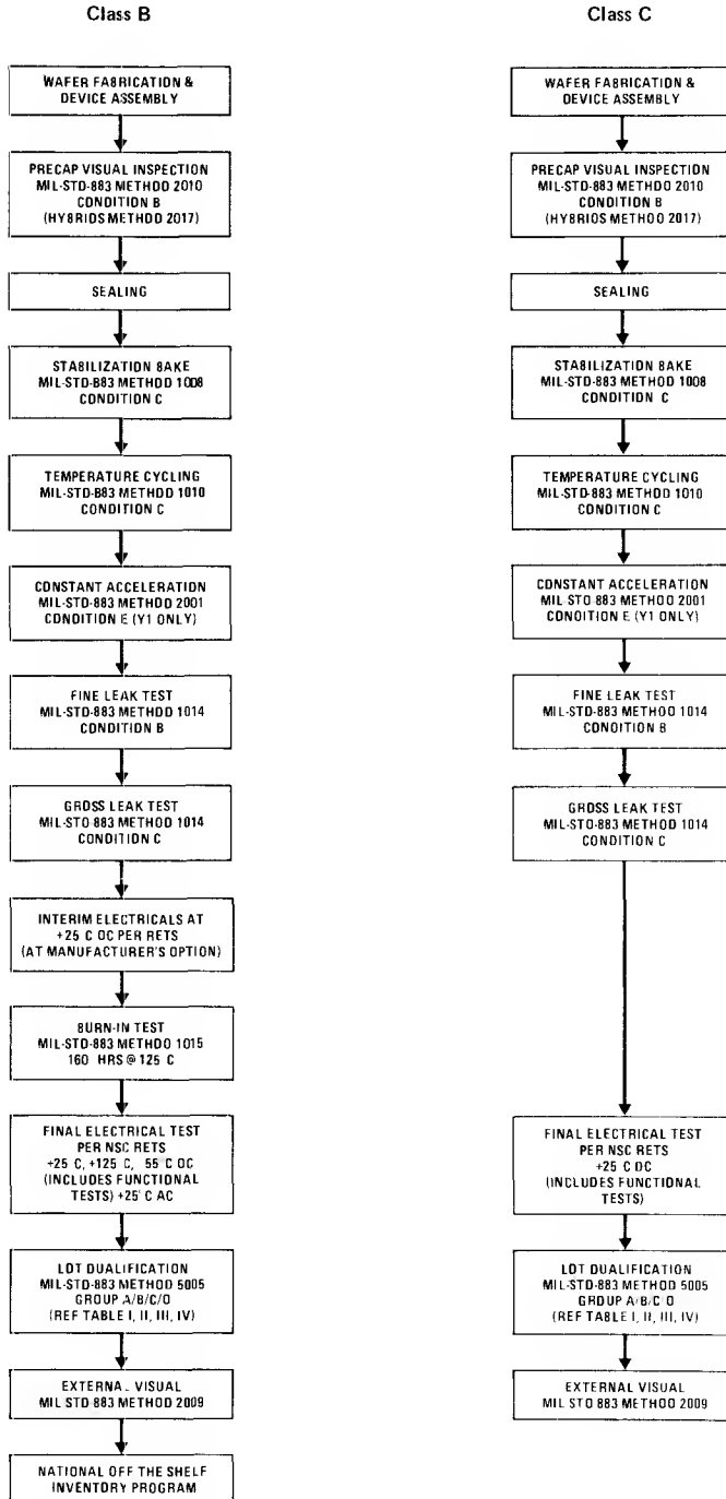
FIGURE 1. MIL-STD-883 Screening
