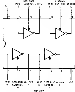
Dual-In-Line Package
