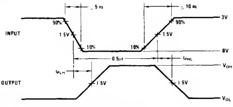
FIGURE 12. Propagation Delay Times, Each Gate (DS55450/DS75450 Only)
