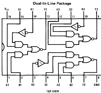
Order Number DS55122J, DS75122J, DS75122N or DS55122W See NS Package J16A, N16A or W16A
