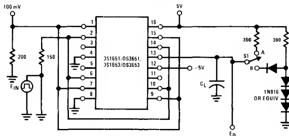
FIGURE 2. Strobe Propagation Delay tPLH(S) and tPHL(S)
