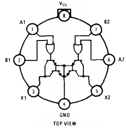
Order Number DS1634H or DS3634H
