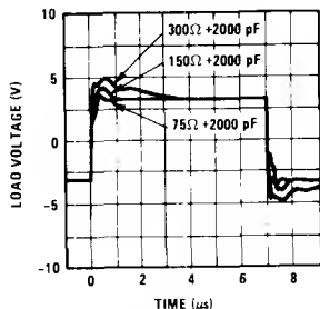
FIGURE 21. Line Response for Various Termination Resistances With a DC Isolation Capacitor
