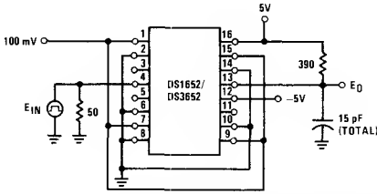
FIGURE 10. Strobe Propagation Delay t_{PLH}(S) and t_{PHL}(S)
