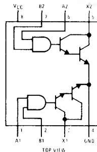
Dual-In-Line Package
