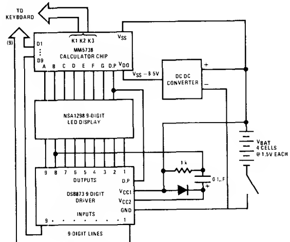
FIGURE 1. 4-Cell System
