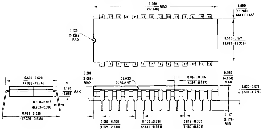
NS Package J28A 28-Lead Cavity DIP (J)
