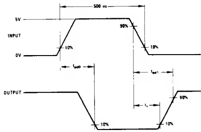
FIGURE 6. Sink-Output Switching Times
