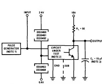
FIGURE 13. Switching Times, Each Transistor (DS55460 and DS75460 Only)
