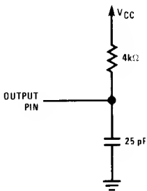
FIGURE 1. Test Load
