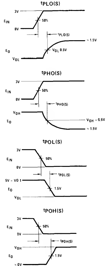
FIGURE 9. Strobe Propagation Delay t_{PLO}(S) , t_{POL}(S) , t_{PHO}(S) and t_{POH}(S)
