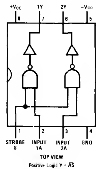
Dual-In-Line Package
