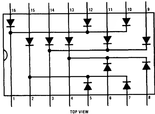
Order Number DS8656N See NS Package N16A
