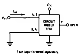
FIGURE 2. I_{IH} , I_{IL}
