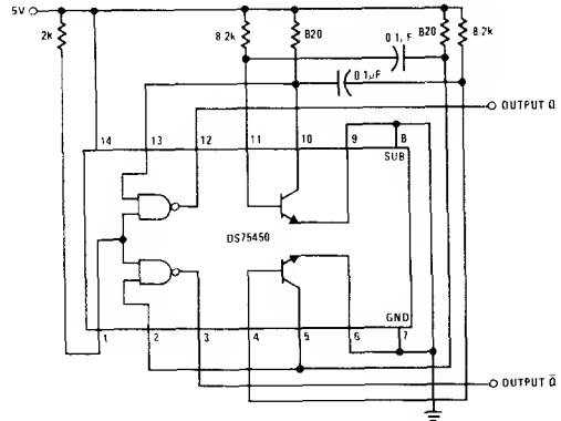
FIGURE 23. Square-Wave Generator
