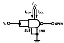
FIGURE 6. I_{CCH} , I_{CCL}
