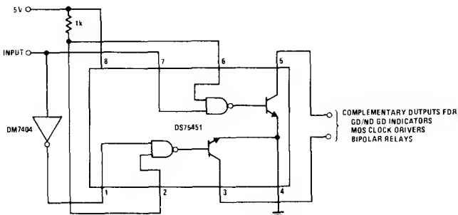
FIGURE 29. Complementary Driver
