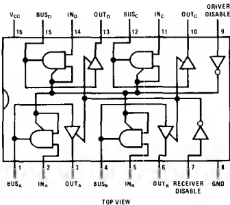
Dual-In-Line Package
