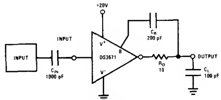
Typical Bootstrap
