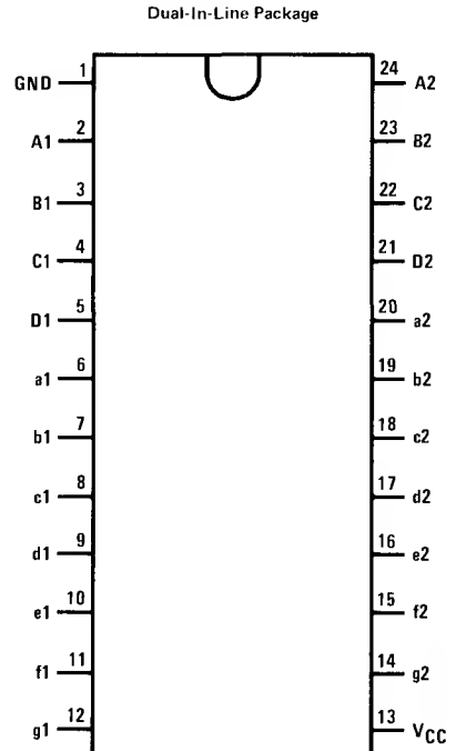
TDP VIEW
