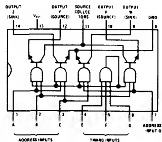
Dual-In-Line Package
