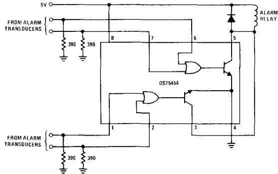
FIGURE 35. Alarm Detector
