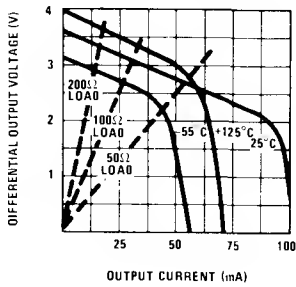
Differential Output Voltage (V NAND - V NAND ) Vs Differential Output Current
