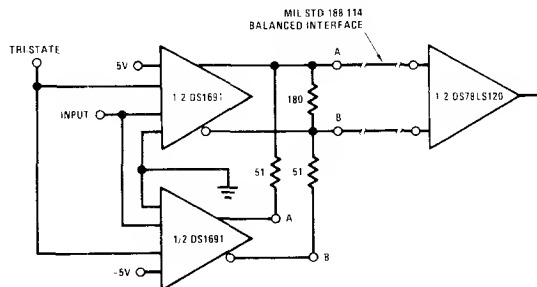
FIGURE 5. MIL-STD-188-114 (Balanced) Application
