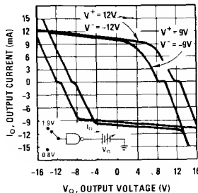
Output Voltage and Current-Limiting Characteristics
