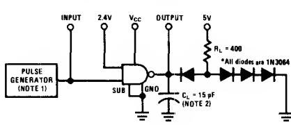
FIGURE 12. Propagation Delay Times, Each Gate (DS55460 and DS75460 Only)
