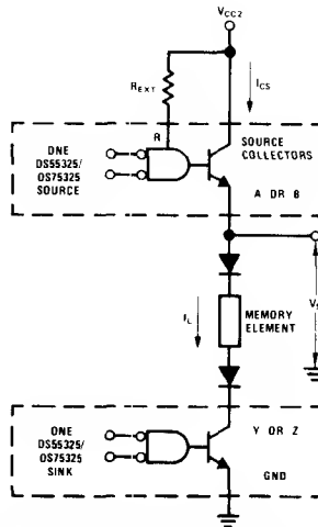
Note 1: For clarity, partial logic diagrams of two DS55325's are shown. Note 2: Source and sink shown are in different packages
