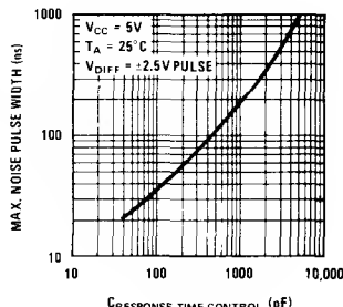
Noise Rejection
