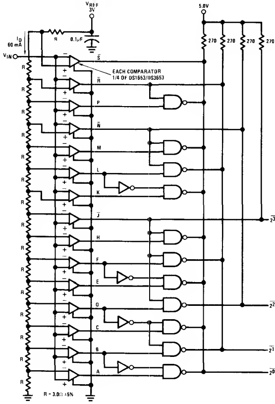
4-Bit Parallel A/D Converter
