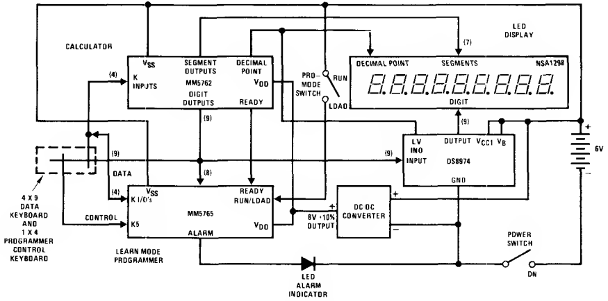
FIGURE 1. 6V Programmable Statistical Calculator
