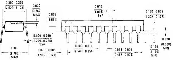
NS Package N20A 20-Lead Molded DIP (N)
