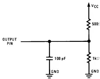
FIGURE 2. Test Load
