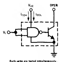
FIGURE 10. I_{OCH} , I_{OCL} for AND, NAND Circuits
