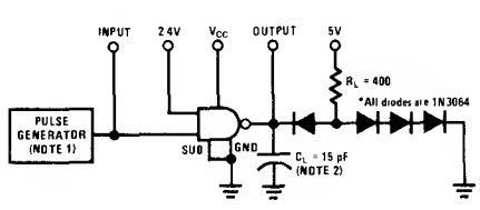
FIGURE 12. Propagation Delay Times, Each Gate (DS55450/DS75450 Only)
