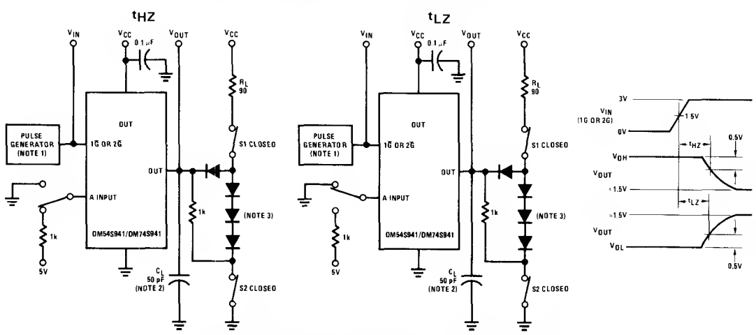
FIGURE 9. Propagation Delay to TRI-STATE from High or Low Level
