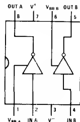
Dual-In-Line Package
