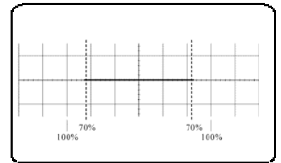
Fig. 1.10 Measuring the Trace Length at the 3 dB Point Frequency
