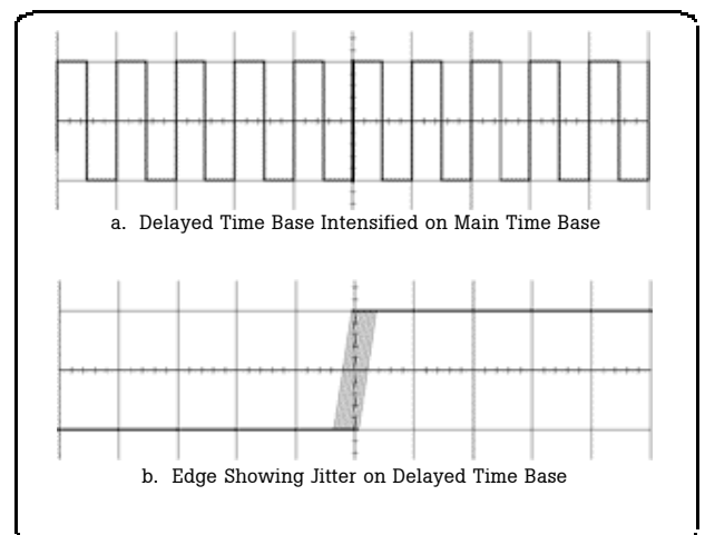
Fig. 1.15 Measuring the Delay Time Jitter
