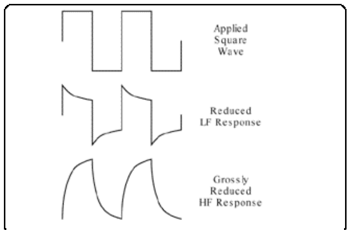
Fig. 1.4 LF Square Wave - Distortions
