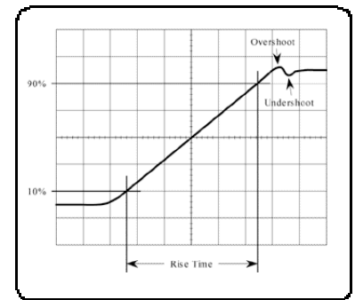
Fig. 1.5 Measurement of Rise Time
