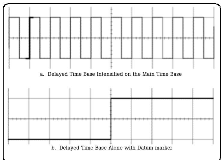
Fig. 1.12 Adjusting the Delayed Time Base to the First Datum Marker
