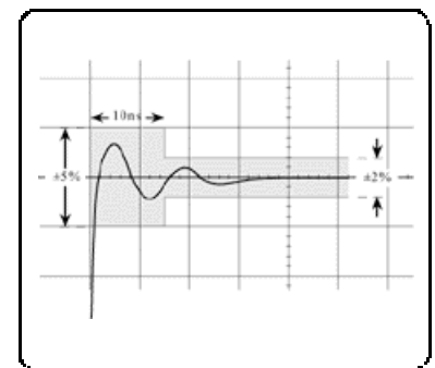
Fig. 1.6 Leading Edge Aberration
