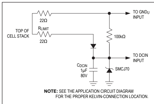
Figure 24. DCIN Overvoltage Protection and Decoupling Circuit
