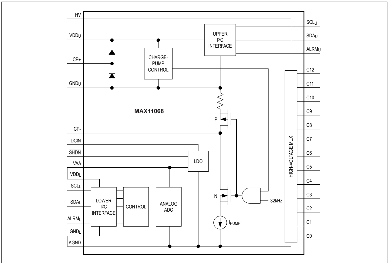
Figure 23. Detailed View of Supply and Ground Connections
