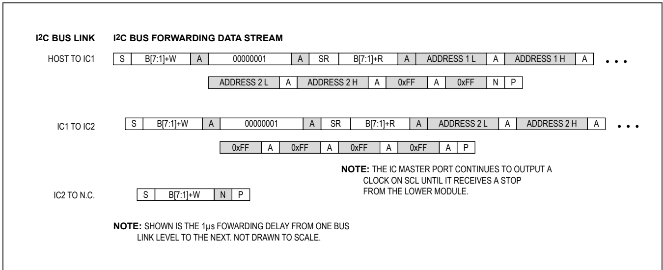
Figure 32. ROLLCALL Command SMBus Ladder Sequences with Two Modules
