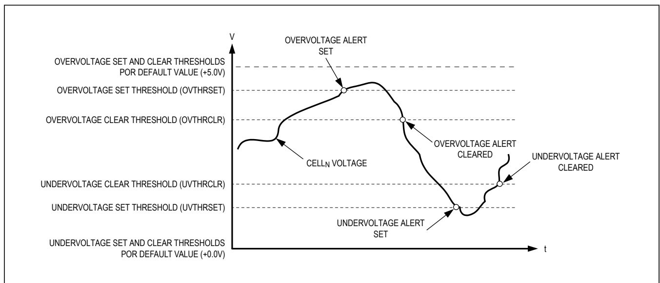
Figure 12. Programmable Overvoltage and Undervoltage Thresholds Diagram
