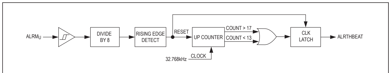
Figure 44. ALRM U Pin and ALRTHBEAT Block Diagram
