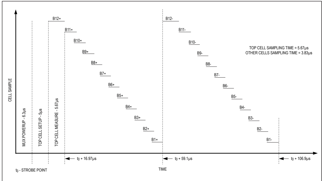
Figure 10. Cell-Scanning Timing
