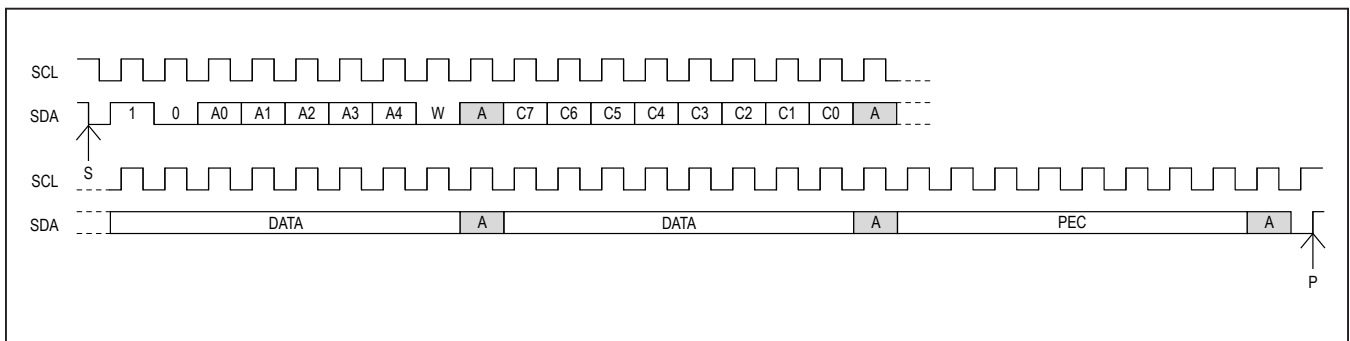
Figure 33. I 2 C Communication Sequence for the SETLASTADDRESS Command
