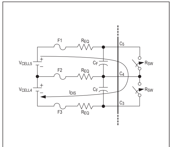
Figure 14. Discharge Current Path for Adjacent Enabled Balancing Switches
