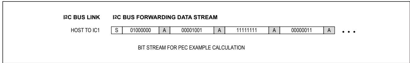
Figure 43. Example WRITEALL Bit Stream Prior to PEC Transmission
