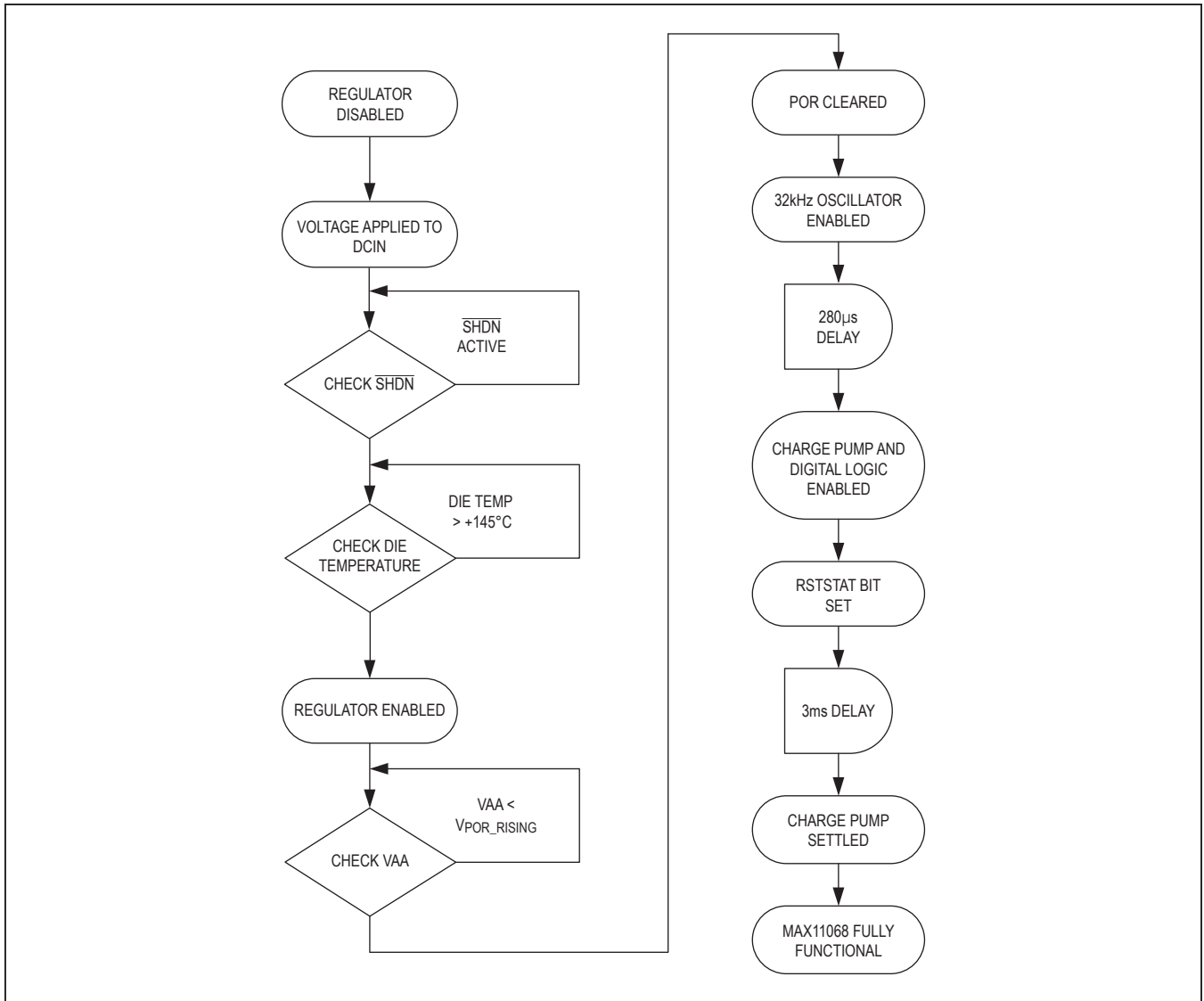
Figure 20. Power-Up Sequence
