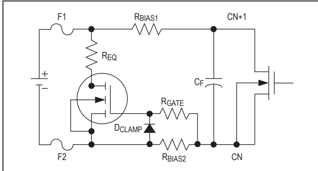
Figure 17. External Cell-Balancing Circuit with a MOSFET Transistor
