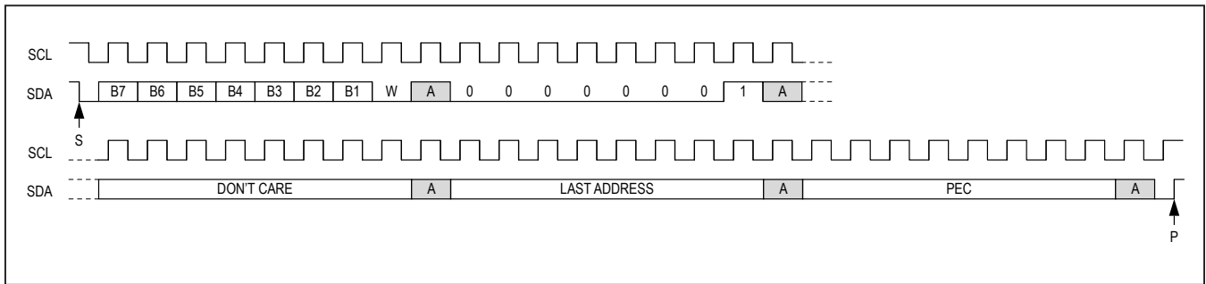
Figure 37. I 2 C Communication Sequence for the WRITEDEVICE Command
