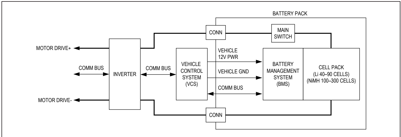
Figure 7. Electric Vehicle System
