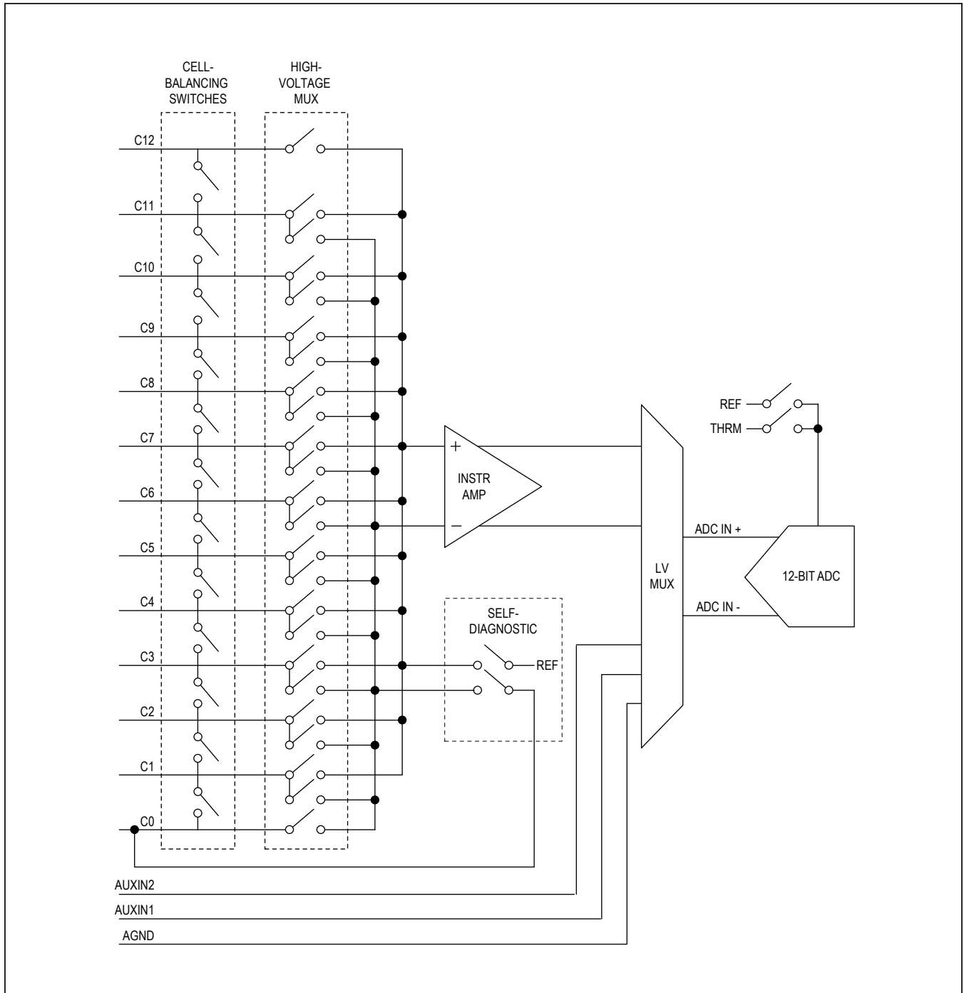
Figure 2. Analog Front-End Block Diagram
