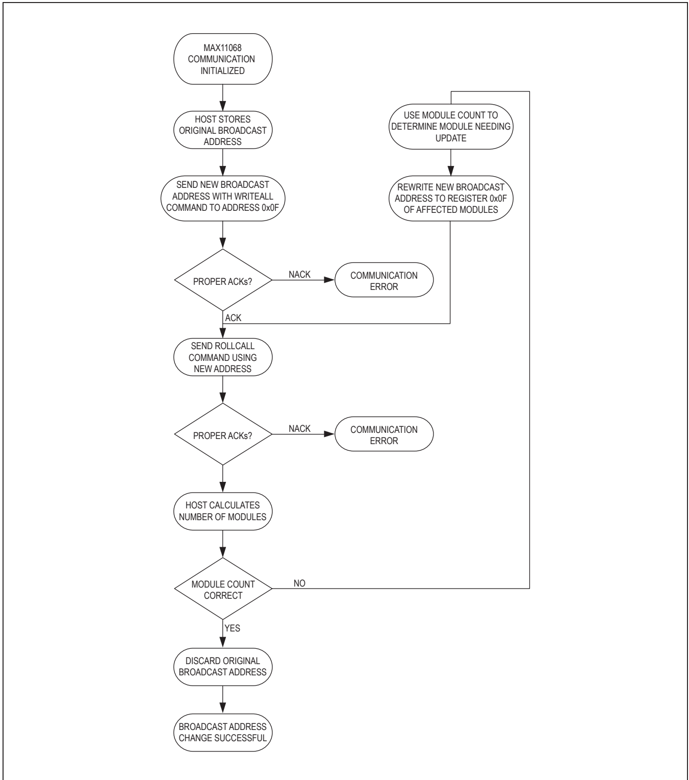
Figure 48. Broadcast Address Change Procedure
