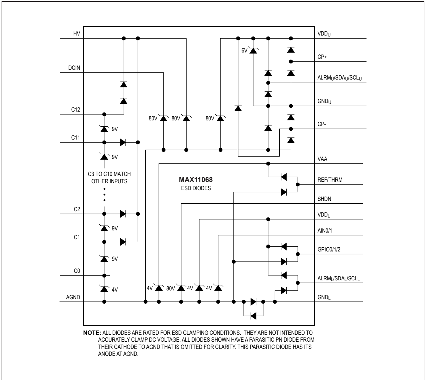
Figure 3. MAX11068 ESD Diode Diagram
