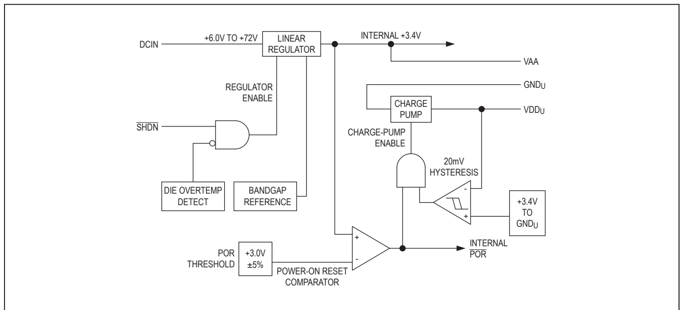
Figure 19. Internal Low-Dropout Regulator Block Diagram
