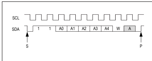
Figure 29. I 2 C Address Byte for the HELLOALL Command
