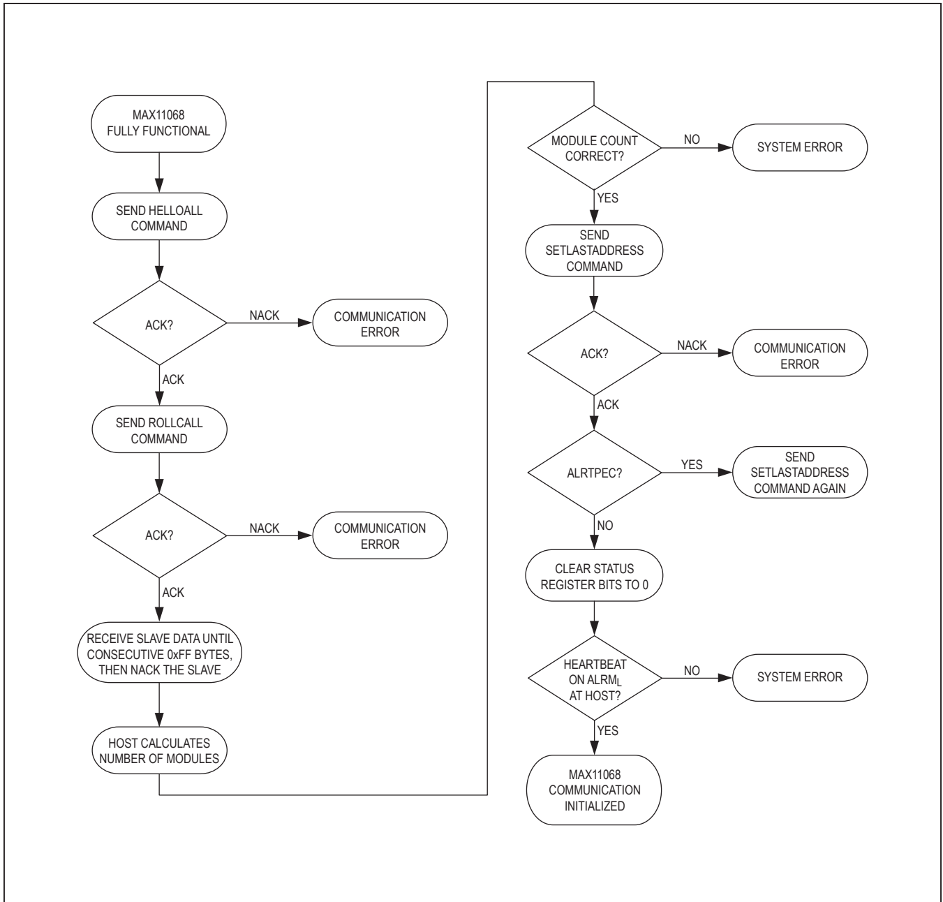
Figure 47. Communication Initialization Sequence Following Any Reset Event or Module Connection Change
