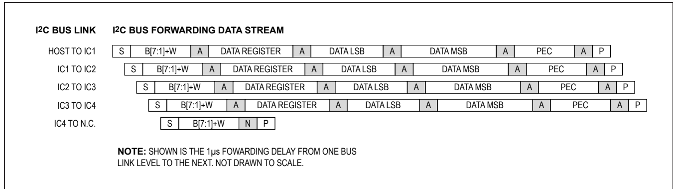
Figure 34. SETLASTADDRESS Command SMBus Ladder Sequences with Four Modules
