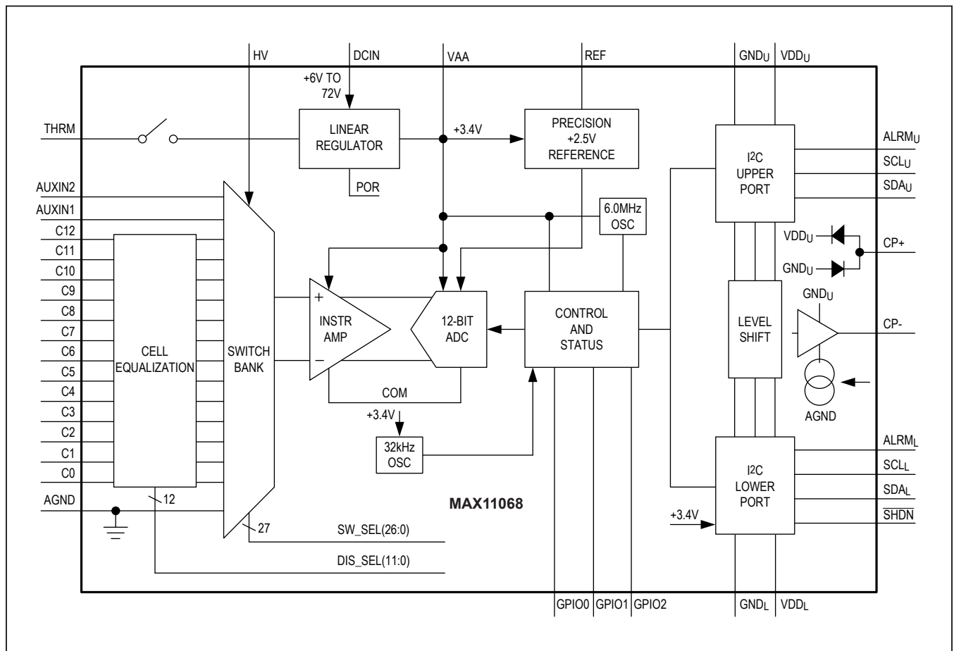
Figure 1. Functional Diagram
