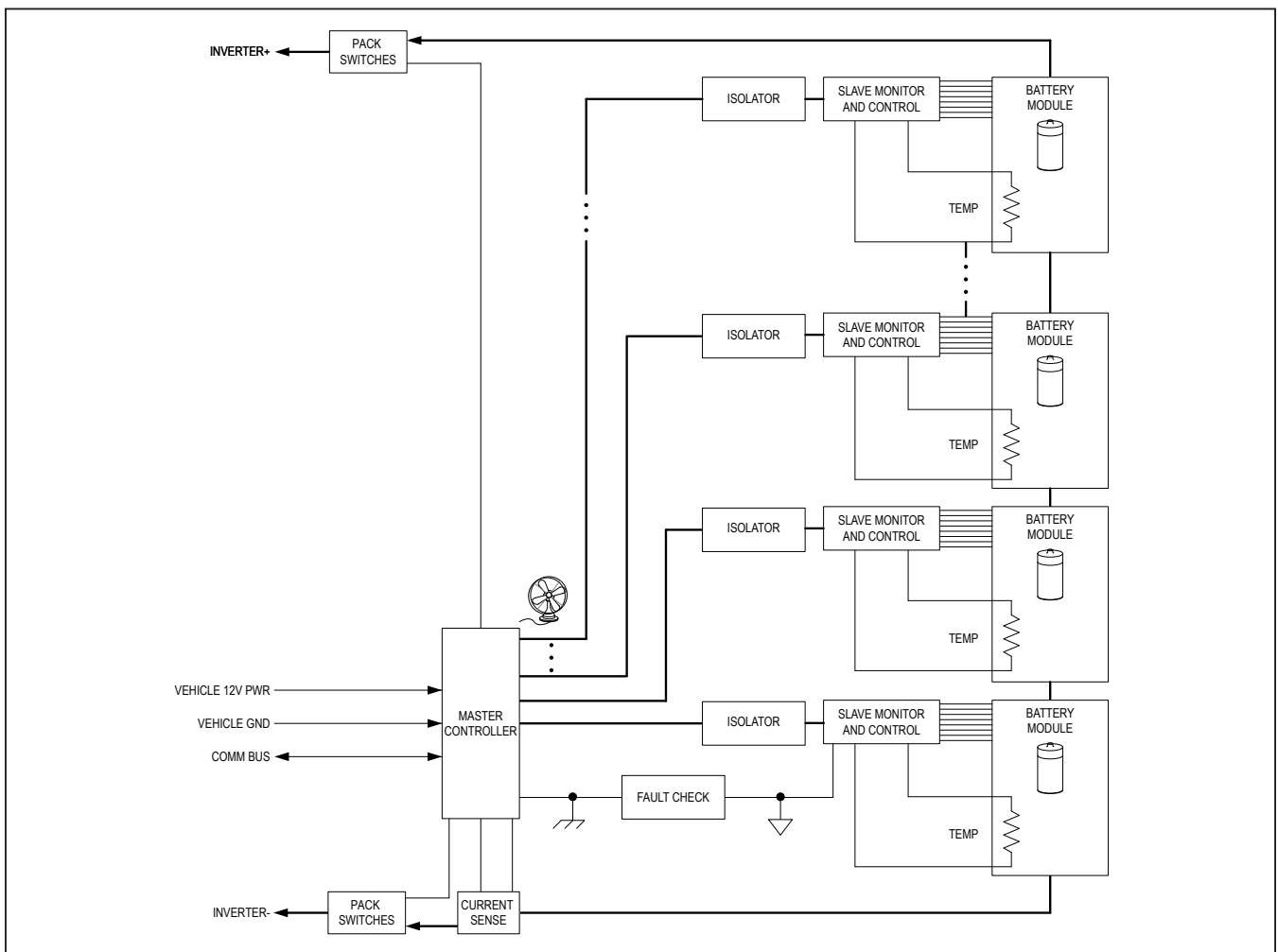
Figure 8. Distributed Communication Battery Pack
