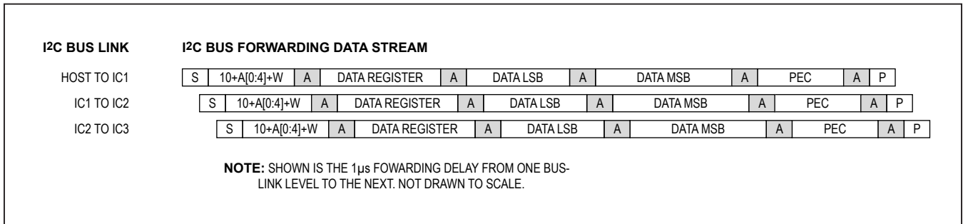
Figure 38. WRITEDEVICE Command SMBus Ladder Sequences Where the Device Address Matches IC3
