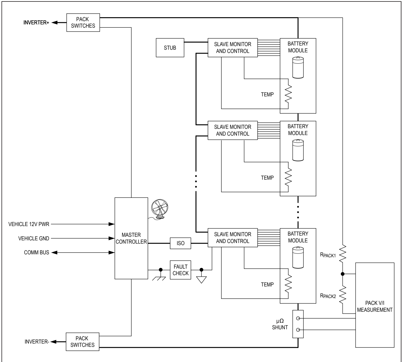
Figure 9. SMBus-Laddered Battery Module Communication
