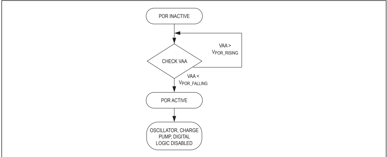
Figure 22. Power-On-Reset Event Sequence
