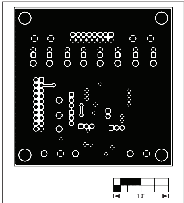
Figure 27. MAX11614 EV Kit Daughter Board PCB Layout—Bottom
