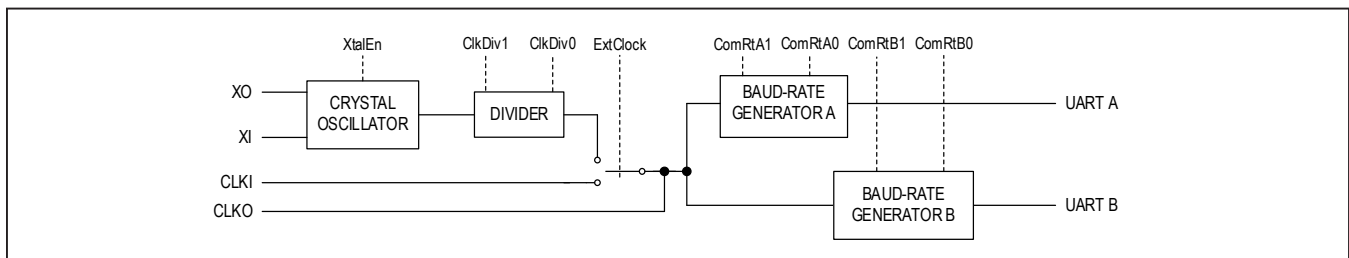
Figure 15. Clock Generation
