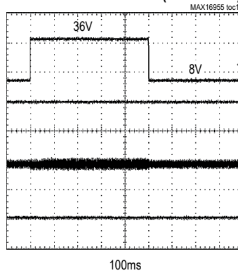
LOAD DUMP RESPONSE (SKIP MODE)
