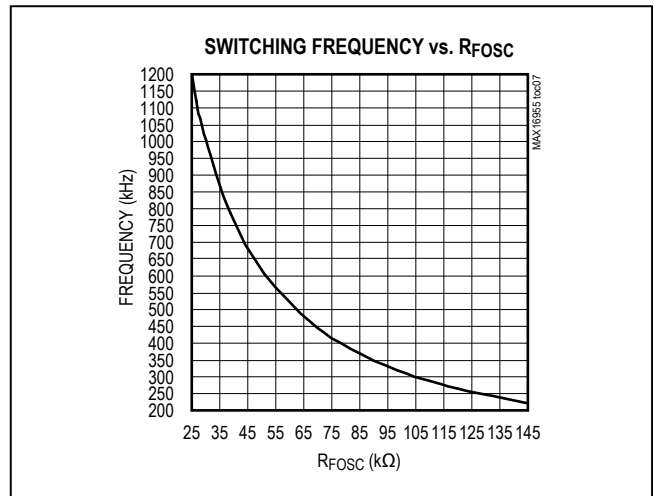
Figure 3. Switching Frequency vs. R FOSC
