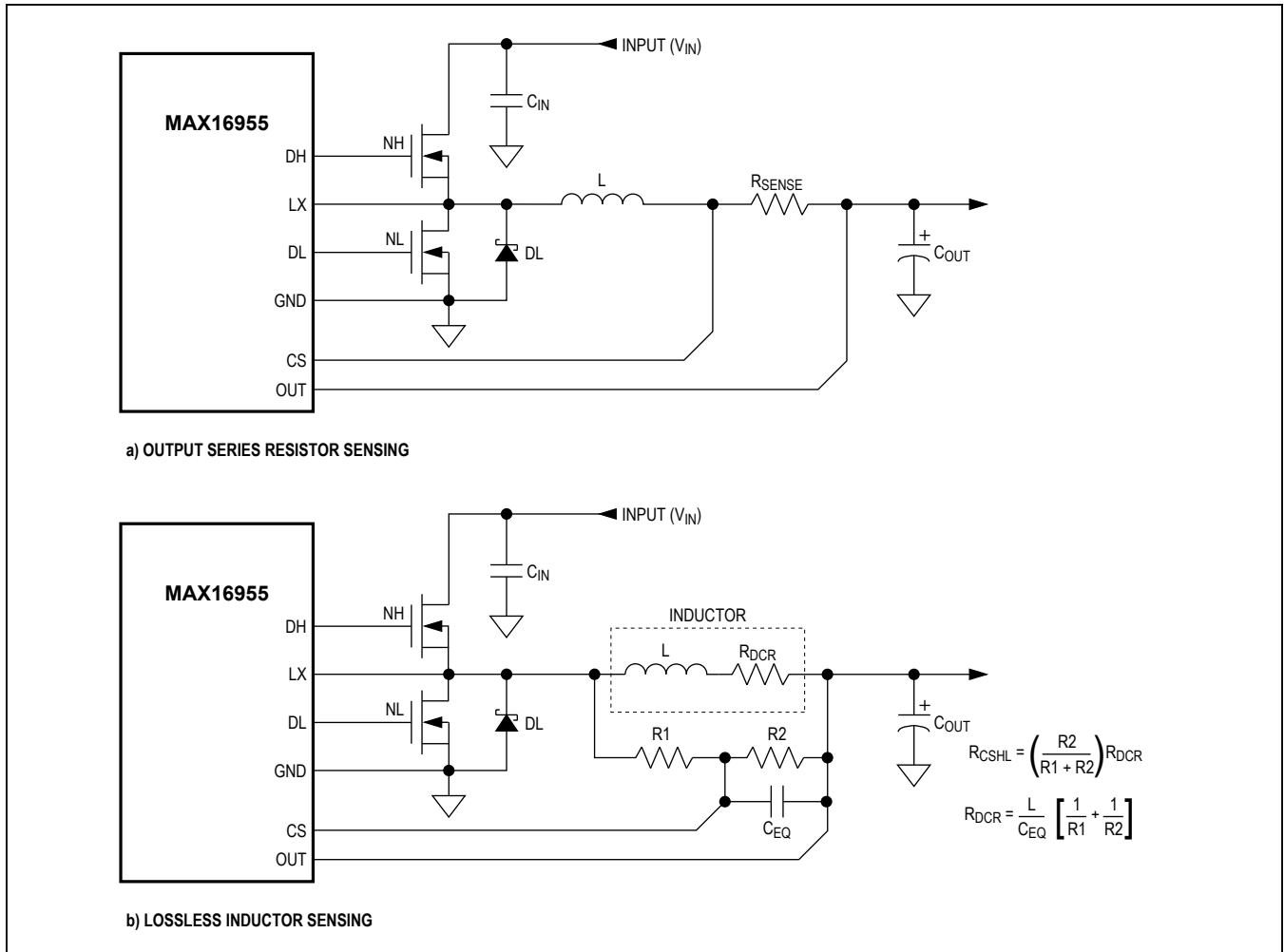
Figure 4. Current-Sense Configurations
