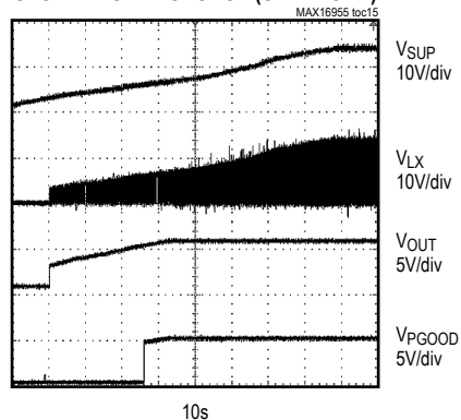
SLOW INPUT RESPONSE (SKIP MODE)
