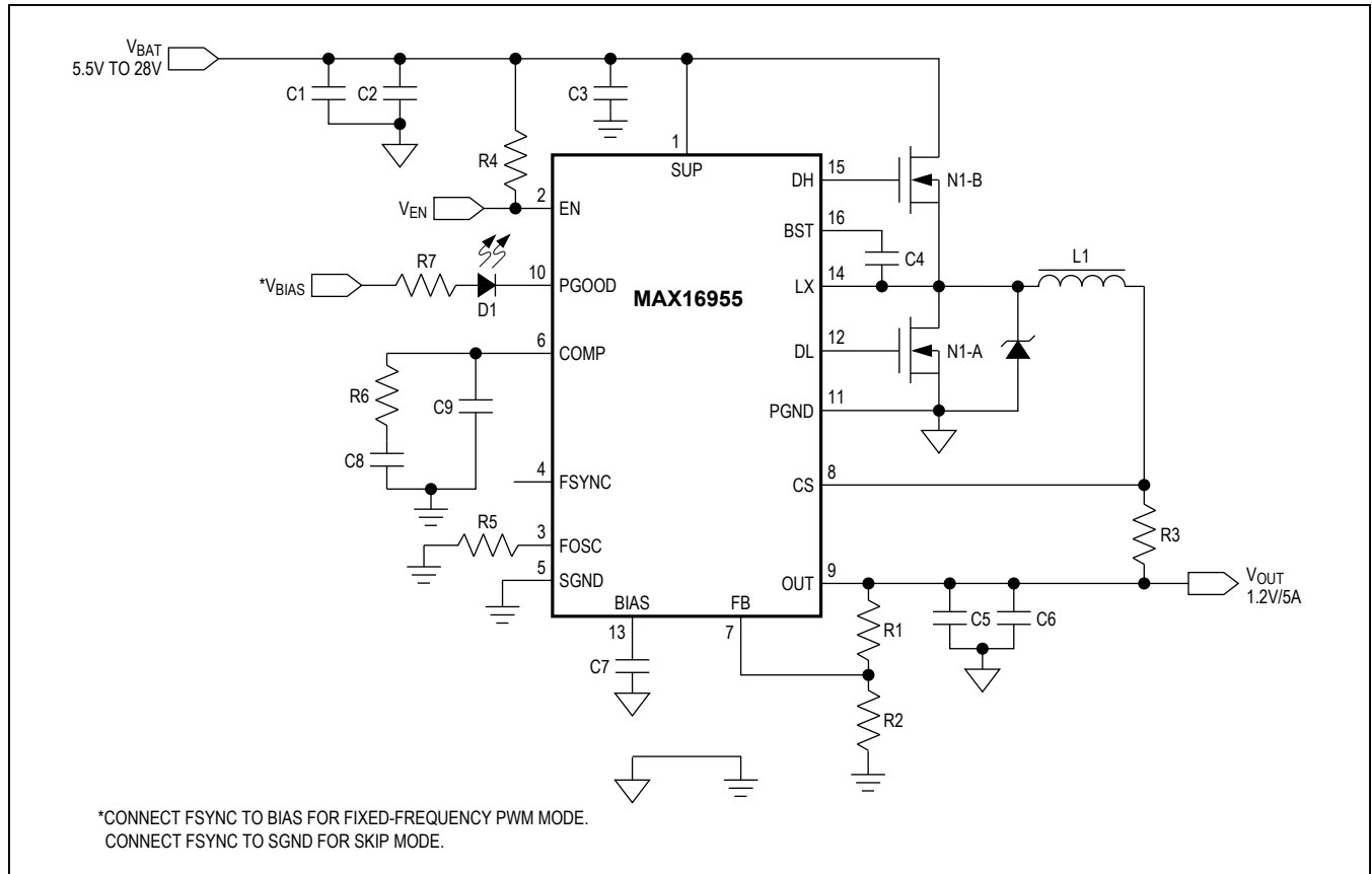
Figure 7. Typical Operating Circuit for Adjustable Output Voltage, V_{OUT} = 1.2V/5A
