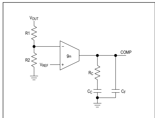
Figure 5. Compensation Network
