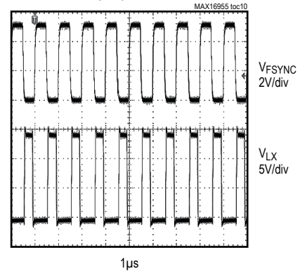
SYNCHRONIZATION WITH EXTERNAL CLOCK f_{SYNC} = 1MHz
