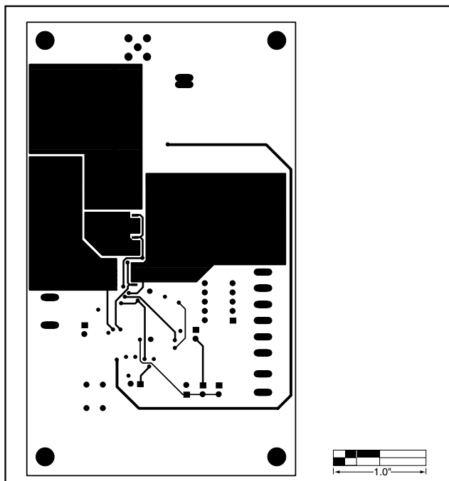
Figure 5. MAX1855 EV Kit PC Board Layout—Solder Side
