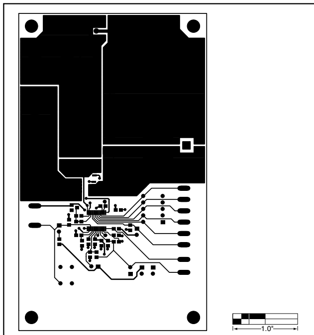
Figure 3. MAX1855 EV Kit PC Board Layout—Component Side
