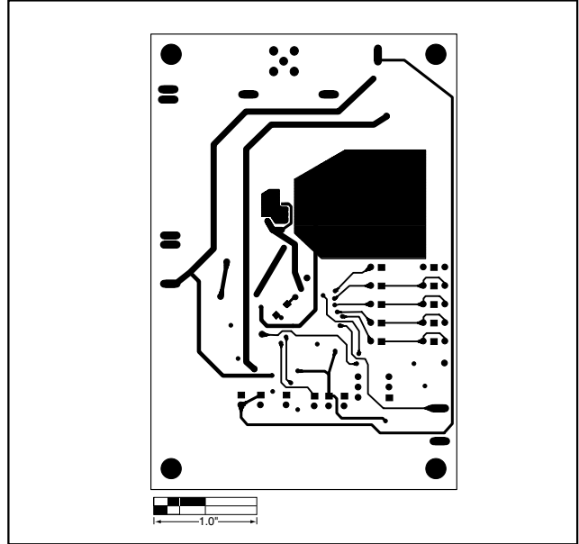
Figure 7. MAX1717 EV Kit PC Board Layout—Solder Side
