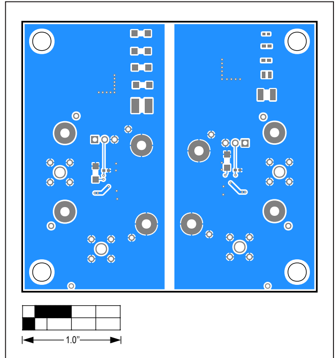
MAX17225 EV Kit—Bottom
