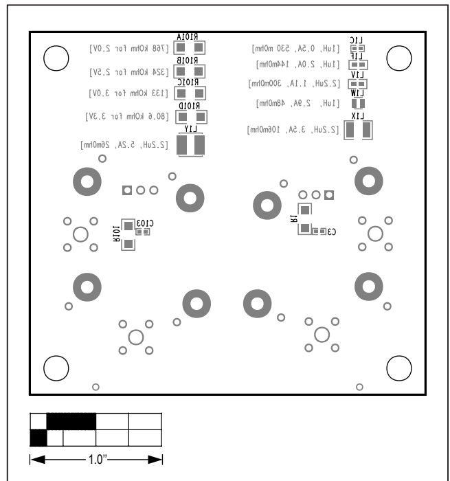
MAX17225 EV Kit—Bottom Silkscreen
