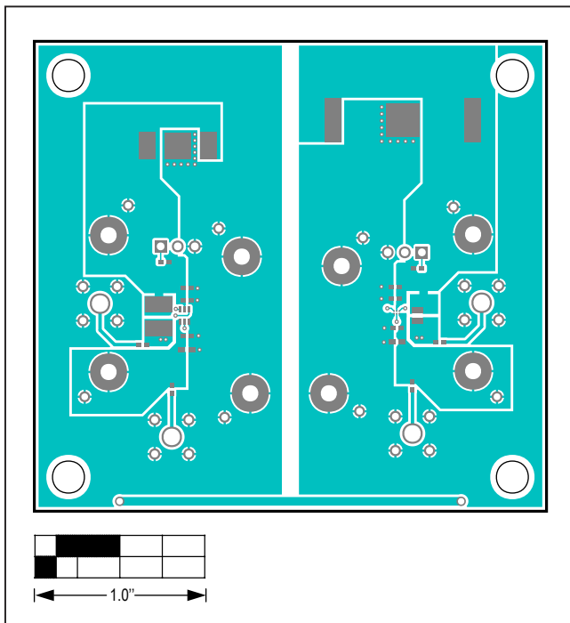
MAX17225 EV Kit—Top
