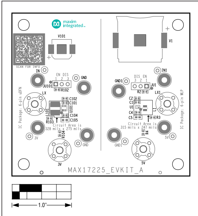
MAX17225 EV Kit—Top Silkscreen
