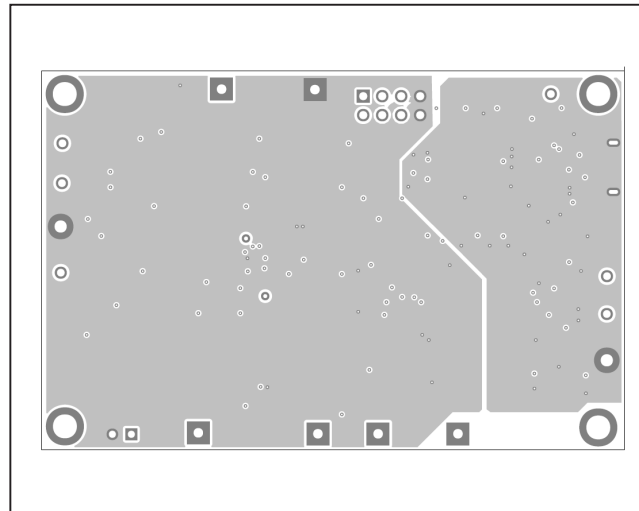
MAX173x0G EV Kit Layout—Layer 2
