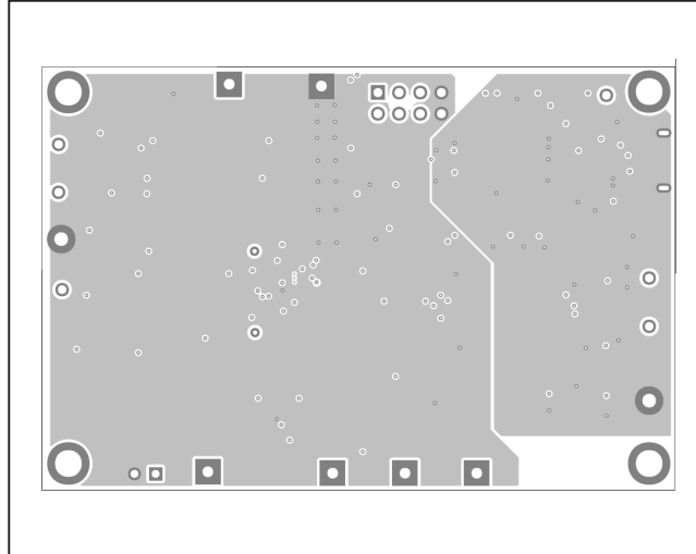
MAX173x0X EV Kit Layout—Layer 2
