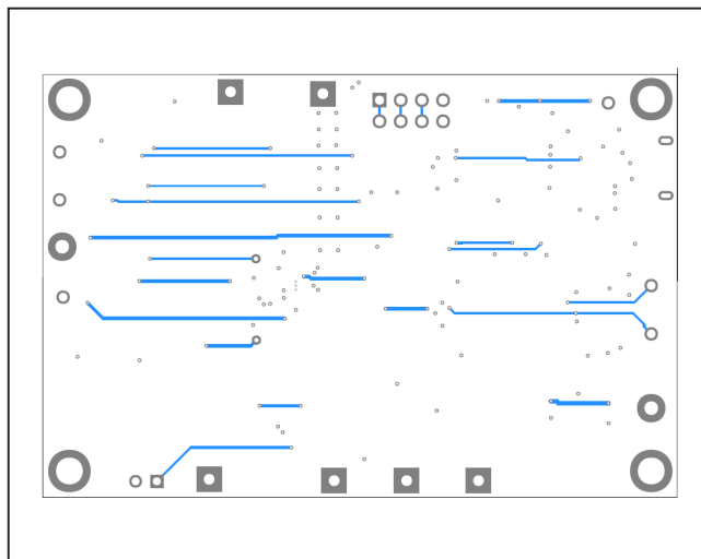
MAX173x0X EV Kit Layout—Bottom Layer
