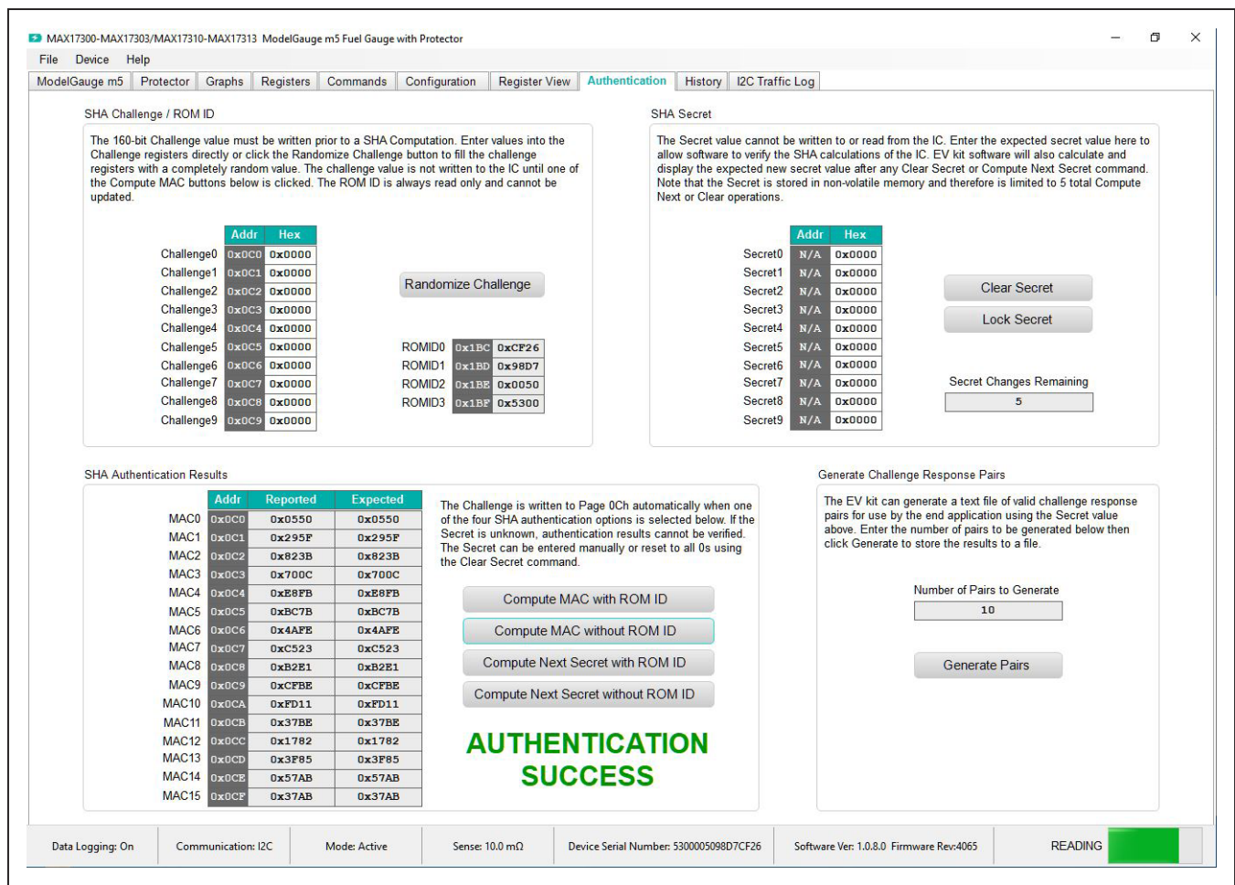
Figure 11. Authentication Tab
