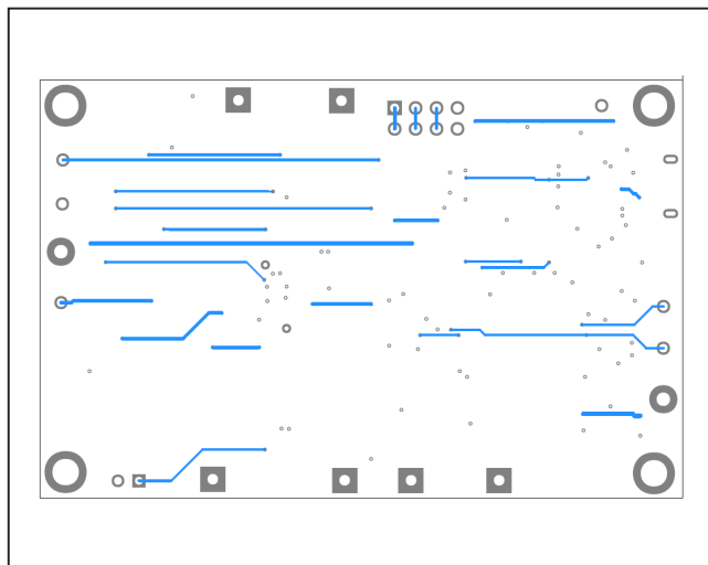
MAX173x0G EV Kit Layout—Bottom Layer
