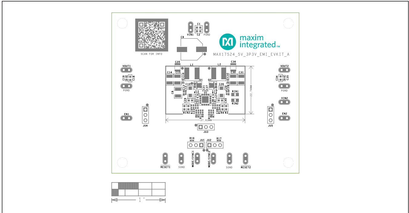
MAX17524EVKITE# PCB—Top Silkscreen
