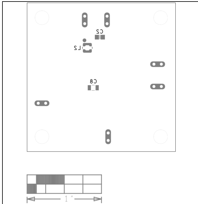
MAX17553A EV Kit PCB Layout—Bottom Silkscreen
