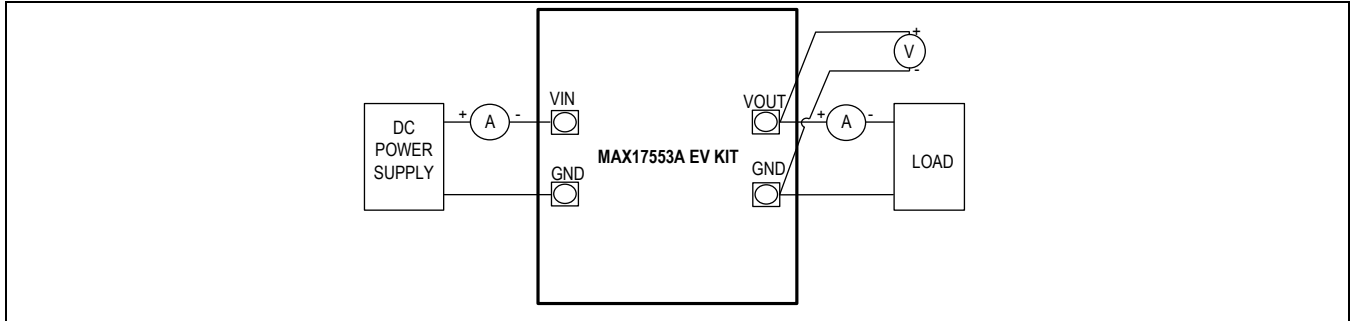
Figure 1. MAX17553A EV Kit Setup Diagram
