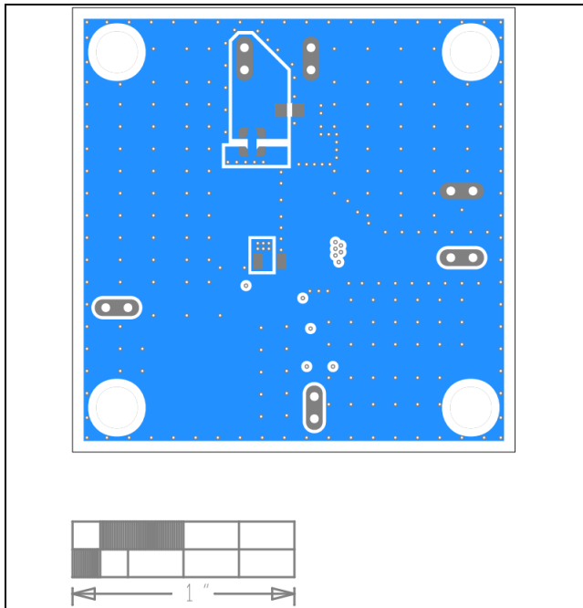
MAX17553A EV Kit PCB Layout—Bottom Layer
