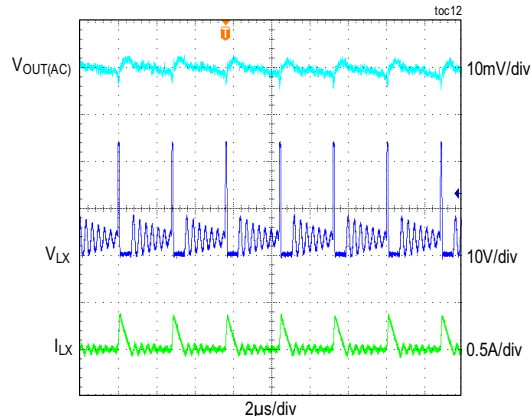
CONDITIONS: DCM MODE, 40mA LOAD
