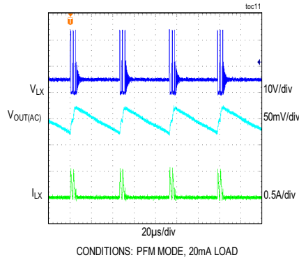
STEADY-STATE PERFORMANCE
