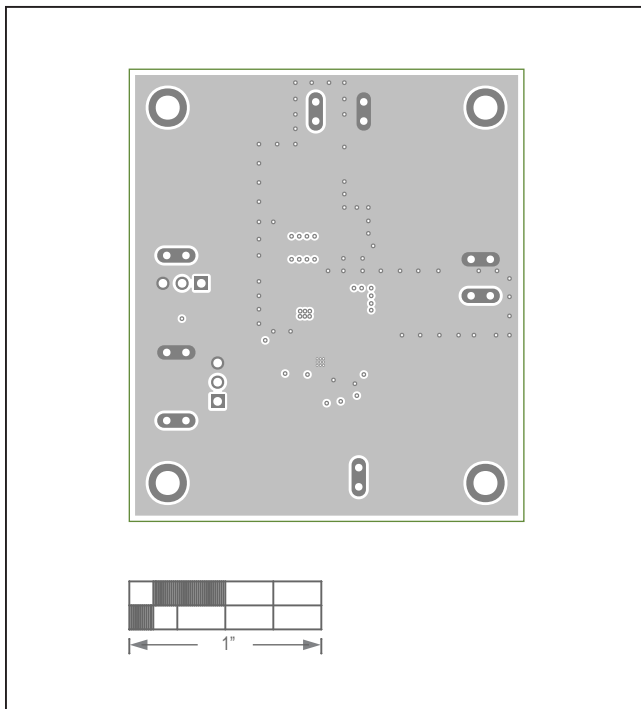
MAX17631BEVKIT# EV Kit—Layer 2
