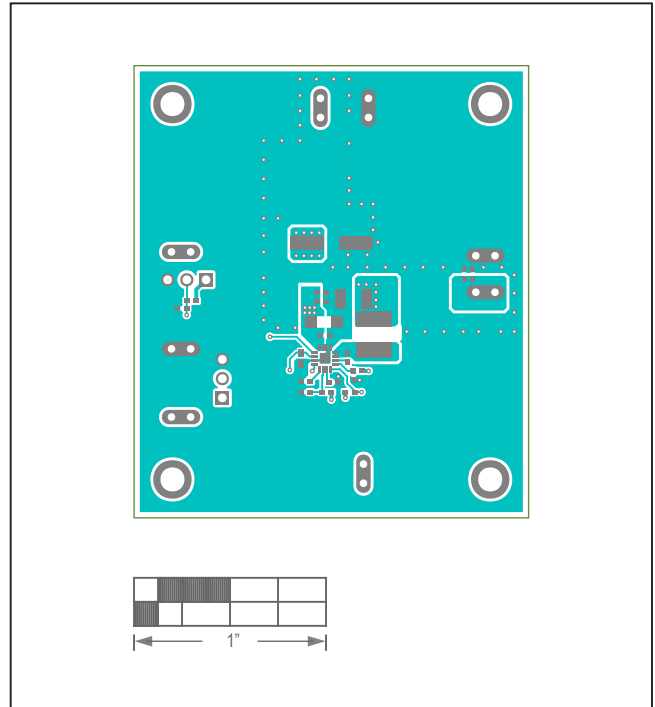
MAX17631BEVKIT# EV Kit—Top Layer
