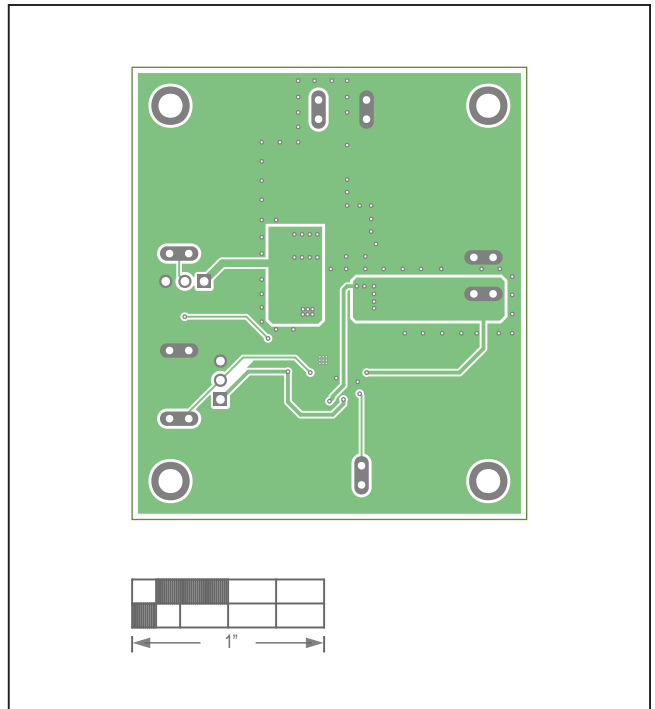
MAX17631BEVKIT# EV Kit—Layer 3
