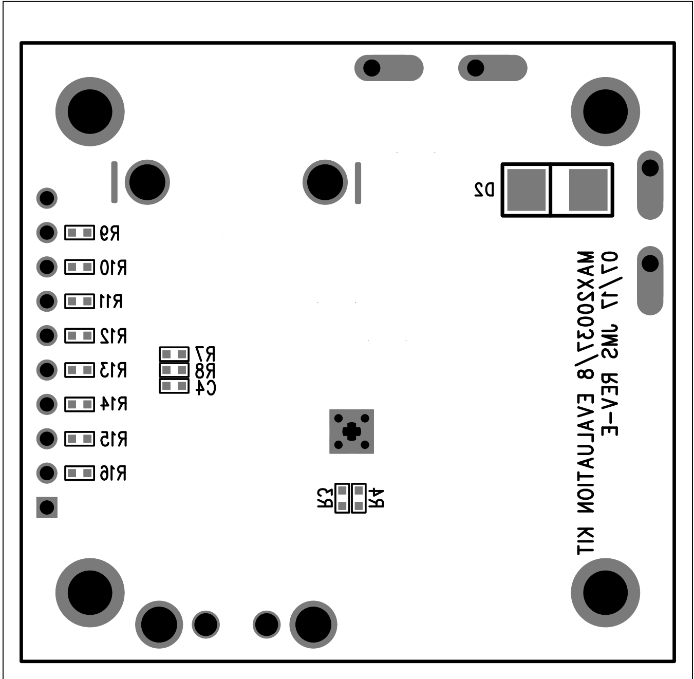
MAX20038 EV Kit PCB Layout—Bottom Silkscreen
