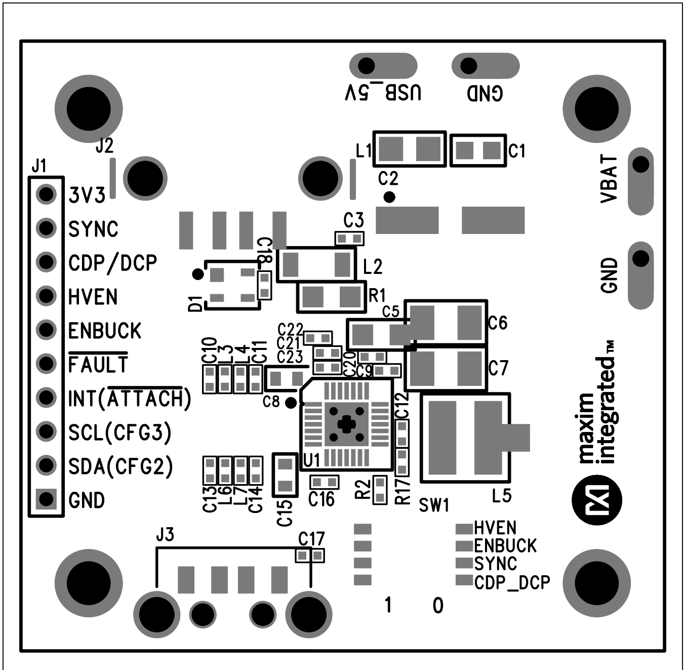
MAX20038 EV Kit PCB Layout—Top Silkscreen
