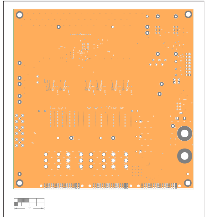
MAX20754 EV Kit--Internal Layer 5 GND
