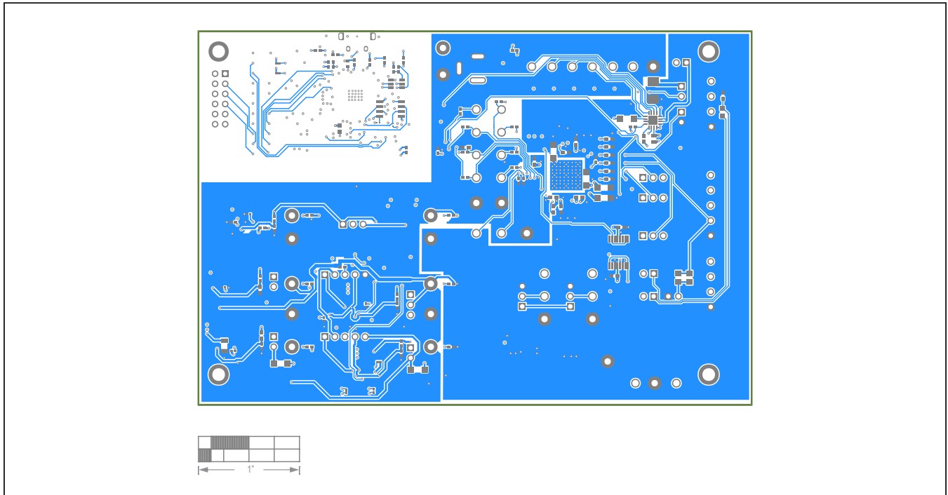
MAX22000 EV Kit—Bottom Layer
