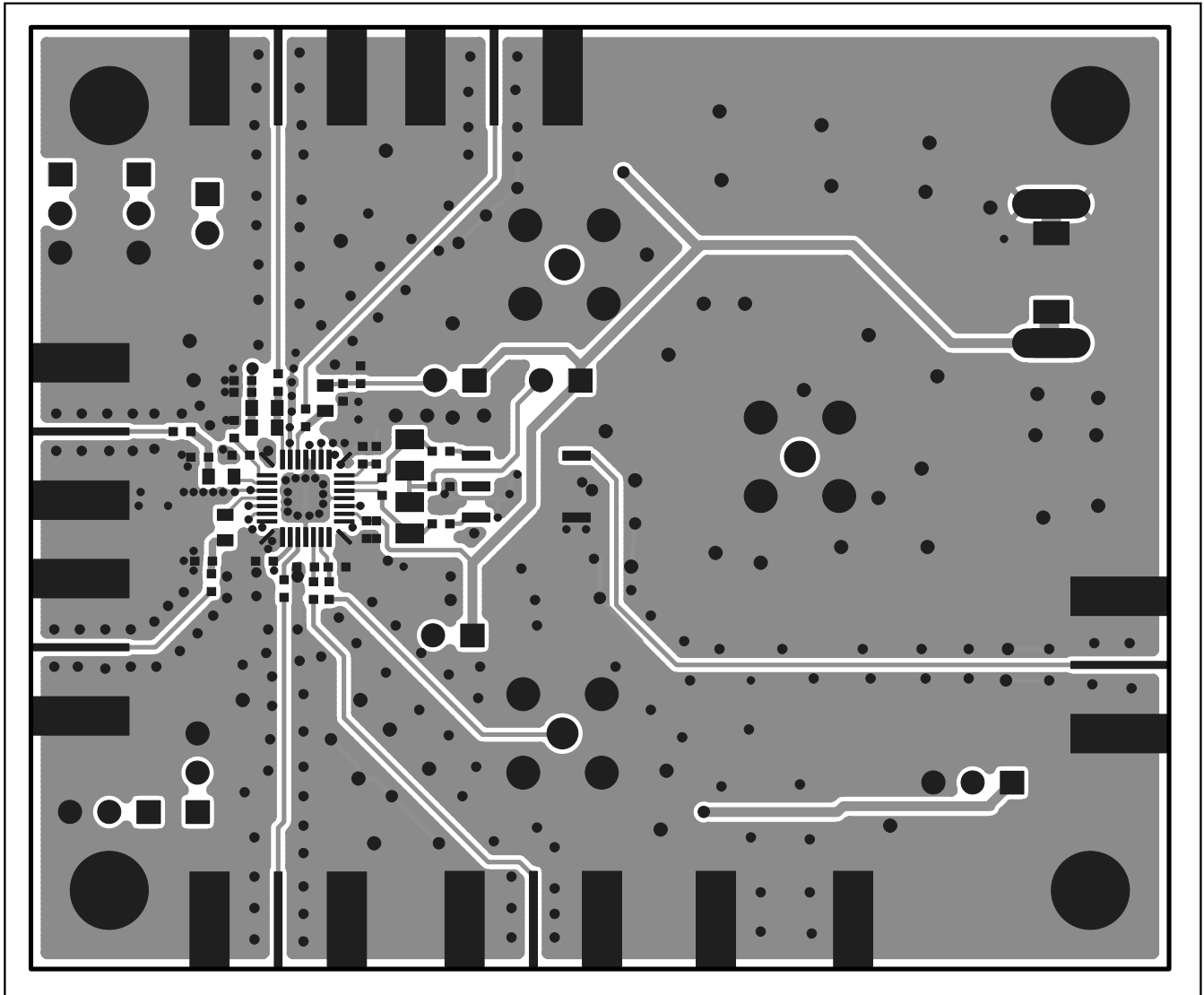
Figure 2. MAX2335 EV Kit PC Board Layout—Front Side
