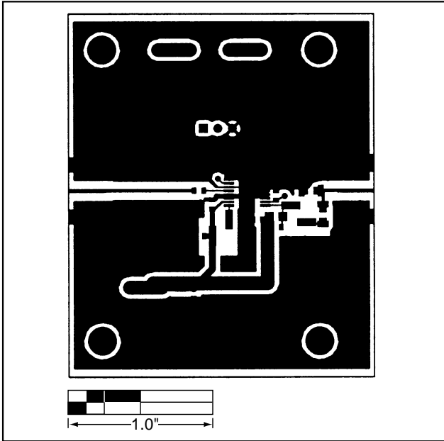
Figure 8. MAX2430 EV Kit-PwrQSOP PC Board Layout—Component Side
