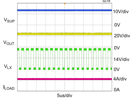
SWITCHING WAVEFORM
