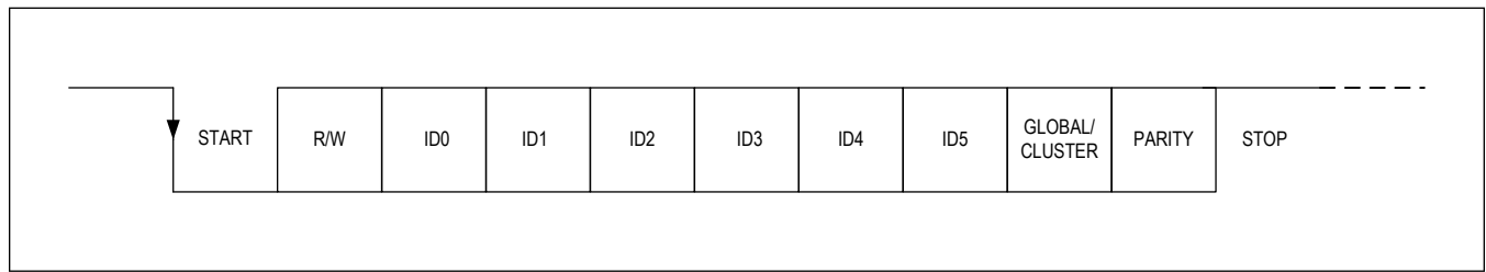
Figure 12. Device ID and Address Frame
