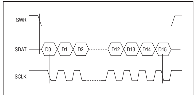
Figure 3. Reading Mode Register Timing Diagram
