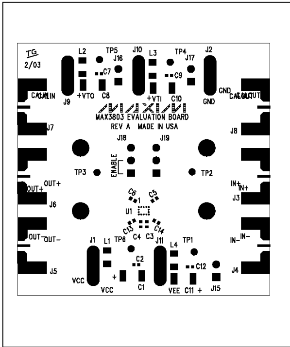
Figure 2. MAX3803 Component Placement Guide
