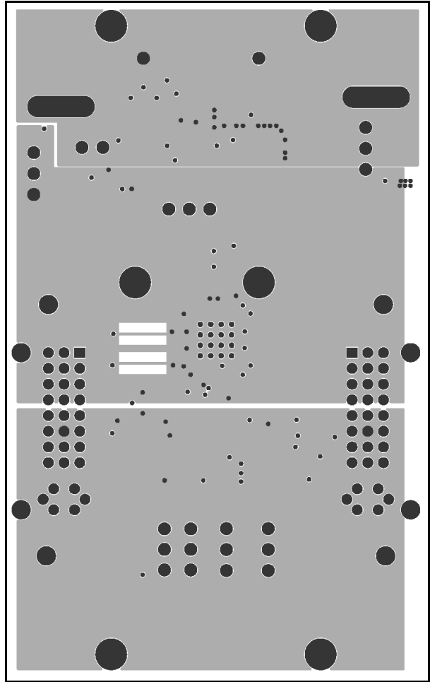
Figure 5. MAX3815 EV Kit PC Board Layout—Power Plane
