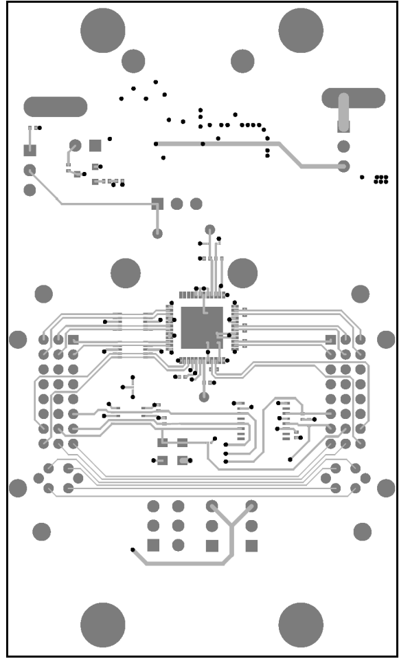
Figure 3. MAX3815 EV Kit PC Board Layout—Top Side
