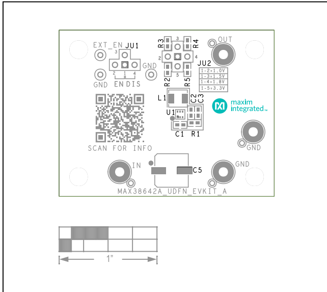
MAX38642A \mu DFN EV Kit—Top Silkscreen
