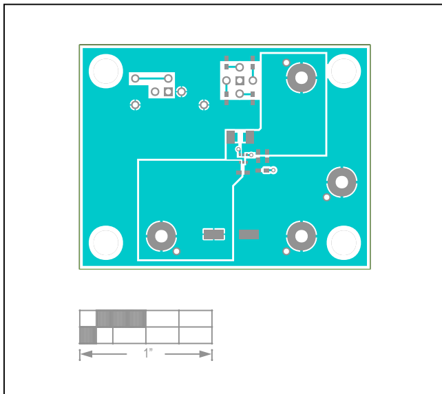
MAX38642A \mu DFN EV Kit—Top
