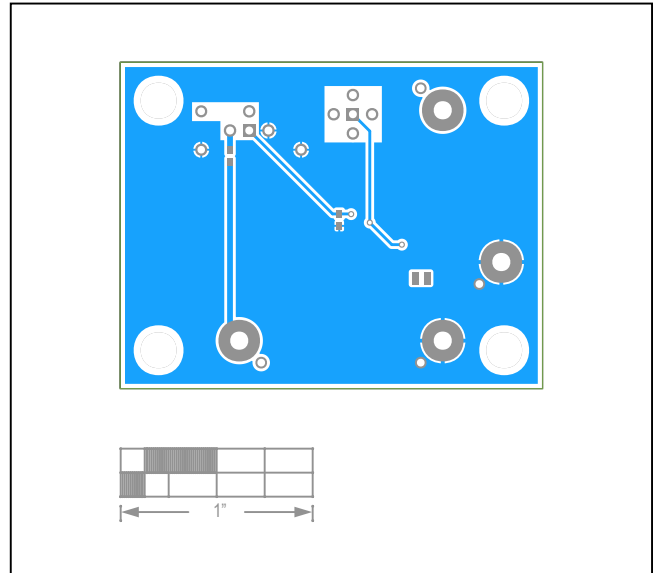
MAX38642A \mu DFN EV Kit—Bottom
