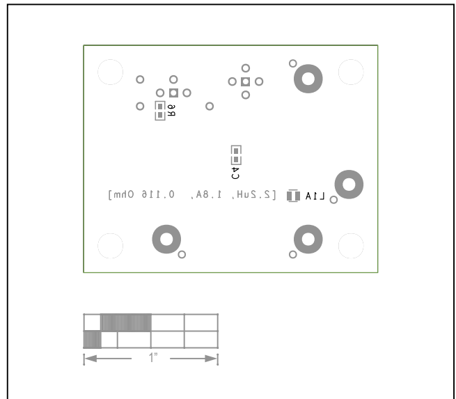
MAX38642A \mu DFN EV Kit—Bottom Silkscreen
