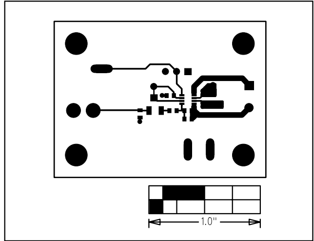
Figure 3. MAX4366 EV Kit PC Board Layout—Component Side
