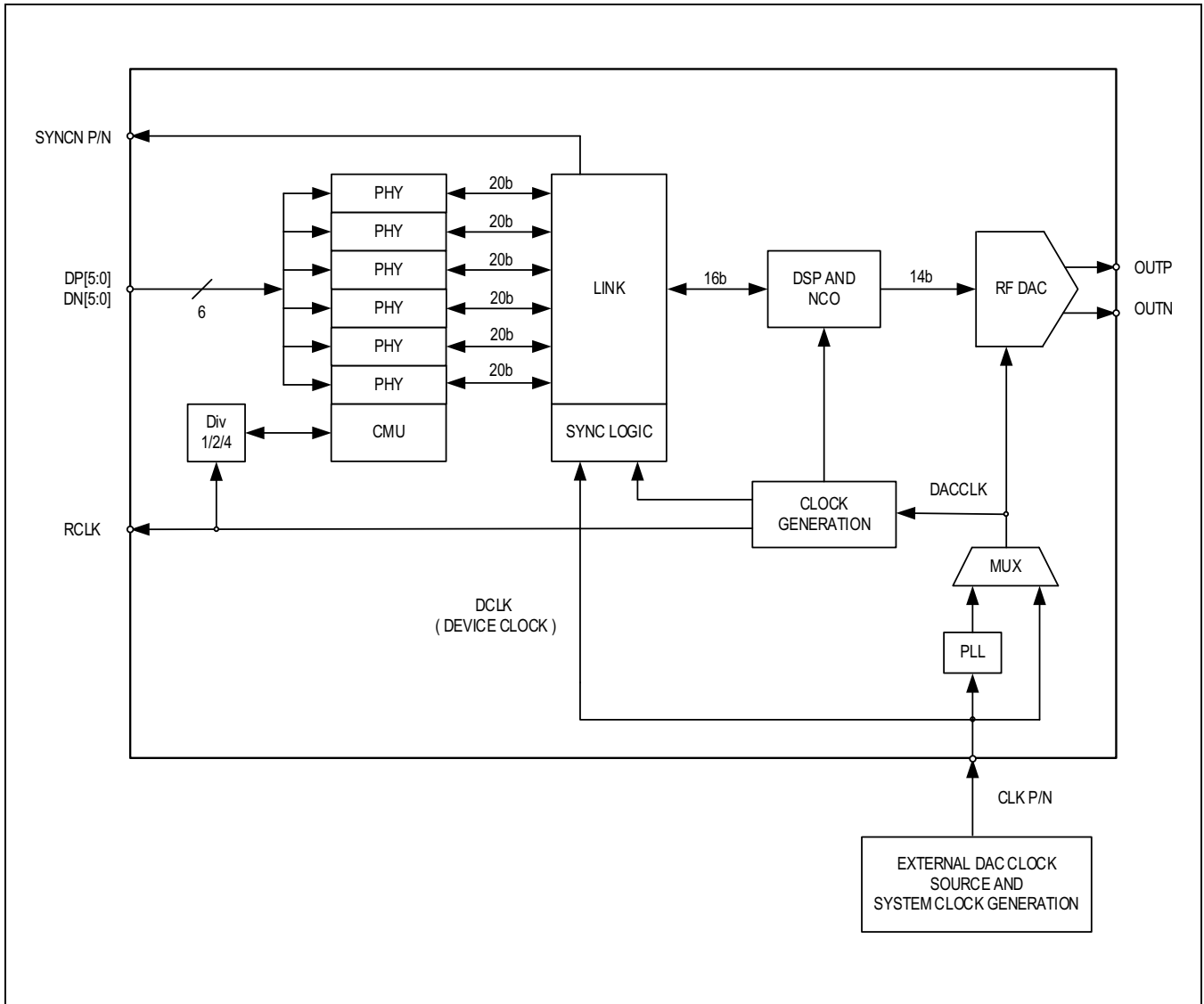
Figure 2. Simplified Diagram of JESD204B Internal to MAX5857
