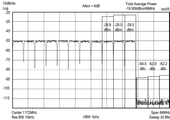
32-CHANNEL 256-QAM (DOCSIS) ACP UPPER CHANNELS ( f_{CENTER} = 1100MHz , T_J = 65^\circ C )
