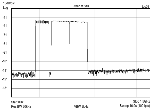
24-CHANNEL 256-QAM (6MHz Wide) and 2x192MHz OFDM CHANNELS (DOCSIS 3.1, Ncp=512, Nrp=64, 1024-QAM, 4096pt FFT) TOTAL AVERAGE POWER = -15dBFS, f_{NCO} = 528MHz , T_J = 65^{\circ}C
