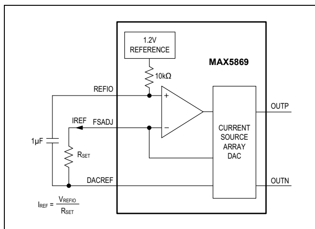
Figure 25a. Reference Architecture, Internal Reference Configuration
