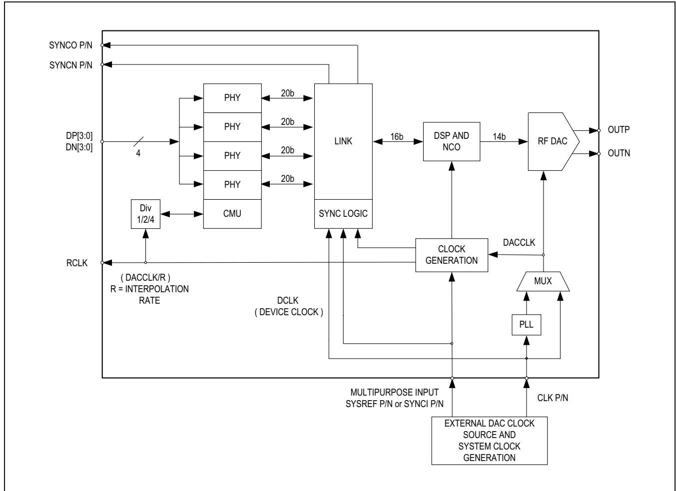
Figure 1. Simplified Diagram of JESD204B Internal to MAX5869
