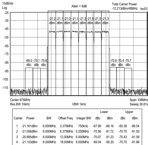
8-CHANNEL 256-QAM (DOCSIS) ACP ( f_{CENTER} = 975MHz , T_J = 65^\circ C )
