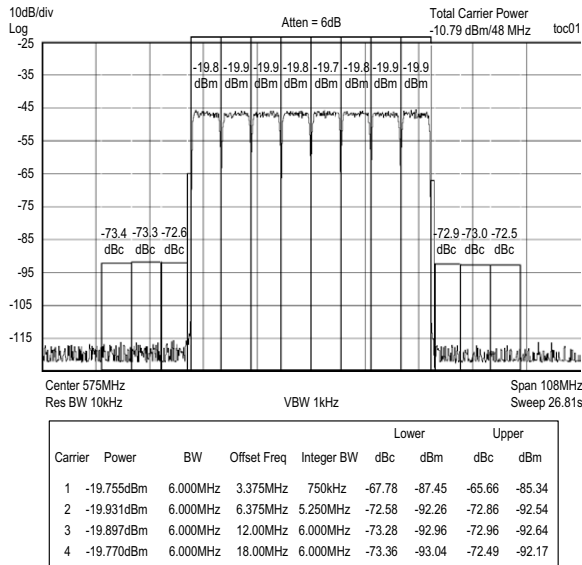
8-CHANNEL 256-QAM (DOCSIS) ACP ( f_{CENTER} = 575MHz , T_J = +65^\circ C )
