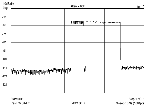
24-CHANNEL 256-QAM (6MHz Wide) and 2x192MHz OFDM CHANNELS (DOCSIS 3.1, Ncp=512, Nrp=64, 1024-QAM, 4096pt FFT) TOTAL AVERAGE POWER = -15dBFS, f_{NCO} = 939MHz , T_J = 65^{\circ}C
