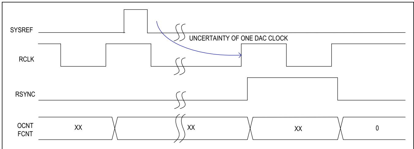
Figure 7. SYSREF Usage for Sample Clock (From DACCLK) Generation and Synchronization
