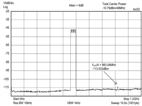
8-CHANNEL 256-QAM (DOCSIS) ACP ( f_{CENTER} = 575MHz , T_J = 65^\circ C )
