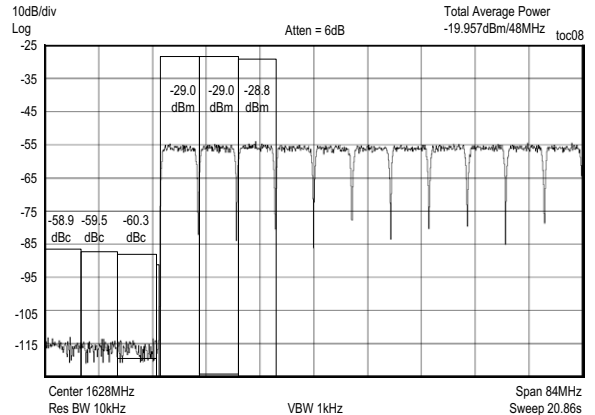
32-CHANNEL 256-QAM (DOCSIS) ACP LOWER CHANNELS ( f_{CENTER} = 1700MHz , T_J = 65^\circ C )
