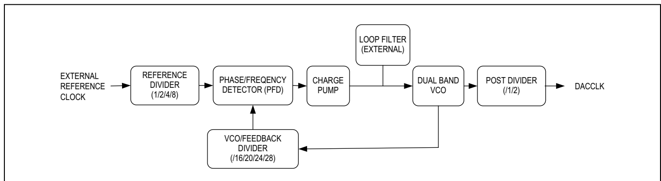
Figure 28. DAC Clock PLL Functional Block Diagram
