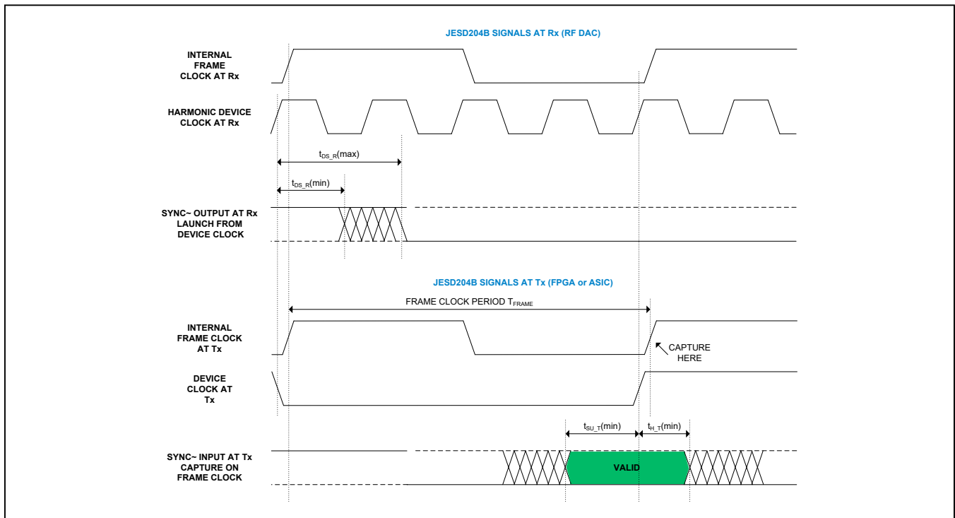
Figure 8. Interface Timing for Subclass-0 (See JEDEC Standard No. 204B.01, Figure 11)
