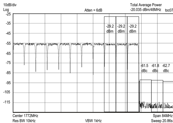
32-CHANNEL 256-QAM (DOCSIS) ACP UPPER CHANNELS ( f_{CENTER} = 1700MHz , T_J = 65^\circ C )
