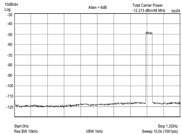
8-CHANNEL 256-QAM (DOCSIS) ACP ( f_{CENTER} = 975MHz , T_J = 65^\circ C )
