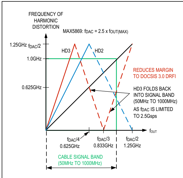
Figure 22a. Example of Incorrect Frequency (Folded HD2/HD3 In-Band)
