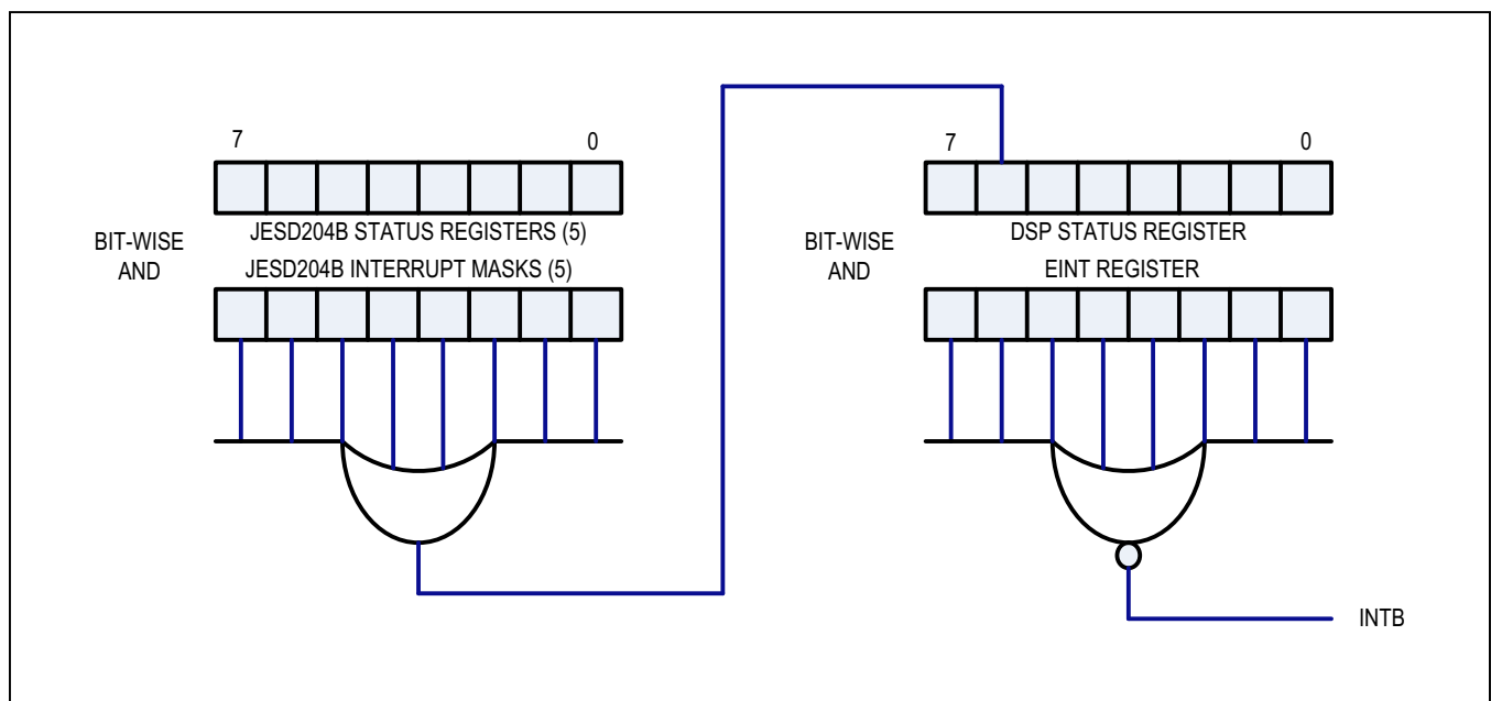
Figure 20. MAX5869 Interrupt Tree
