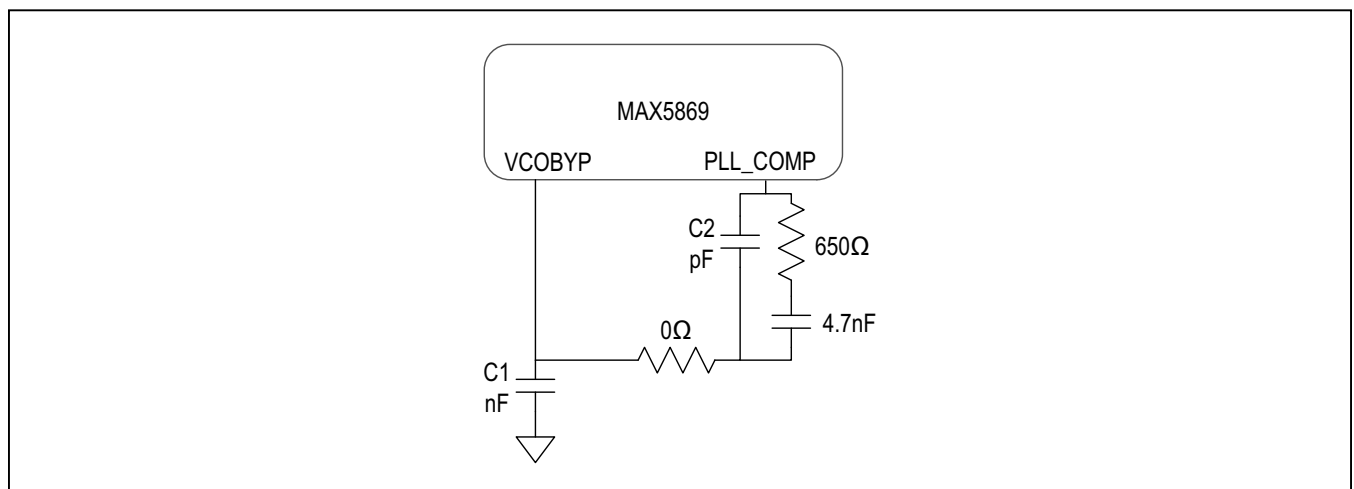
Figure 29. DAC Clock PLL External Components
