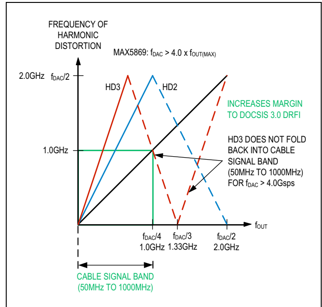
Figure 22b. Example of Correct Frequency (Folded HD2/HD3 Out-of-Band)
