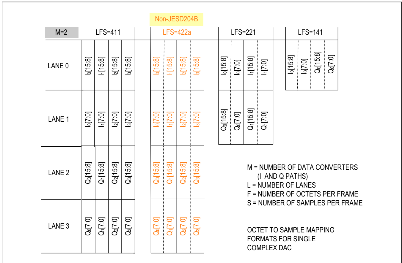
Figure 11. Octet To Sample Conversion vs. Modes and Lanes
