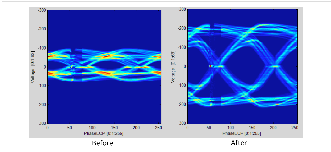
Figure 4. Receiver Equalization Eye Diagram Before and After Lane Training (9.8304Gbps, 30in Nelco Trace)
