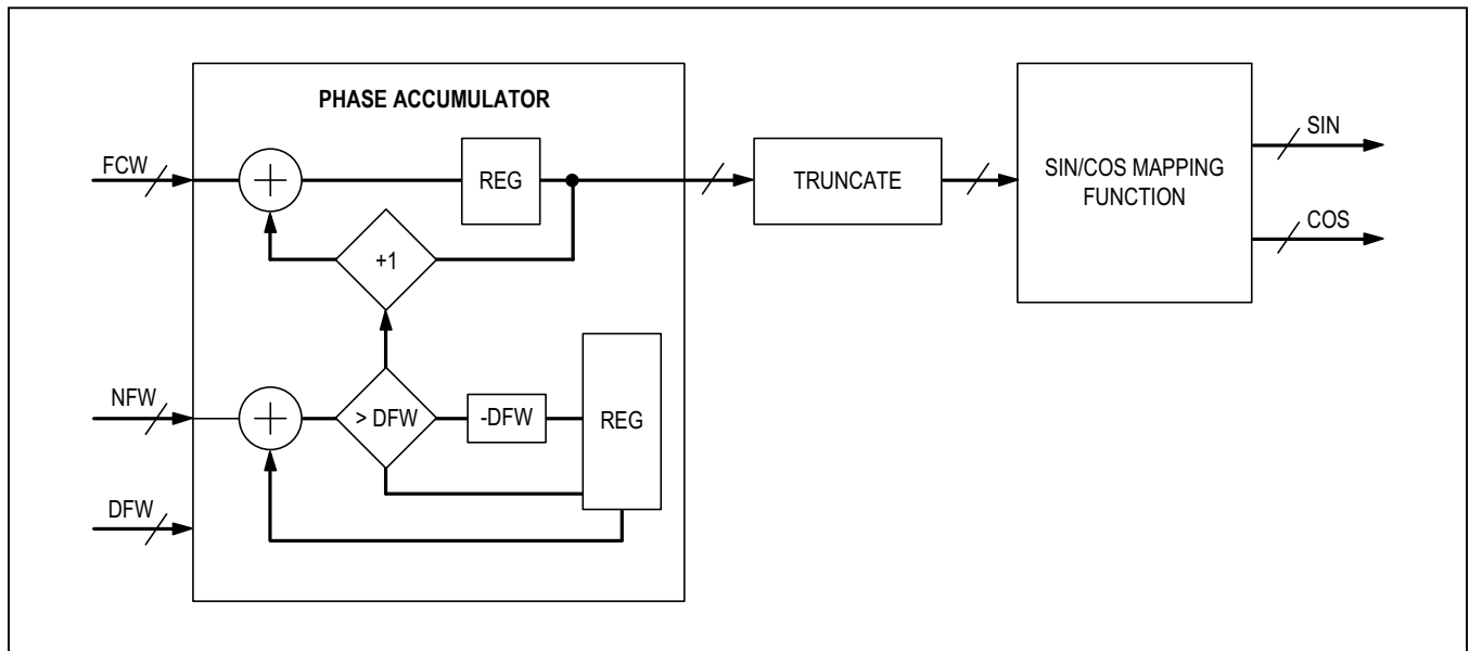
Figure 24. NCO Block Diagram
