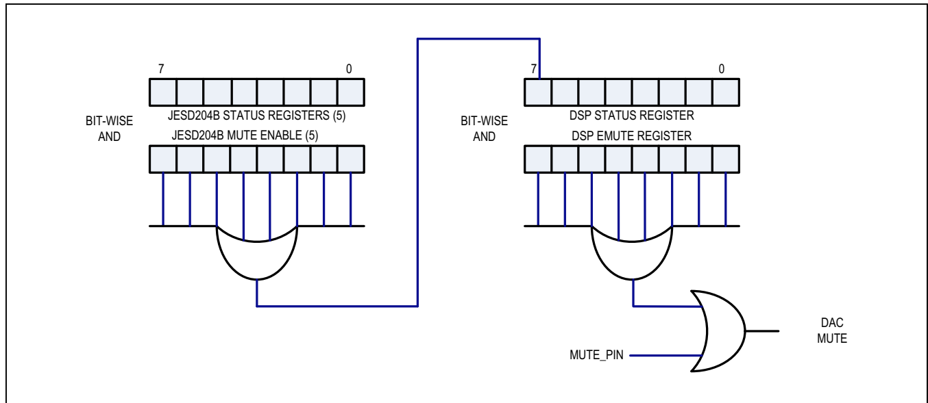
Figure 21. MAX5869 DAC Mute Generation
