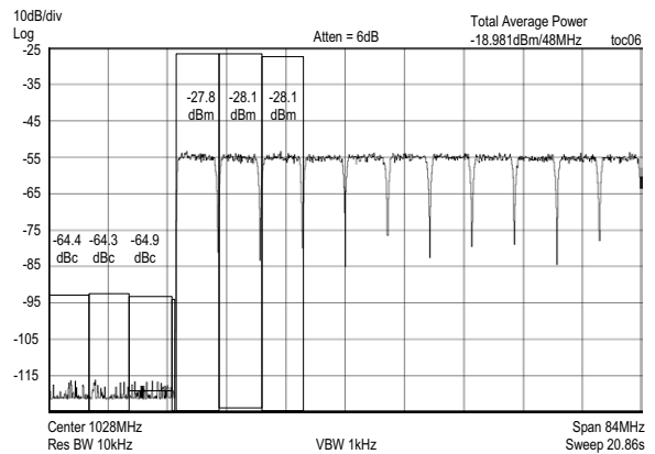
32-CHANNEL 256-QAM (DOCSIS) ACP LOWER CHANNELS ( f_{CENTER} = 1100MHz , T_J = 65^\circ C )
