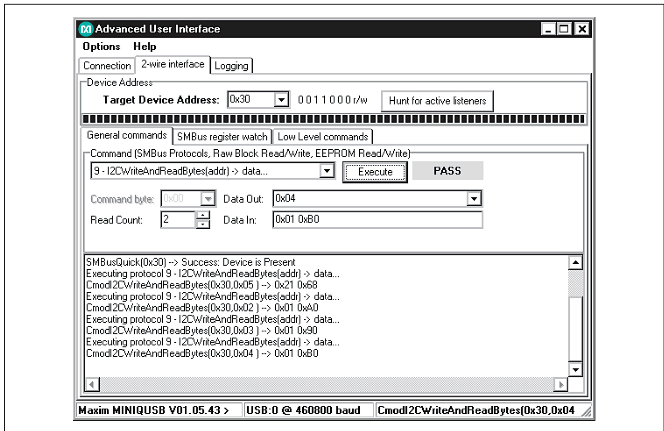
Figure 2. Advanced User Interface Window (2-Wire Interface Tab)
