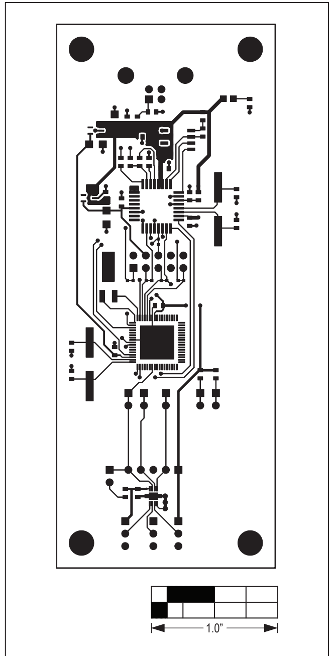
Figure 5. MAX6604 EV Kit PCB Layout—Component Side
