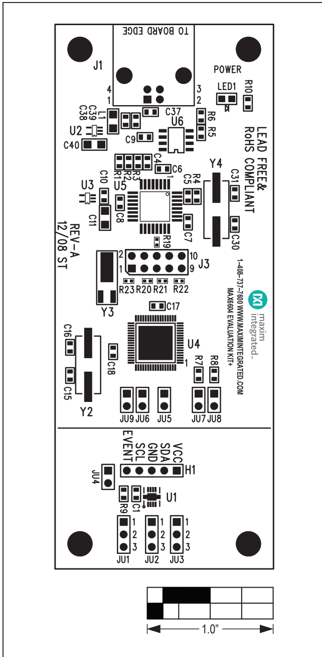
Figure 4. MAX6604 EV Kit Component Placement Guide—Component Side
