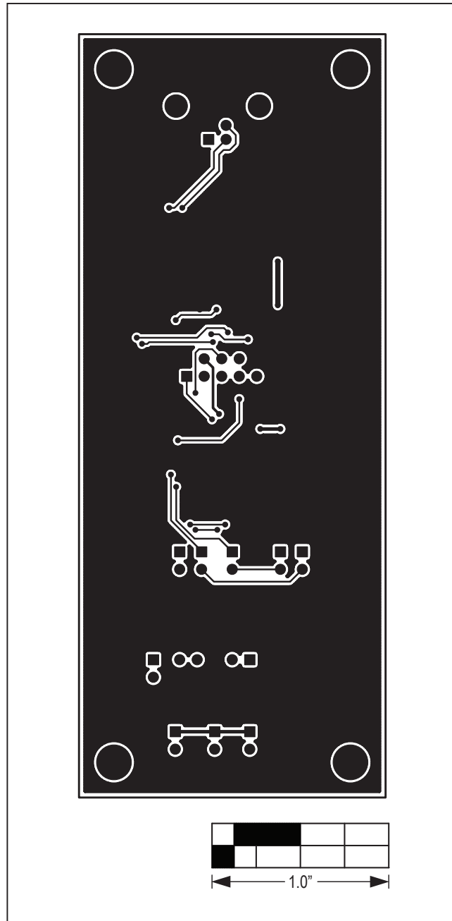
Figure 6. MAX6604 EV Kit PCB Layout—Solder Side
