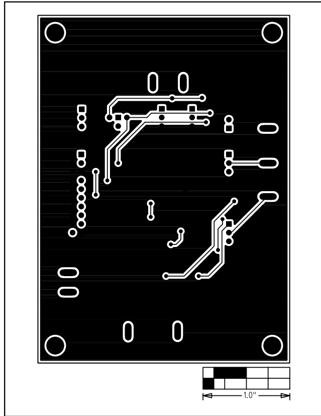
Figure 7. MAX6965 EV Kit PC Board Layout—Solder Side
