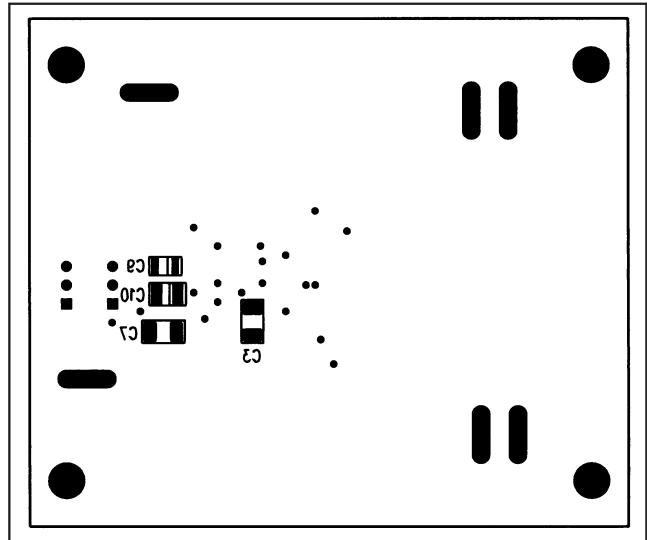
Figure 3. MAX742 EV Kit Component Placement Guide—Solder Side
