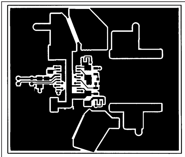
Figure 4. MAX742 EV Kit PC Board Layout—Component Side
