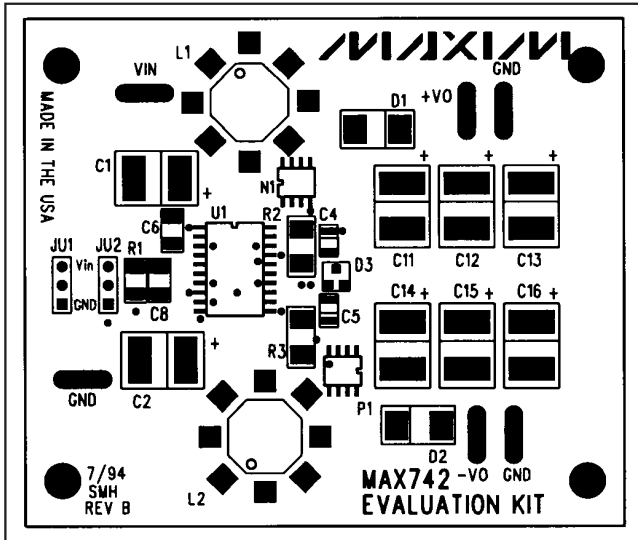
Figure 2. MAX742 EV Kit Component Placement Guide—Component Side
