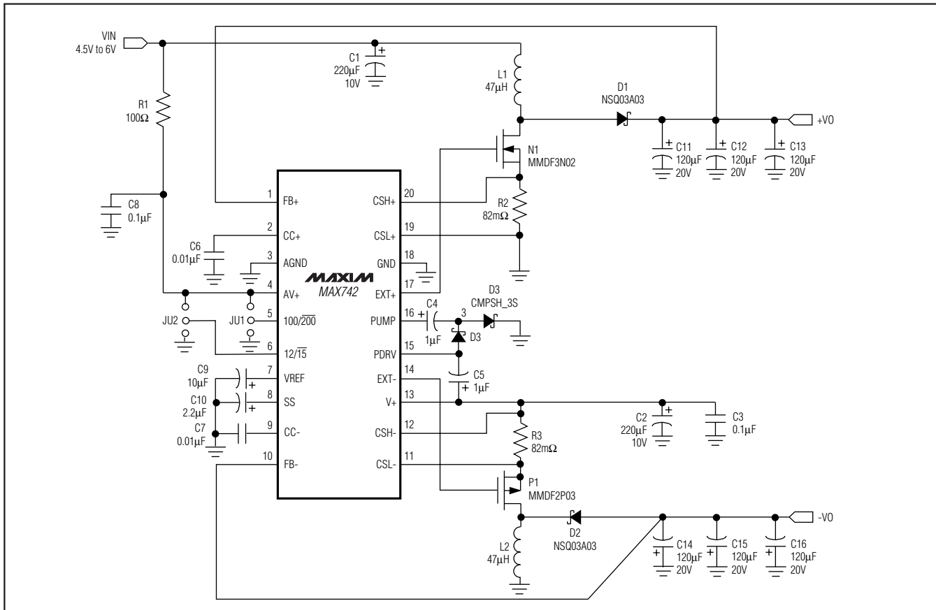
Figure 1. MAX742 EV Kit Schematic
