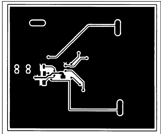
Figure 5. MAX742 EV Kit PC Board Layout—Solder Side
