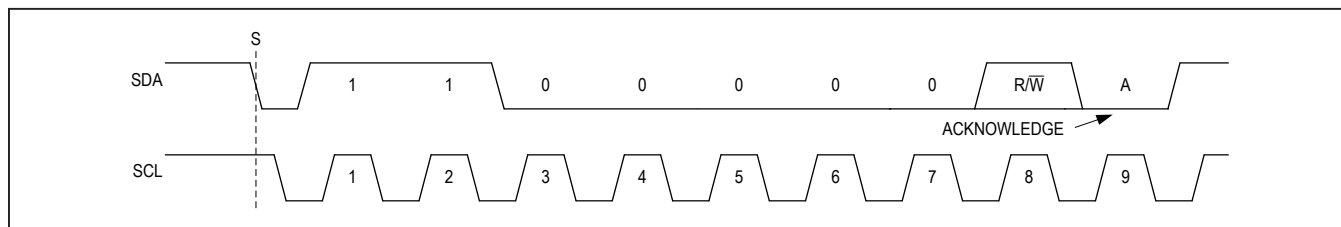
Figure 12. Slave Address Byte Example
