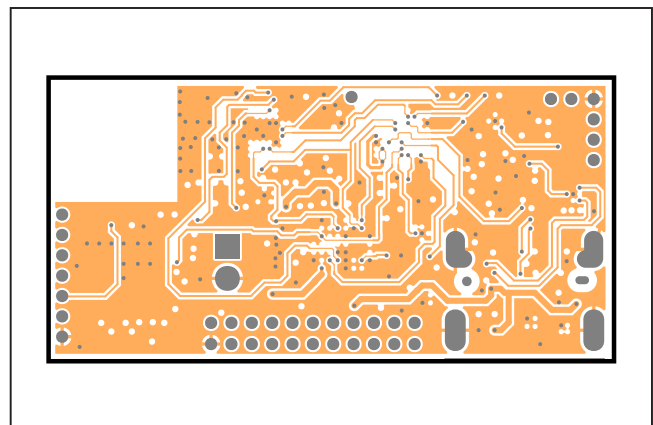
MAXSensorBLE_EVKIT—L05_SIGS
