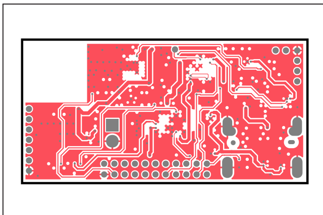
MAXSensorBLE_EVKIT—L04_SIGS
