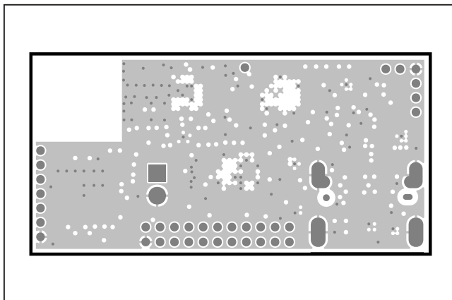
MAXSensorBLE_EVKIT—L02_GND
