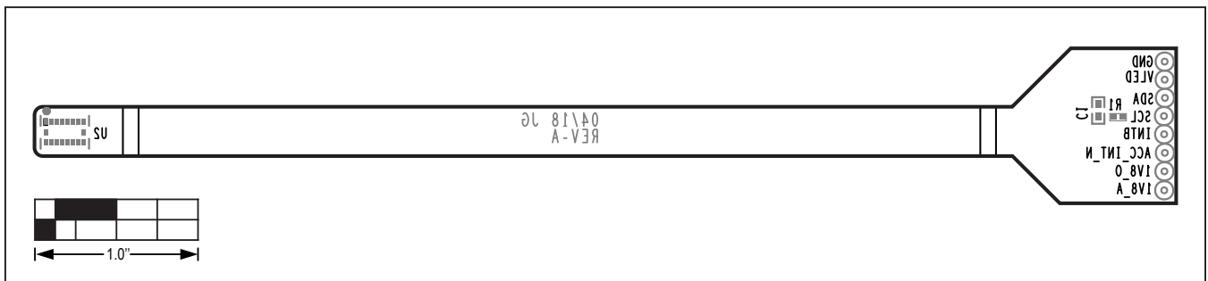
MAX86160OSBEK#—BOTTOM_SILKSCREEN
