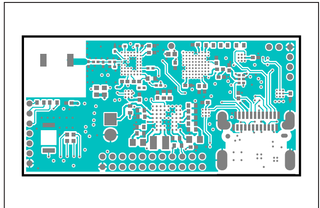
MAXSensorBLE_EVKIT—Top
