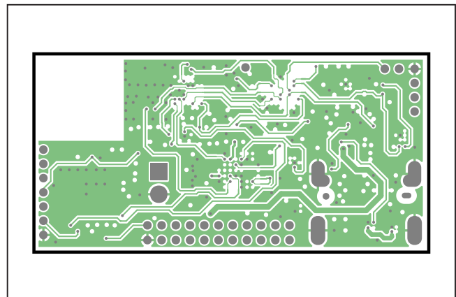
MAXSensorBLE_EVKIT—L03_SIGS
