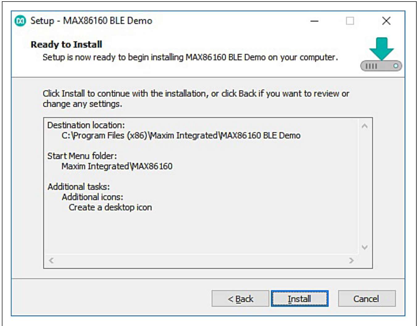
Figure 5. Setup MAX86160 EVSYS GUI Software Step 5
