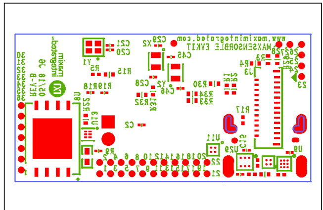
MAXSensorBLE_EVKIT—Bottom Silkscreen
