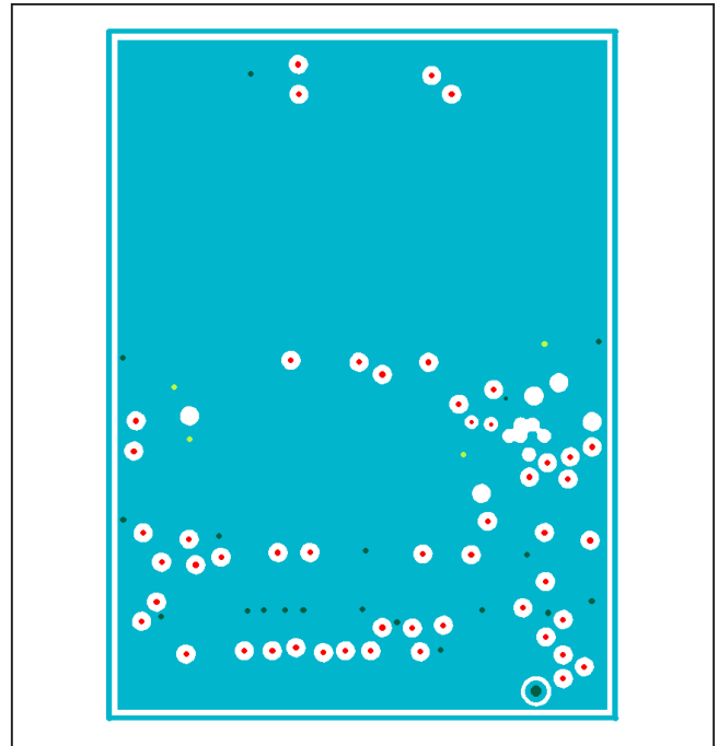
MAX86171OSBEK#—L02_GND
