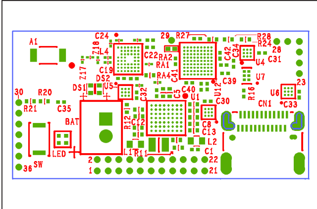
MAXSensorBLE_EVKIT—Top Silkscreen
