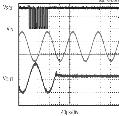
HEADPHONE AMPLIFIER TURN-OFF RESPONSE
