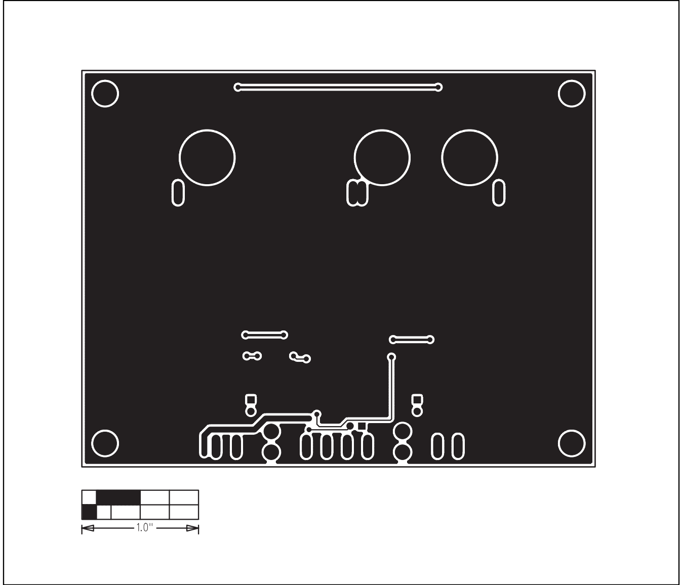
Figure 5. MAX9742 EV Kit PCB Layout—Solder Side
