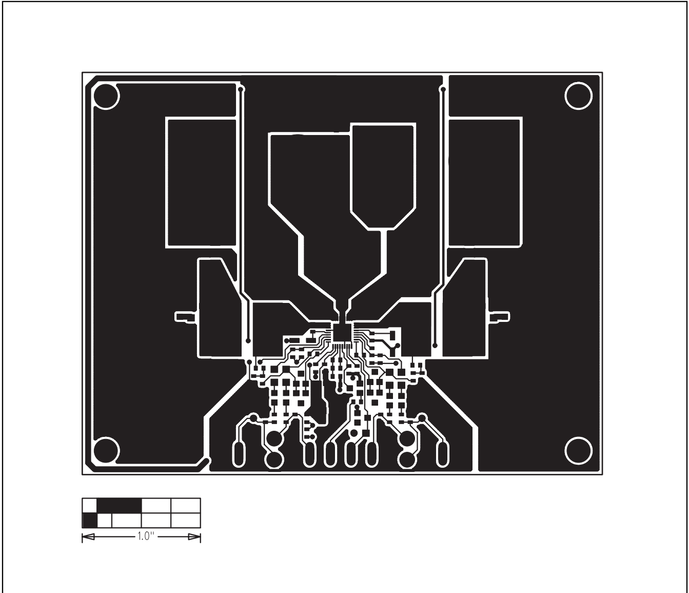
Figure 4. MAX9742 EV Kit PCB Layout—Component Side
