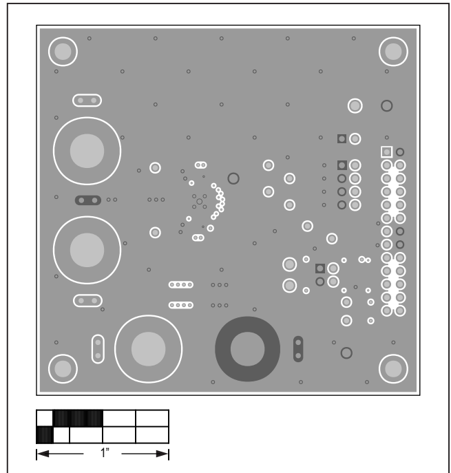
MAX98372 (TQFN) EV Kit PCB Layout—GND Layer 2
