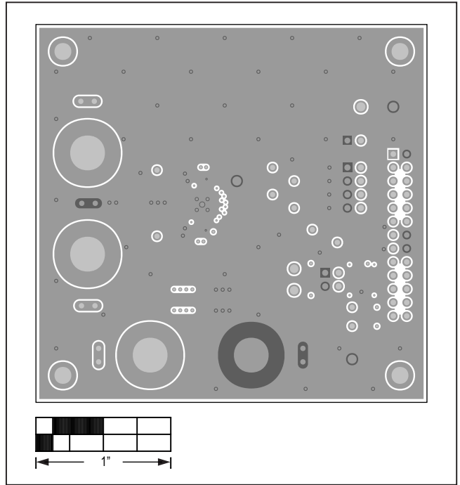
MAX98372 (TQFN) EV Kit PCB Layout—GND Layer 5
