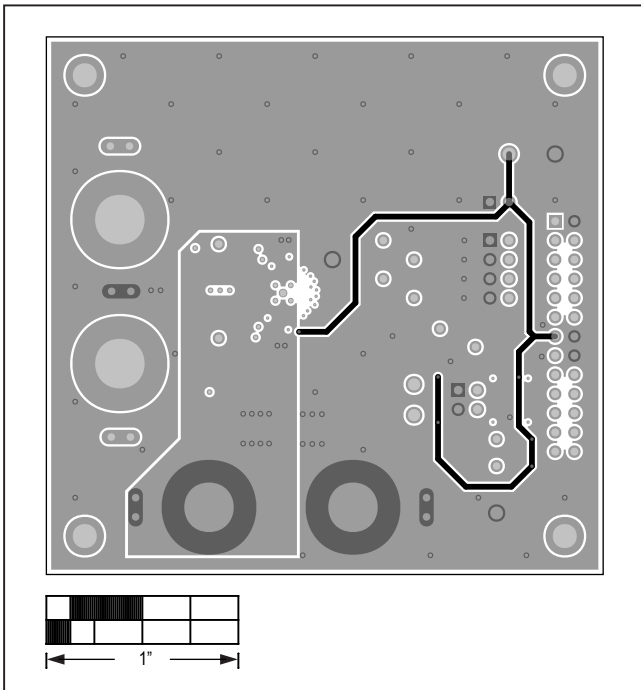
MAX98372 (TQFN) EV Kit PCB Layout—Power Layer 4
