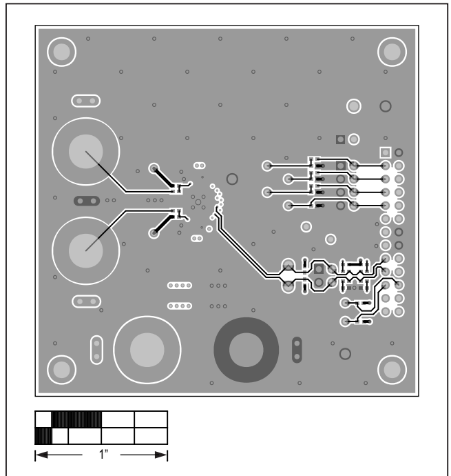
MAX98372 (TQFN) EV Kit PCB Layout—Bottom
