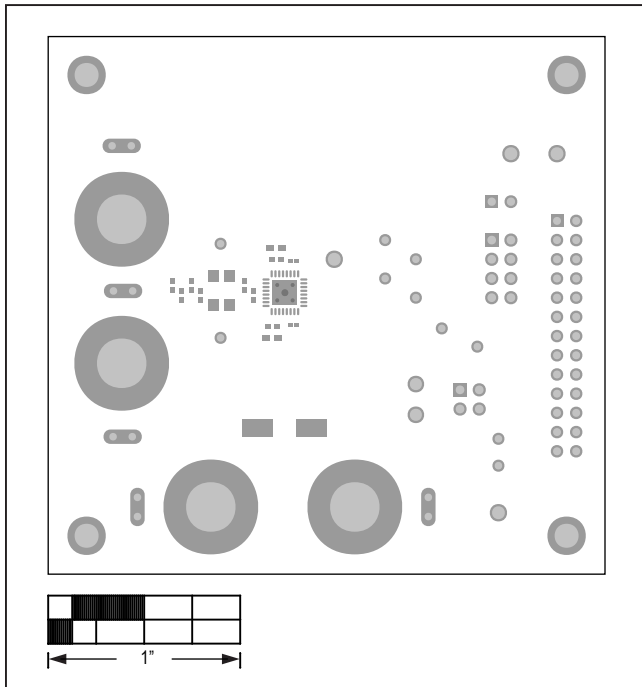
MAX98372 (TQFN) EV Kit PCB Layout—Mask Top
