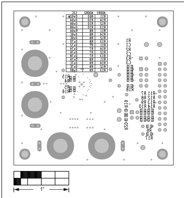
MAX98372 (TQFN) EV Kit Component Placement Guide—Bottom Silkscreen
