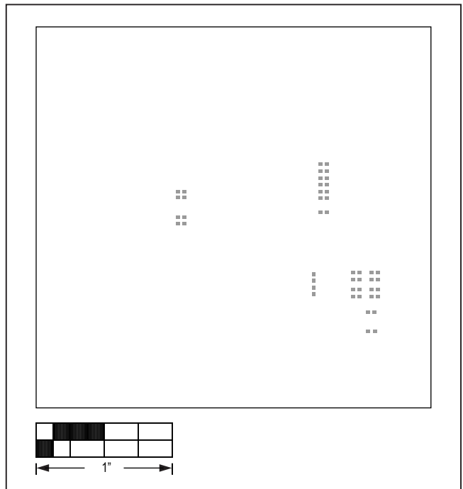
MAX98372 (TQFN) EV Kit PCB Layout—Paste Bottom
