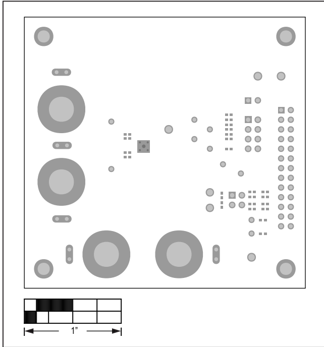
MAX98372 (TQFN) EV Kit PCB Layout—Mask Bottom
