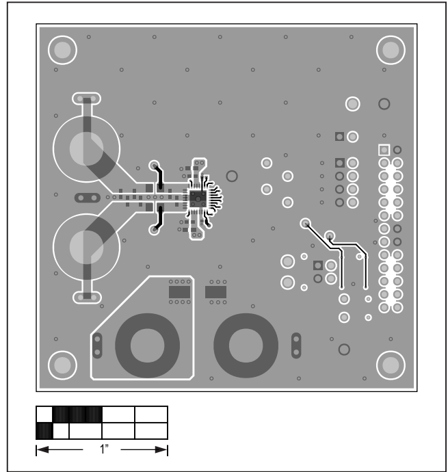
MAX98372 (TQFN) EV Kit PCB Layout—Top
