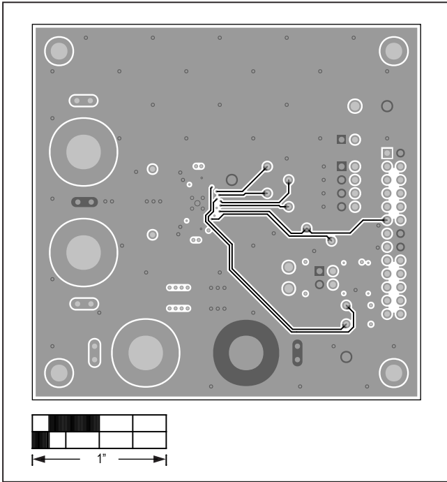
MAX98372 (TQFN) EV Kit PCB Layout—Signal GND Layer 3
