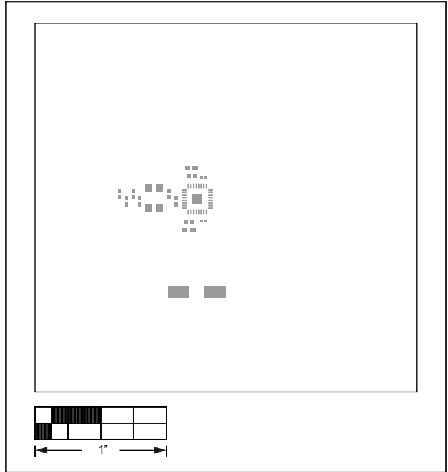
MAX98372 (TQFN) EV Kit PCB Layout—Paste Top
