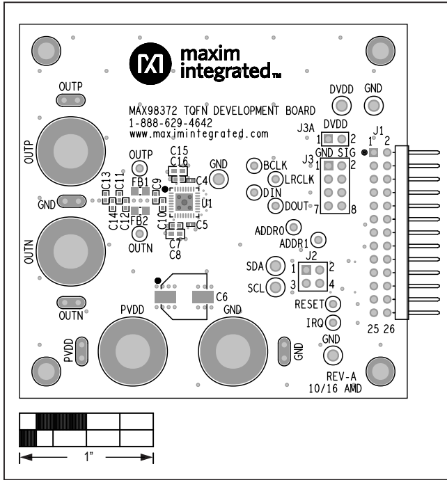
MAX98372 (TQFN) EV Kit Component Placement Guide—Top Silkscreen
