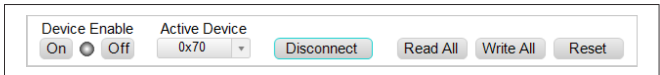
Figure 4. Communication Toolbar
