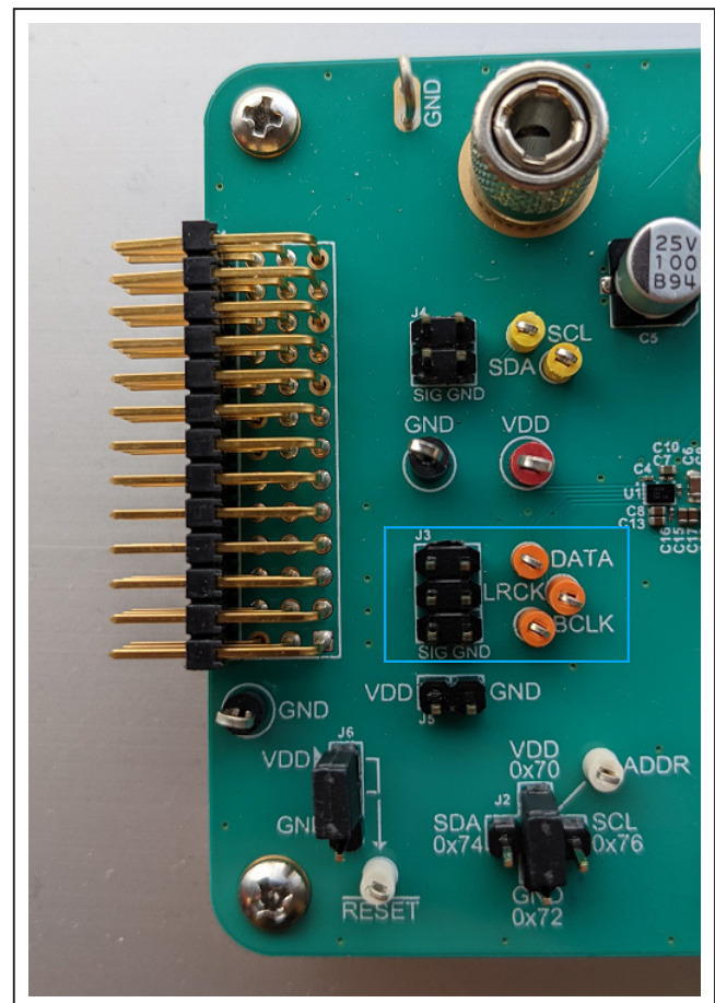
Figure 8. MAX98380 DAI Interface Headers
