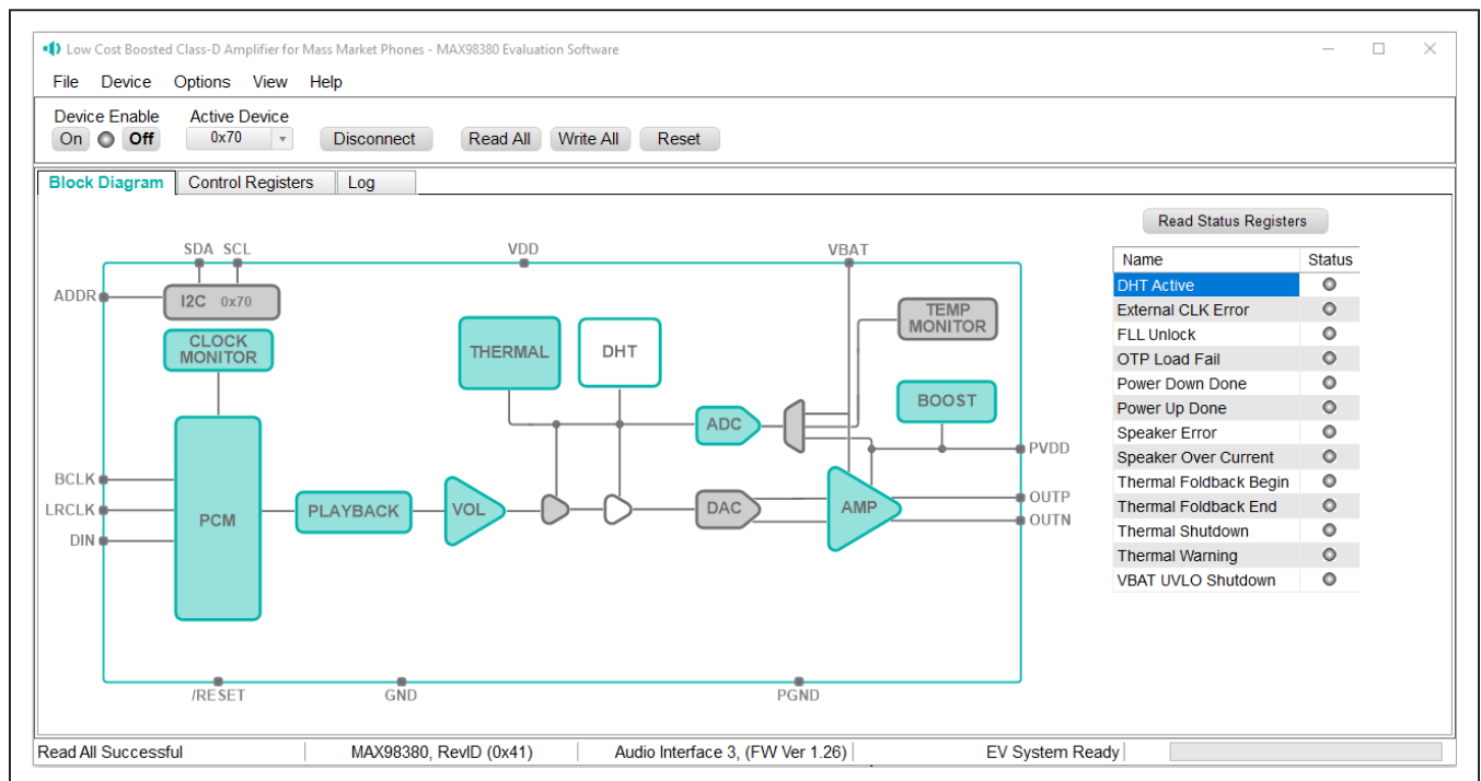
Figure 5. MAX98380 Block Diagram—USB Audio Input to Speaker Output
