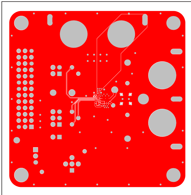
MAX98380 EV Kit PCB Layout—Top Layer
