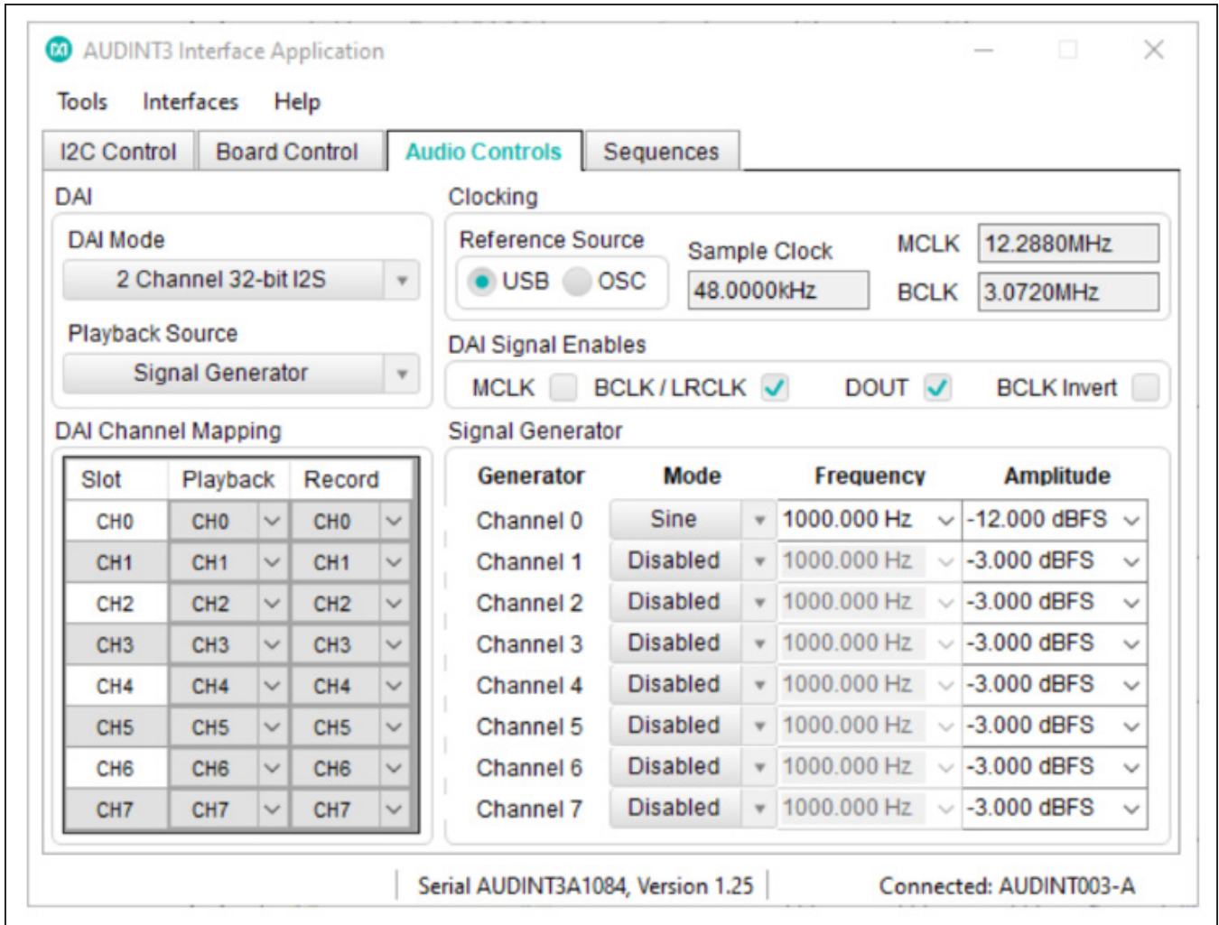
Figure 10. AUDINT3 Configured for a -12dBFS 1kHz Sine Input using an Internal Signal Generator
