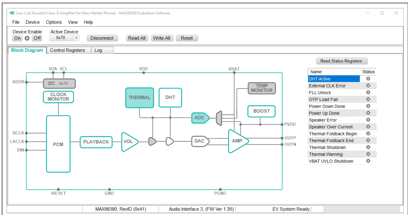
Figure 3. MAX98380 Evaluation Software—Main Window
