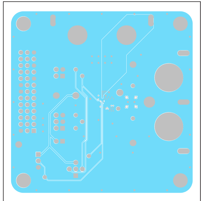
MAX98380 EV Kit PCB Layout—Layer 3
