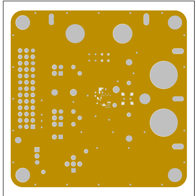
MAX98380 EV Kit PCB Layout—Layer 2
