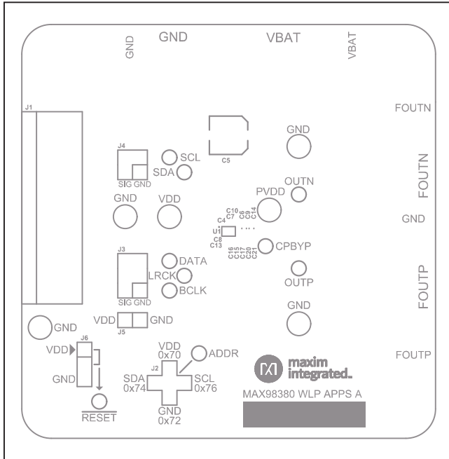
MAX98380 EV Kit Component Placement Guide—Top Silkscreen
