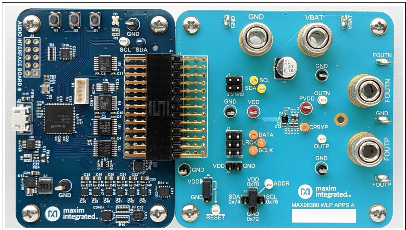
Figure 1. MAX98380 Evaluation System
