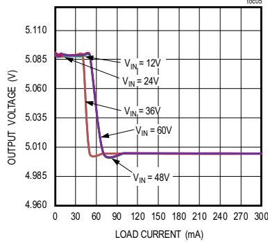
OUTPUT VOLTAGE vs. LOAD CURRENT V_{OUT} = 5V , PFM MODE
