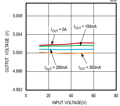
OUTPUT VOLTAGE vs. INPUT VOLTAGE V_{OUT} = 5V , PWM MODE
