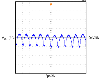
OUTPUT VOLTAGE RIPPLE V_{IN} = 24V , V_{OUT} = 5V FULL LOAD, PWM MODE
