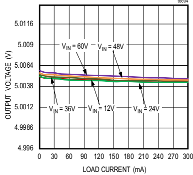
OUTPUT VOLTAGE vs. LOAD CURRENT V_{OUT} = 5V , PWM MODE
