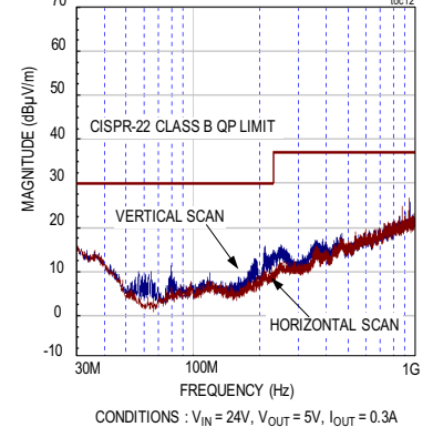
(C6 = 0.1µF, C7, C8, C9 = OPEN, L1 = SHORT)
