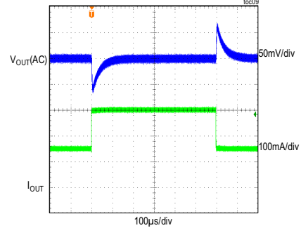
LOAD TRANSIENT RESPONSE V_{IN} = 24V , V_{OUT} = 5V , PWM MODE (LOAD CURRENT STEPPED FROM 150mA TO 300mA)
