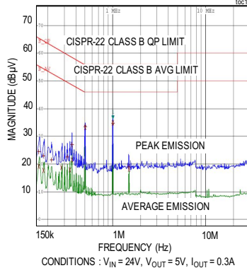
CONDUCTED EMISSION PLOT (EMI FILTER C = 0.1µF + 0.68µF, L = 82µH, C = 1µF)
