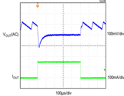
LOAD TRANSIENT RESPONSE V_{IN} = 24V , V_{OUT} = 5V , PFM MODE (LOAD CURRENT STEPPED FROM 5mA TO 150mA)
