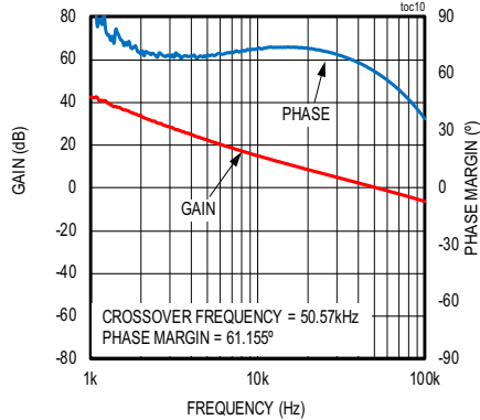
V_{IN} = 24V , V_{OUT} = 5V , FULL LOAD, PWM MODE
