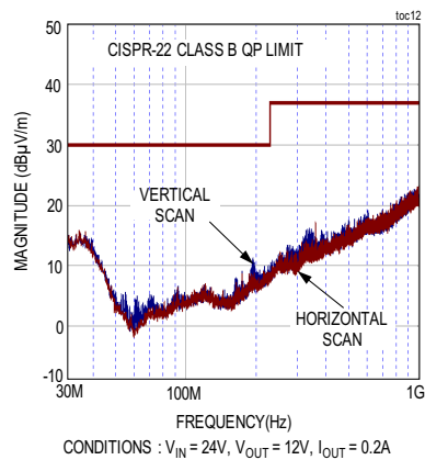
RADIATED EMISSION PLOT L_{EMI\_1} = \text{SHORT}, C_{EMI\_1} = C_{EMI\_2} = \text{OPEN}
