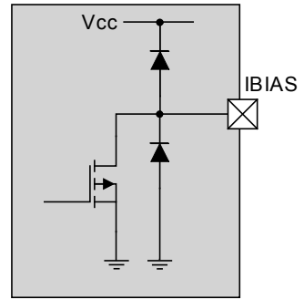
Figure 30 - Laser bias output structure
