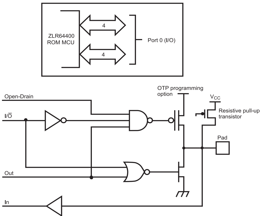
Figure 4. Port 0 Configuration
