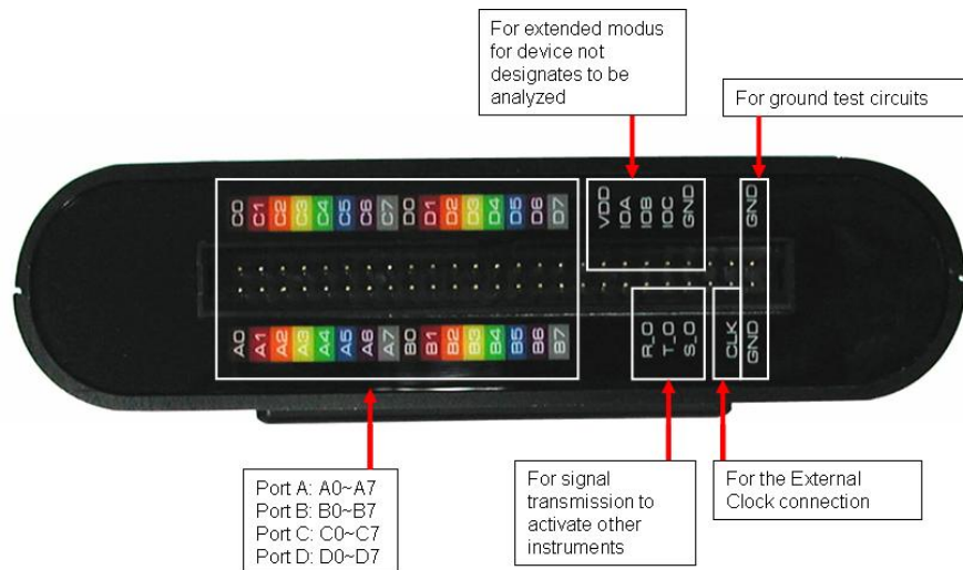
Fig. 1-10: Side View of the AKIP Logic Analyzer; the power of the Logic Analyzer is drawn from the USB connection.
