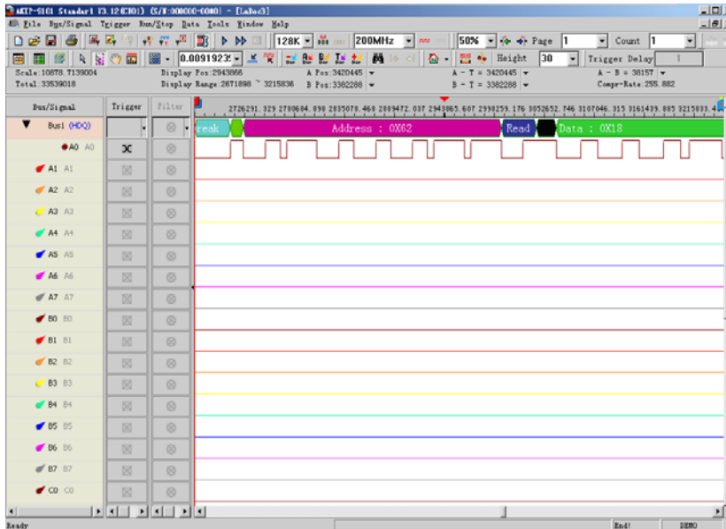
Fig4-118- Protocol Analyzer HDQ Decoding
