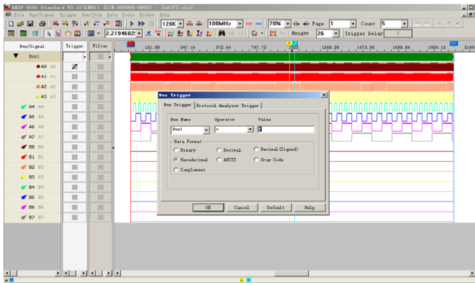
Fig 4-32 – Bus Trigger Setup
