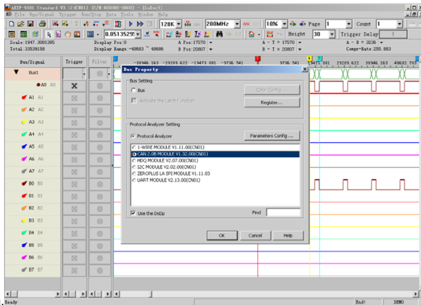
Fig4-132 - CAN 2.0B Bus Property Setup
