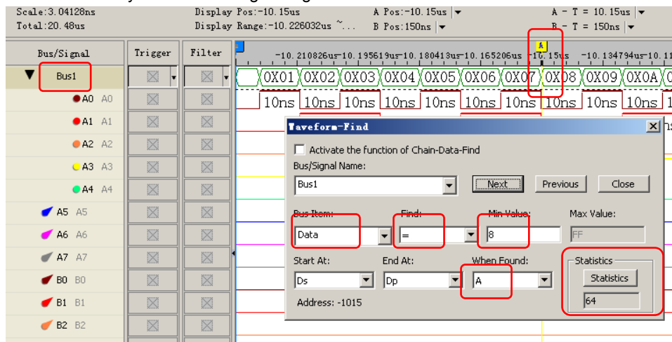
Fig 3-124: The A Bar is placed at the 0X08 of Bus1 where the condition of the Waveform-Find is set. The Statistic of Waveform-Find shows a "64".
