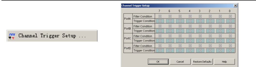
Fig 3-32: The trigger action tells the Logic Analyzer when to send data to the PC. The trigger conditions determine when the trigger point starts to record the information.
