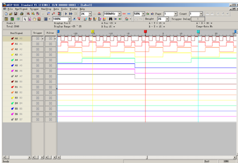
Fig4-129 - CAN 2.0B Waveform
