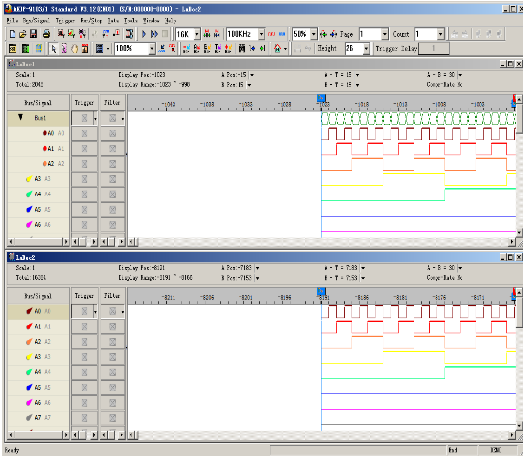
Fig4-155 - Display the Contrast Results in the Waveform Windows
