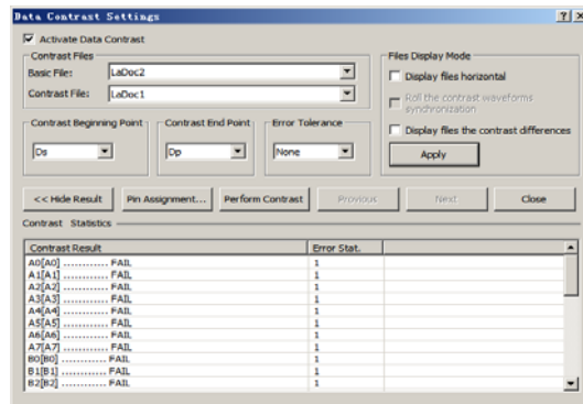
Fig4-154 - Display the Contrast Results in the Data Contrast Settings Dialog Box
