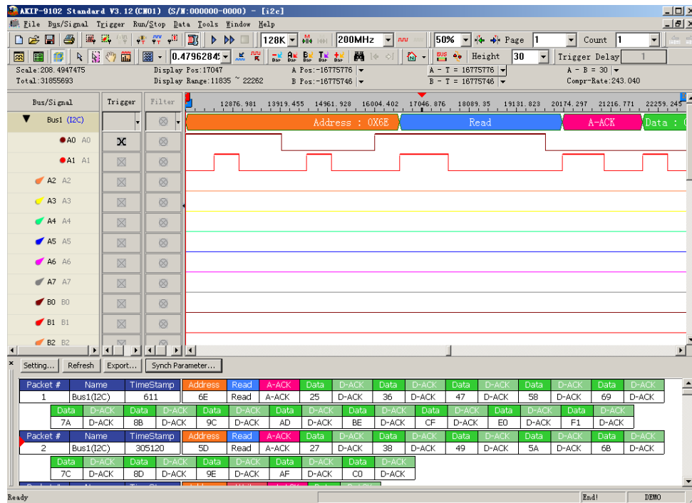
Fig 4-53 - Waveform and Packet Synchronization Interface
