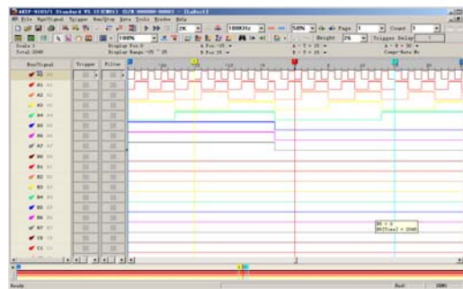
Fig3-105: Reverse Function Displayed in the Waveform Window
