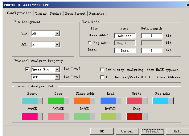
Fig 4-67 – Protocol Analyzer I2C Configuration dialog box
