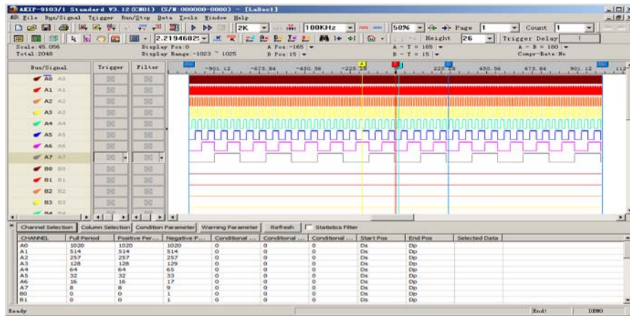
Fig 3-128: Logic Analyzer with Statistics Enabled
