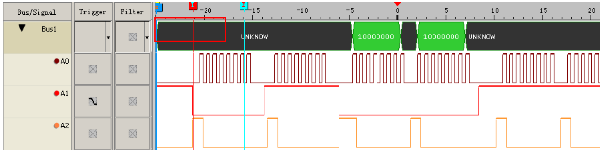
Fig4-159 - Analyze the Data Between Ds and Dp
