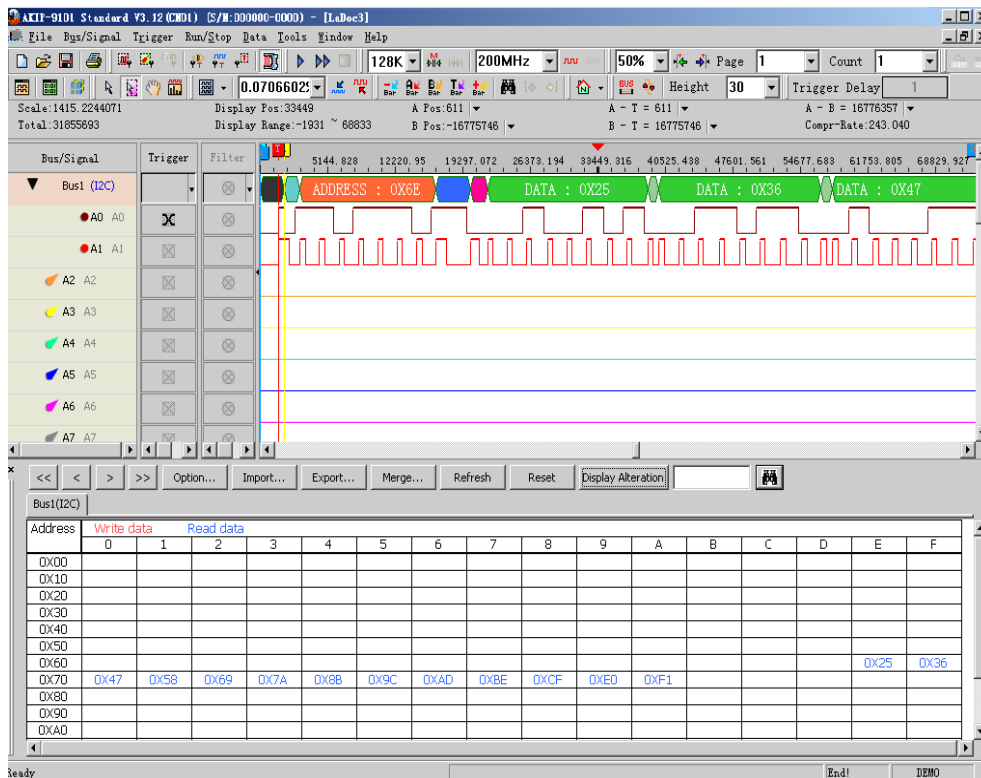
Fig4-169 – Memory Analyzer Display
