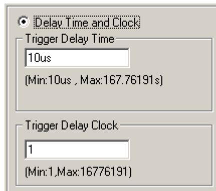
Fig. 6-2 – Delay Time and Clock
