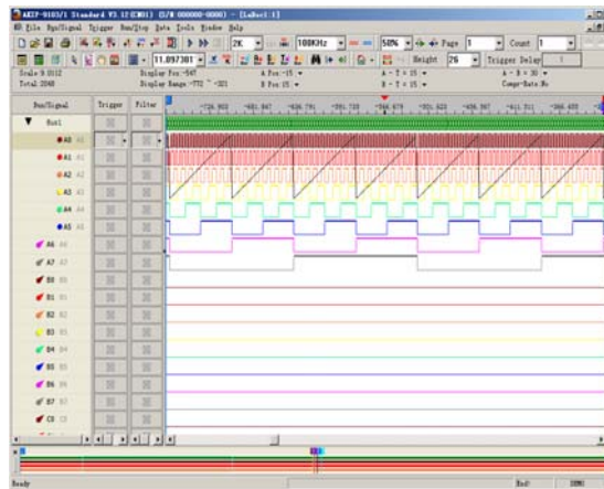
Fig 3-83: Mixed Analog Display
