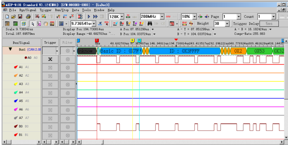
Fig4-134 - CAN 2.0B Decoding
