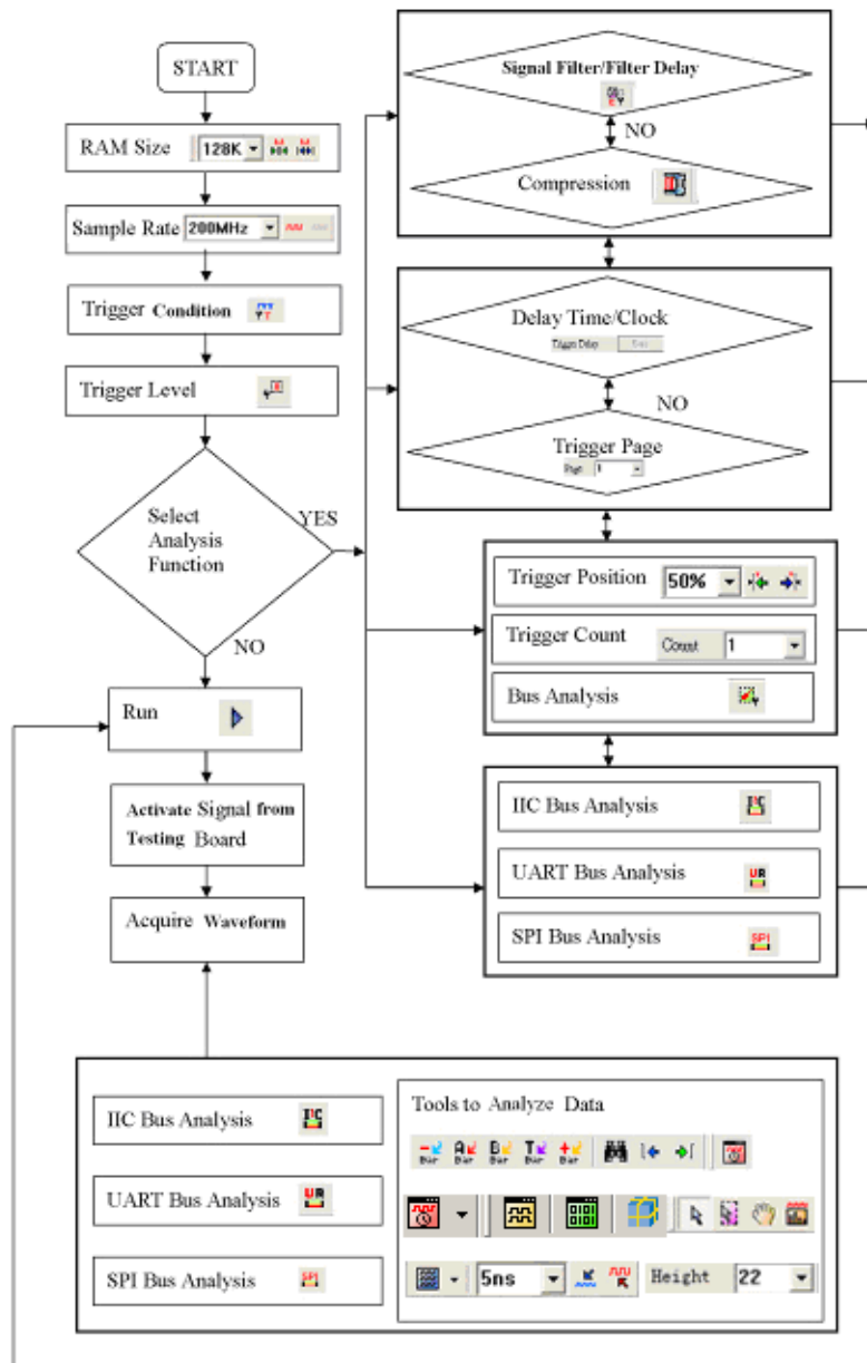
Fig 3-155: Software Flow Diagram
