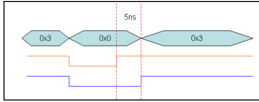
Fig3-45: Before and After Filtering
