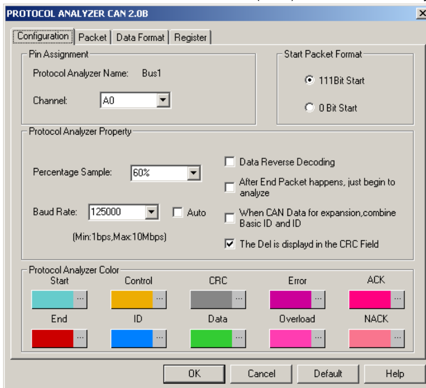
Fig4-133 - Protocol Analyzer CAN 2.0B Setup
