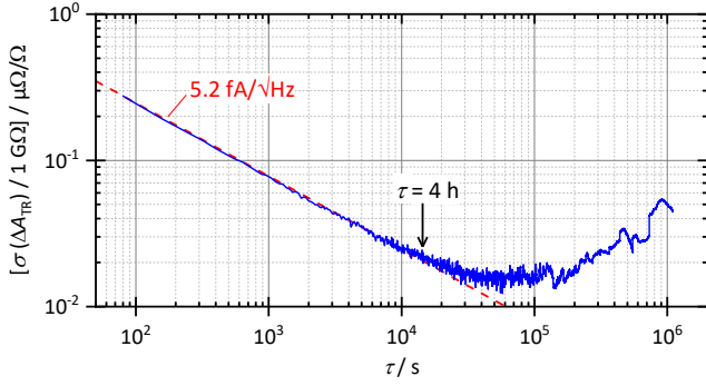
Fig. 9. Allan deviation plot of the ULCA-ULCA calibration measurements. The red dotted line is a fit corresponding to white noise of 5.2 \text{ fA}/\sqrt{\text{Hz}} , calculated using Eq. 2 in ref. [2] with an effective integration time \tau_e = \tau/4 . \tau_e is reduced with respect to \tau by a factor of 2 due to the sequential measurement mode (using the MUX), and by another factor of 2 due to the disregarded data after current reversal (suppressing transients).
