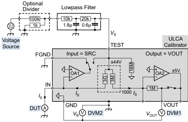
Fig. 1. Setup for the calibration of an electrometer (device under test, DUT) using an ULCA calibrator configured for current source mode ( I_s \leq 5 nA).
