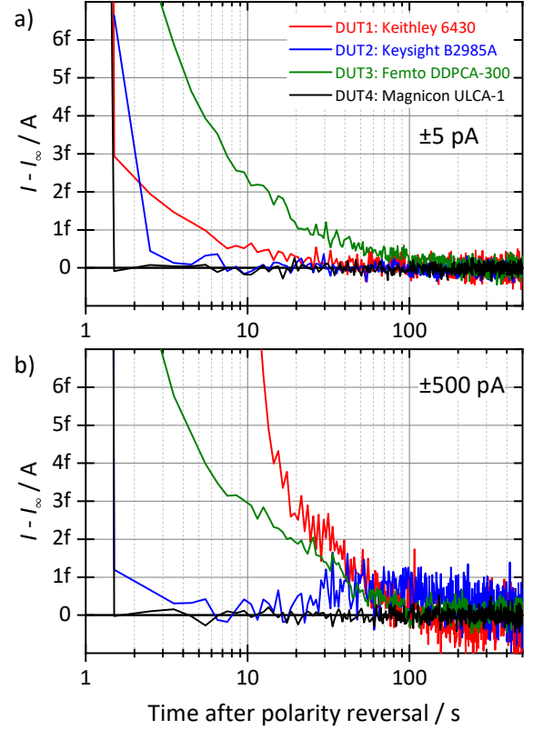
Fig. 4. Settling behavior of the DUTs. Plotted are the DUT output signals versus time after polarity reversal for I_S = \pm 5 pA and \pm 500 pA. I_\infty is the final current signal asymptotically approached. Each curve is the result from averaged data measured over periods of about two to four days. Responses from both switching directions were considered: data from positive current steps were directly used, whereas those for negative steps were inverted before averaging.
