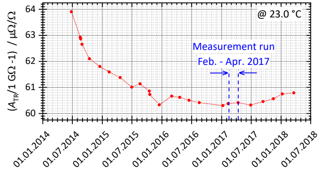
Fig. 2. Calibration results for the total transresistance A_{\text{TR}} of the calibrator ULCA, all performed against a quantum Hall resistance standard and referred to a temperature of 23.0 °C. Error bars corresponding to the calibration uncertainty are smaller than the symbol size. The period of 7 weeks in which the measurements for section IV of this paper were performed is indicated.
