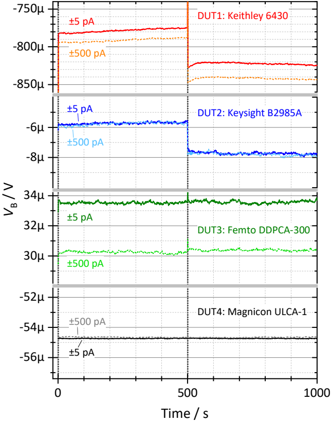
Fig. 5. Measurements of V_B versus time for I_S = \pm 5 pA and \pm 500 pA. Current polarity reversal happened at t = 0 s and 500 s. Note that the range of the y-axis for DUT1 is 20 times the range for the other DUTs. Each curve is the result from averaged data measured over a period of about two to four days.
