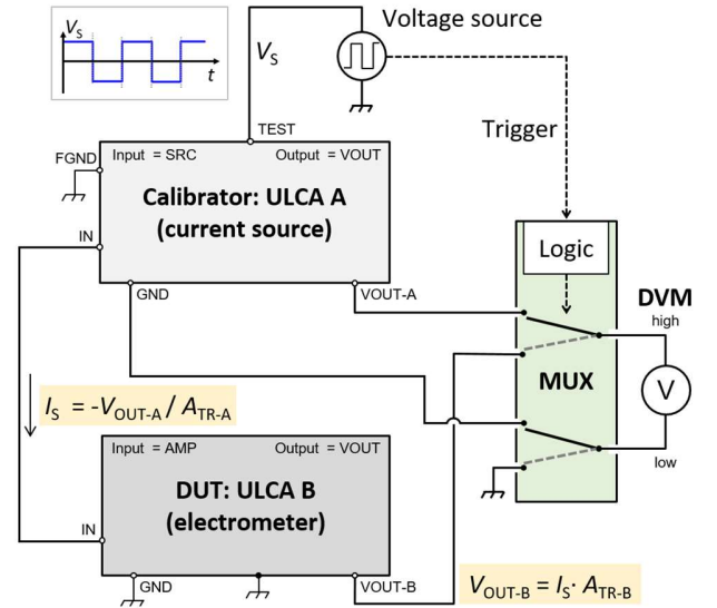
Fig. 8. Advanced setup for the calibration of electrometers with analog voltage output (here: ULCA B) with ULCA A used as calibrator current source, involving a multiplexer circuit (MUX) and a single DVM to measure the outputs of both instruments alternatingly. The voltage source biasing the calibrator ULCA with V_S also gives the trigger signal controlling the MUX switching events.
