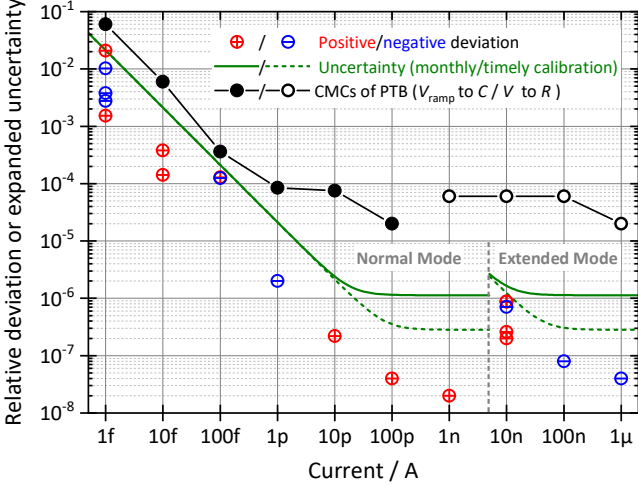
Fig. 7. Red and blue circled symbols show the measurement results from the triangle comparison as sketched in Fig. 6, plotted as relative deviations \Delta A_{TR}/1 \text{ G}\Omega (+/- symbols indicate positive/negative values). Green lines show calculated expected upper limits for the measurement results, based on uncertainty estimates. Black circle symbols represent the present CMC values of PTB for two different, not ULCA-based calibration methods. “Normal” (“extended”) mode refers to the current I_S < (>) 5 \text{ nA} and corresponding configurations of the ULCA instruments. All values correspond to expanded uncertainties (coverage factor k = 2 , or 95% confidence interval).
