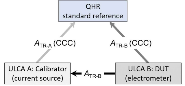
Fig. 6. Triangle comparison involving two ULCA instruments A and B, both calibrated against QHR with highest accuracy and directly compared using the calibration setup shown in Fig. 1.
