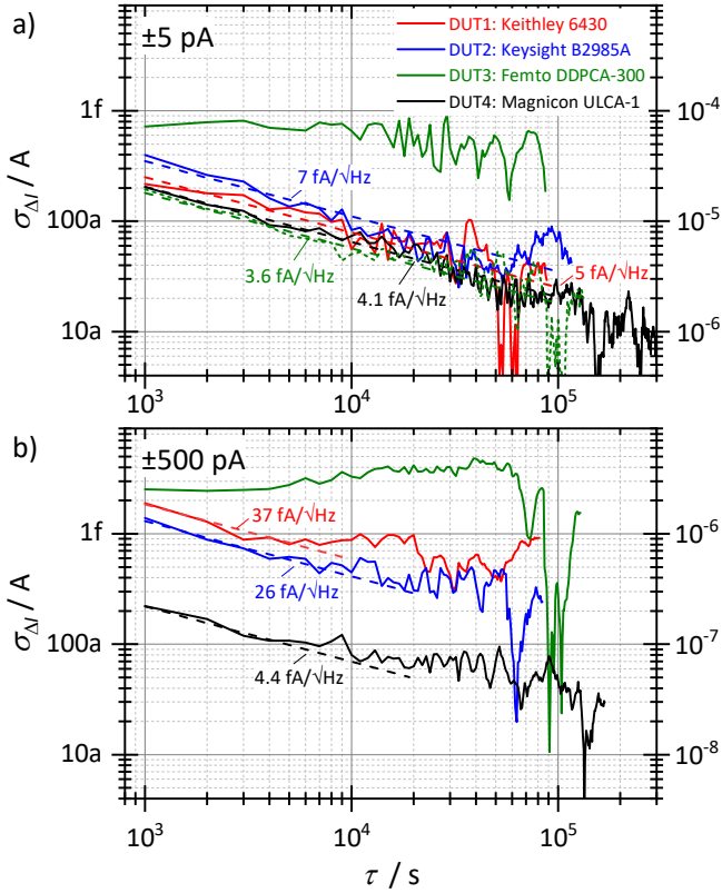
Fig. 3. Allan deviation plots of the DUT error current \Delta I for I_S = \pm 5 pA and \pm 500 pA. Current values as input data for the analysis were computed from the differences of DUT signal data averaged over the negative and positive half-cycles. The first 50 s after each current reversal were rejected to suppress transients. White noise levels, indicated by the dotted fit lines, were calculated using Eq. 2 in ref. [2], considering an effective integration time \tau_e = 0.9 \cdot \tau . The axes on the right side are scaled in relative units, normalized to I_{pp} = 2|I_S| = 10 pA and 1 nA, respectively. Panel a) shows an additional measurement on DUT3 performed at \pm 50 fA (green dotted curve), which corresponds to a noise level of 3.6 fA/√Hz. In this case, the right scale is to be multiplied by a factor of 100 to account for the reduced current level.
