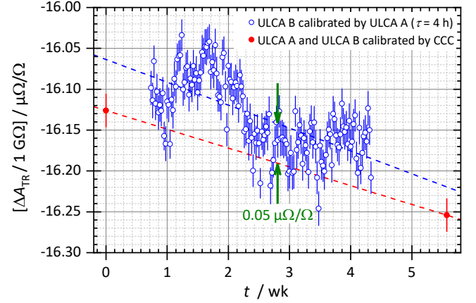
Fig. 10. Blue data points (open symbols) show calibration results using the setup shown in Fig. 8 with I_S = \pm 3 \text{ nA} and data averaged for \tau = 4 \text{ h} . Red points (full symbols) show the results from calibrations of A_{\text{TR-A}} and A_{\text{TR-B}} performed against QHR by using a cryogenic current comparator. Dotted lines represent linear fits to both data sets.
