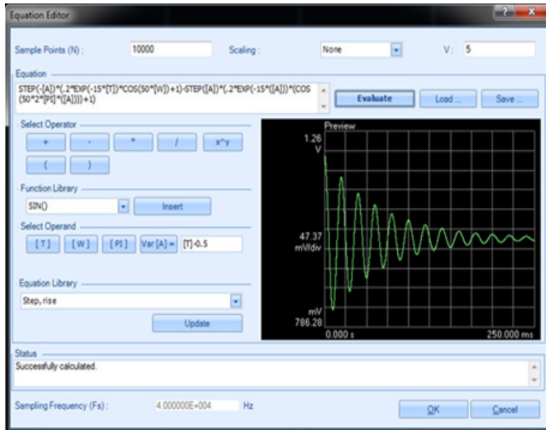
Figure 7. Waveform Builder's Equation editor
