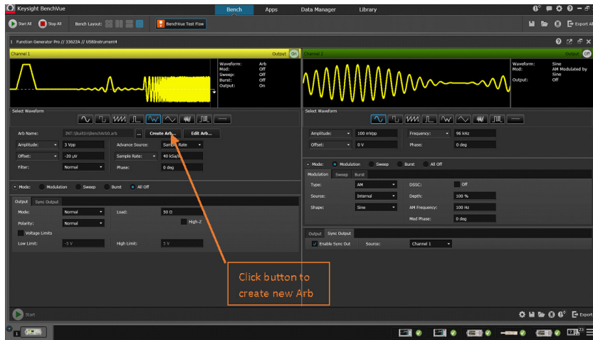
Figure 5. BenchVue's Function Generator application
