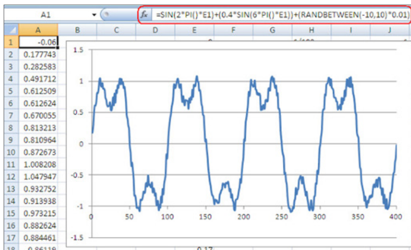
Figure 1. An arbitrary waveform in Excel
