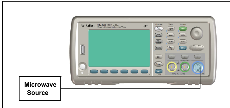
Figure 6-2. Microwave Source Connection to Channel 3
