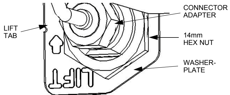
Figure 4-19. Connector-Adapter Parts
