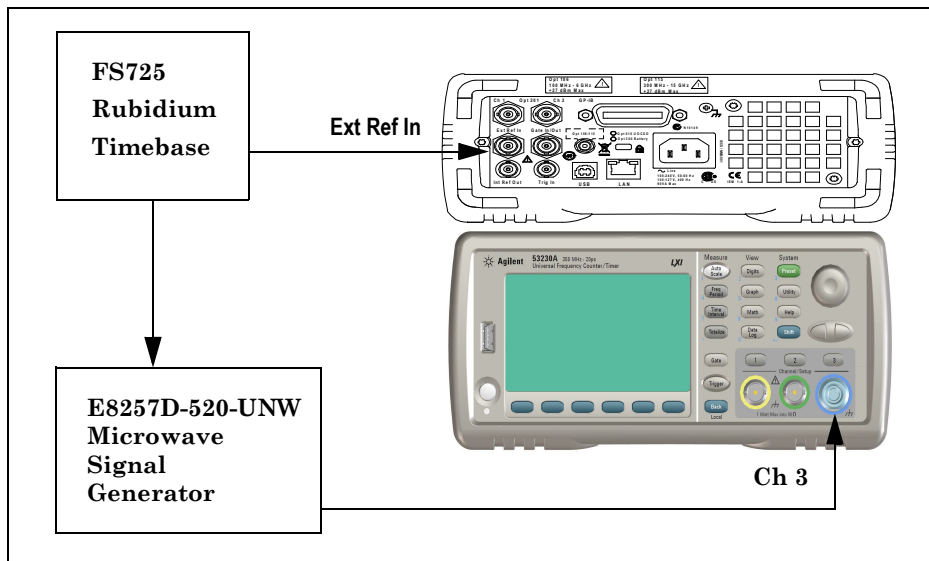
Figure 1-11. Option 115/150 Microwave Channel 3 Test Setup
