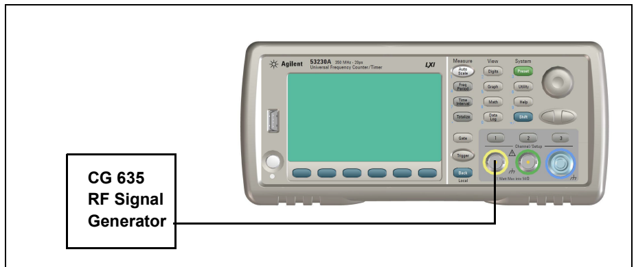
Figure 2-5. Oscillator Calibration Setup
